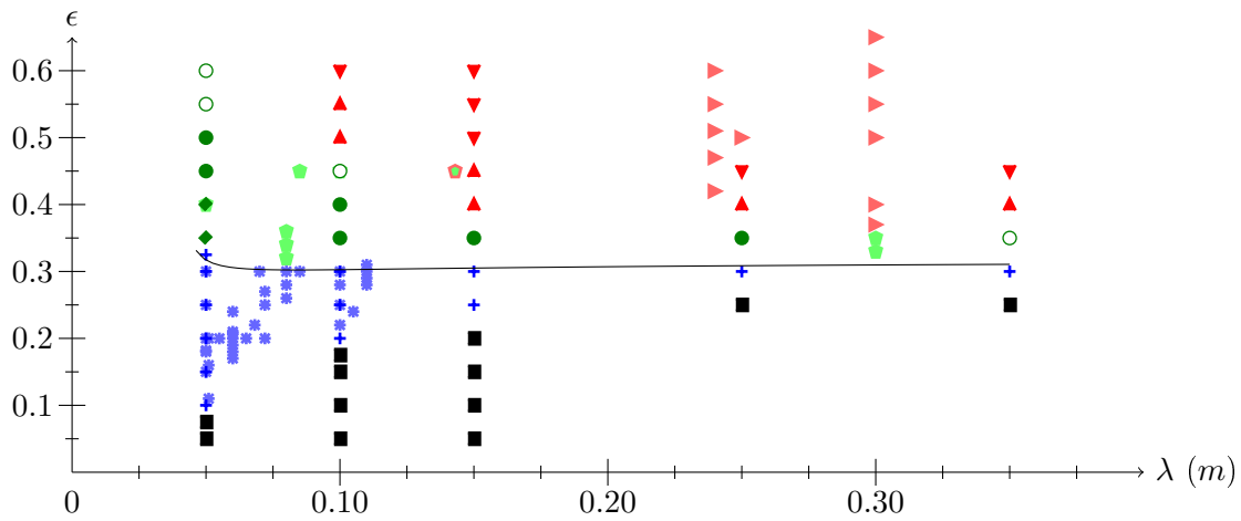
(c) \frac{d}{\lambda} = 0.5
