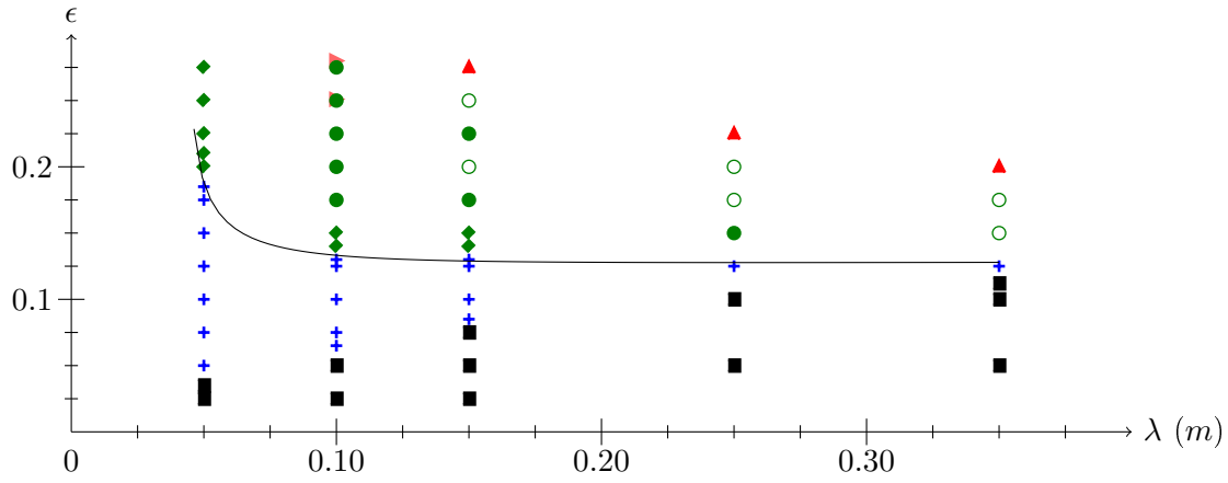
(a) \frac{d}{\lambda} = 0.1
