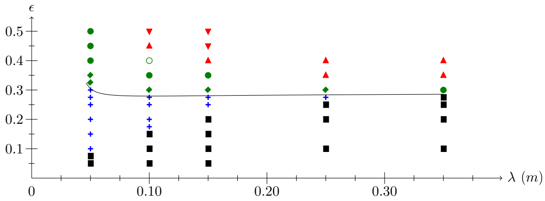
(b) \frac{d}{\lambda} = 0.3
