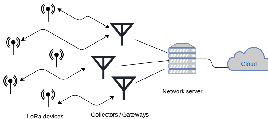
Figure 1.3: LoRa Network Topology
