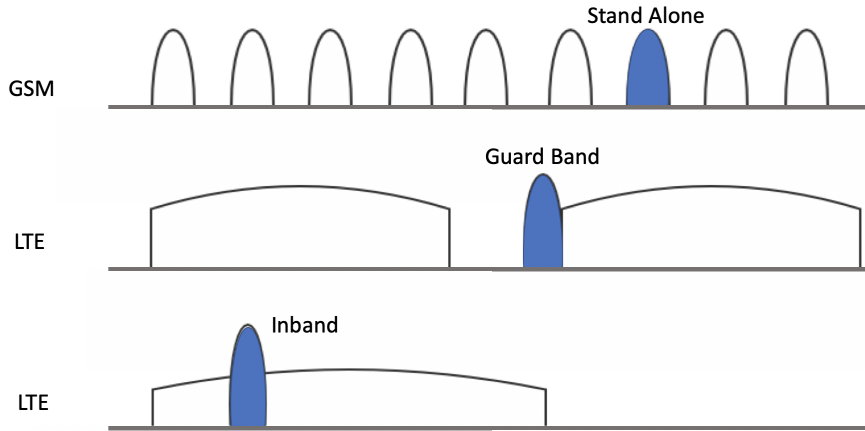
Figure 1.6: Three Different Deployment Modes of NB-IoT.
