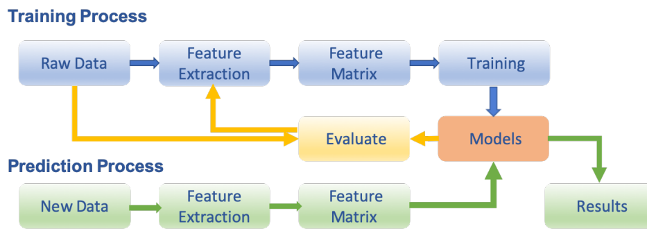
Figure 1.8: Supervised Learning Iterative Process
