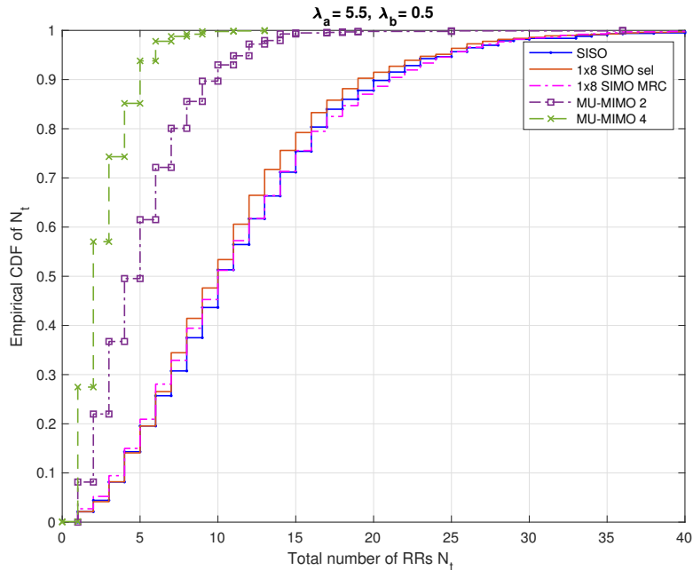
Figure 2.7: The empirical Cumulative Distribution Function (CDF) of N_t total number of RRUs required for the typical cell in which the maximal delay \tau_{max} = 1 ms, \lambda_a = 5.5 nodes/km 2 and \lambda_b = 0.5 nodes/km 2 .
