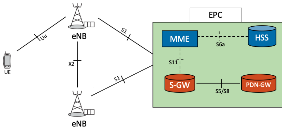
FIGURE 2.7: Architecture LTE.
