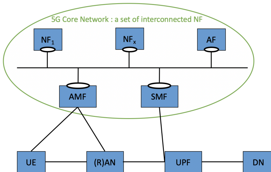
FIGURE 2.10: Architecture générale 5G
