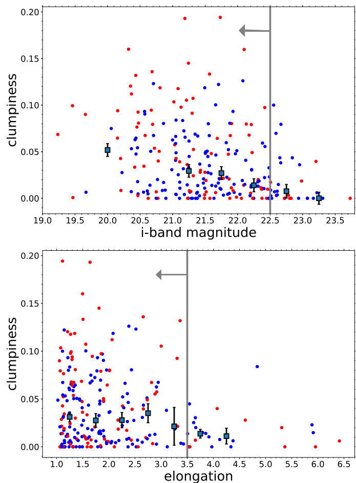
Fig. A.1. Top: Clumpiness vs i-band total magnitude ( i_{\text{mag}} ) for our initial sample of 145 main sequence and 96 starburst galaxies (in blue and red, respectively). Median clumpiness values and errors (gray squares with black error bars) are derived for 6 bins of i_{\text{mag}} . Our selection cut ( i_{\text{mag}} < 22.5 ) is highlighted with a vertical gray line. Bottom: Clumpiness vs elongation for the same sample as above, with median clumpiness and errors estimated in 7 bins of elongation. The vertical gray line indicates our cut for the final selection (elongation < 3.5 ), even though we remember that one additional nearly edge-on MS galaxy was also removed by visual inspection.
