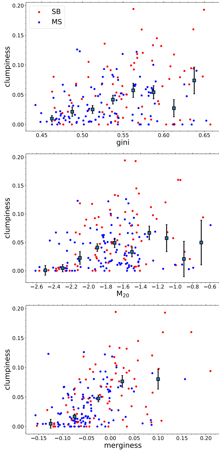
Figure 5.7: The three diagrams compare the clumpiness of our final galaxy sample to the Gini and M_{20} coefficients (first and second panels, respectively), and to the merginess parameter, defined in Eq. 5.3. Starbursts are shown in red, while main sequence galaxies are color coded in blue. The median clumpiness (and errors) computed in bins of Gini, M_{20} and merginess are represented with gray squares and black error bars.
