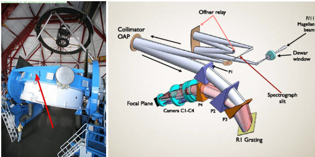
Figure 2.1: Left : View of the Magellan Baade telescope, where the arrow indicates the position of FIRE. Right : Optical layout of FIRE, showing 1:1 pre-slit Offner relay, reflecting collimator, cross-dispersing prism array, reflective diffraction grating, and four-element camera. (R. Bernstein)
