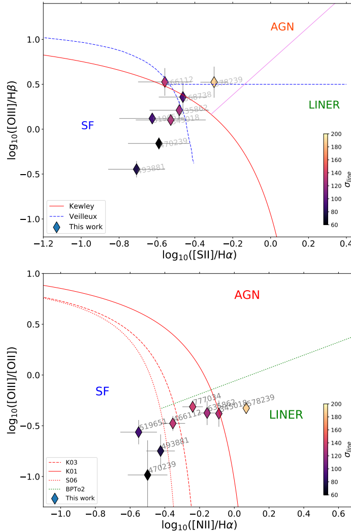
Figure 4.14: Diagram of [\text{OIII}]/\text{H}\beta compared to [\text{SII}]6717+6731/\text{H}\alpha (Top) and [\text{OIII}]5007/[\text{OII}]3727+3729 vs. [\text{NII}]6583/\text{H}\alpha (bottom) for 8 galaxies of the Magellan sample with optical spectra available and contemporary detection of [\text{OIII}] and one between [\text{SII}]+\text{H}\beta or [\text{OII}] . The two diagrams are also called the S2 and the O2 BPT diagrams, respectively. As in the classical BPT diagram in Fig. 4.5, they show that starbursts have different line excitation properties, and those with higher line velocity widths are generally shifted towards the AGN/LINER regions, according to empirical separation lines derived in the local ( z \lesssim 0.3 ) Universe.
