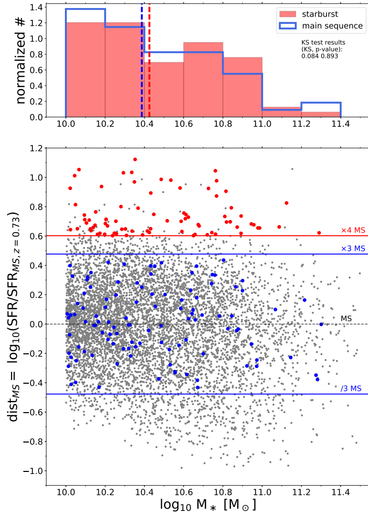
Figure 5.5: Bottom : Diagram showing for my parent sample of star-forming galaxies in COSMOS ( 0.5 < z < 0.9 ) their distance from the main sequence as a function of stellar mass. I highlight with a black horizontal line the 0 level. The blue and red lines indicate the limits taken for the main sequence and starburst selection, respectively. The final selected sample is highlighted with blue and red points, correspondingly. The SFR used in the y -axis is normalized to the median redshift of my sample (0.73), following the SFR-redshift evolution of Sargent et al. (2014). Top : Histogram distribution (normalized to unit area) of the stellar masses of my selected sample of starbursts (red) and main sequence galaxies (blue), showing that the two subsets have similar distributions. The two vertical lines indicate, according to their corresponding colors, the median values of M_* of SB and MS galaxies.
