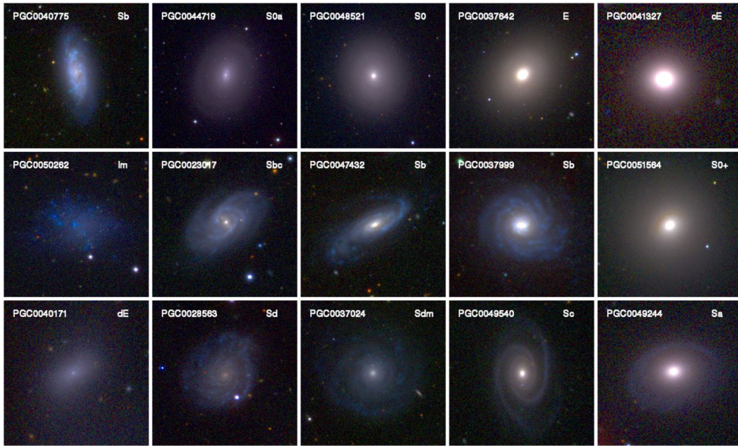
Figure 1.2: irg colour images of nearby galaxies with different morphological classes (cf. Table 1.1) and different Bulge/Disk luminosity ratios (increasing toward the right), from the FIGI catalog (“Extraction de Formes Idéalisées de Galaxies en Imagerie”) of Baillard et al. (2011).
