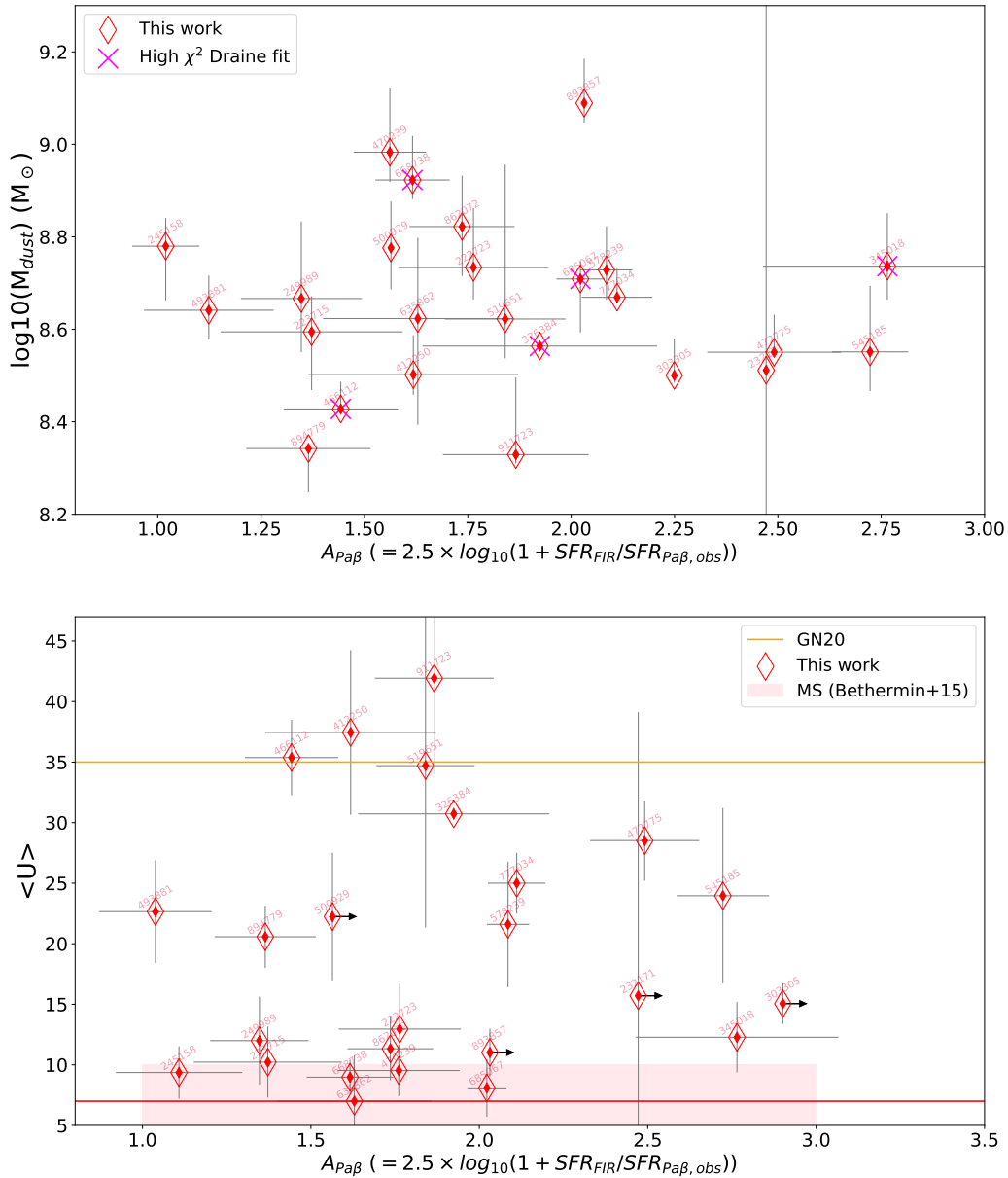
Figure 7.4: Top : Diagram comparing the dust mass to the attenuation at Pa\beta ( A_{Pa\beta,IRX} ) for the 25 starbursts observed with Magellan FIRE; Bottom : Comparison between the attenuation and the average radiation field \langle U \rangle for the same sample.
