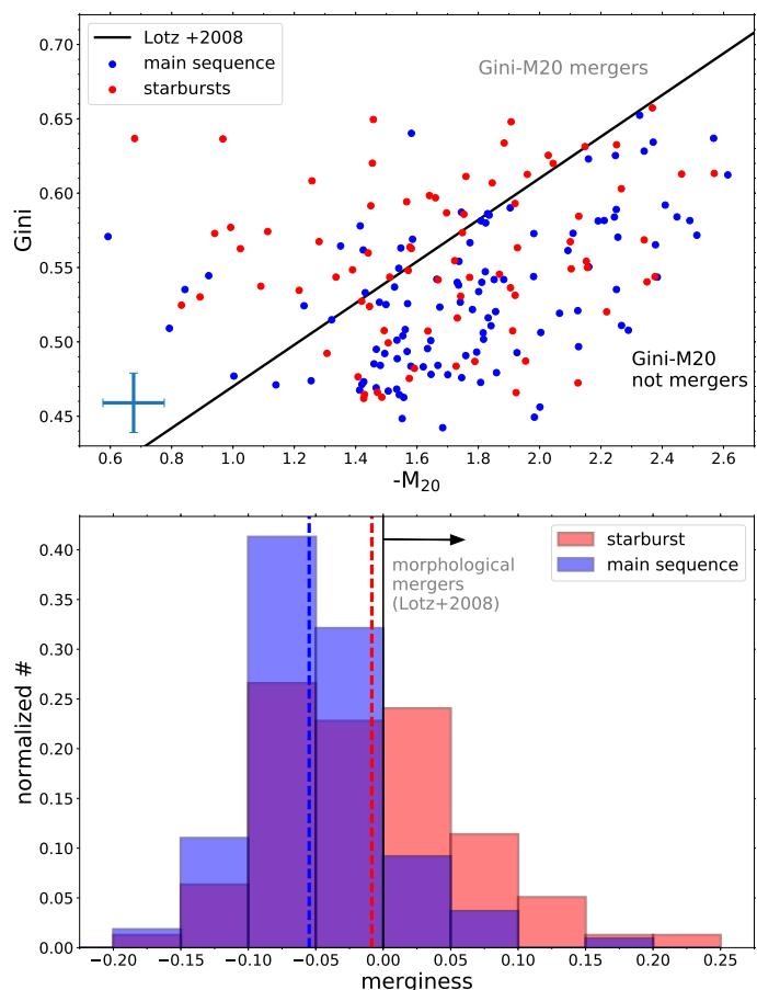
Fig. 3. Top: Gini- M_{20} diagram for the final sample of starburst and main sequence galaxies analyzed in this work (in red and blue, respectively). Galaxies above the black continuous line are morphological mergers, according to Lotz et al. (2008). The typical uncertainties of Gini and M_{20} are shown by the representative error bars in the lower left corner. Bottom: Histogram distribution (for SBs and MS) of the merginess parameter, defined as the difference between the measured Gini coefficient and that required to classify the galaxy as a morphological merger. It shows that the majority of galaxies classified as mergers according to this criterion are also starbursts.
