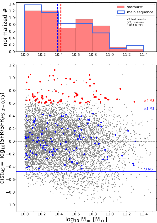
Fig. 5. Bottom: Diagram showing for our parent sample of star-forming galaxies in COSMOS ( 0.5 < z < 0.9 ) their distance from the main sequence as a function of stellar mass. We highlight with a black horizontal line the 0 level. The blue and red lines indicate the limits taken for our main sequence and starburst selection, respectively. The final selected sample is highlighted with blue and red points, correspondingly. The SFR used in the y-axis is normalized to the median redshift of our sample (0.73), following the SFR-redshift evolution of Sargent et al. (2014). Top: Histogram distribution (normalized to unit area) of the stellar masses of our selected sample of starbursts (red) and main sequence galaxies (blue), showing that the two subsets have similar distributions. The two vertical lines indicate, according to their corresponding colors, the median values of M_* of SB and MS galaxies.
