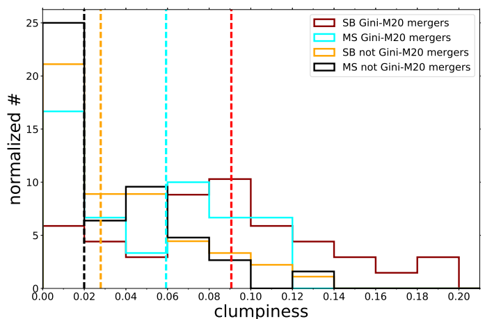
Fig. 8. Normalized distribution (continuous line) and medians (vertical dashed lines) of the clumpiness for four types of galaxies: main sequence galaxies with \text{merginess} < 0 and > 0 (in black and cyan, respectively), and starbursts (in orange those with \text{merginess} < 0 and in red the morphological merger subset). We notice that the merger-selected starbursts dominate the high clumpiness tail, while the remaining SBs are basically indistinguishable from the population of main sequence galaxies with \text{merginess} < 0 . A substantial contribution to the high clumpiness population also comes from mergers inside the MS, as shown by the cyan excess at 0.06 < c < 0.12 . A Kolmogorov-Smirnov (KS) test between merger and not-merger MS systems (cyan and black subsets) yields 0.302 (p-value = 0.094).
