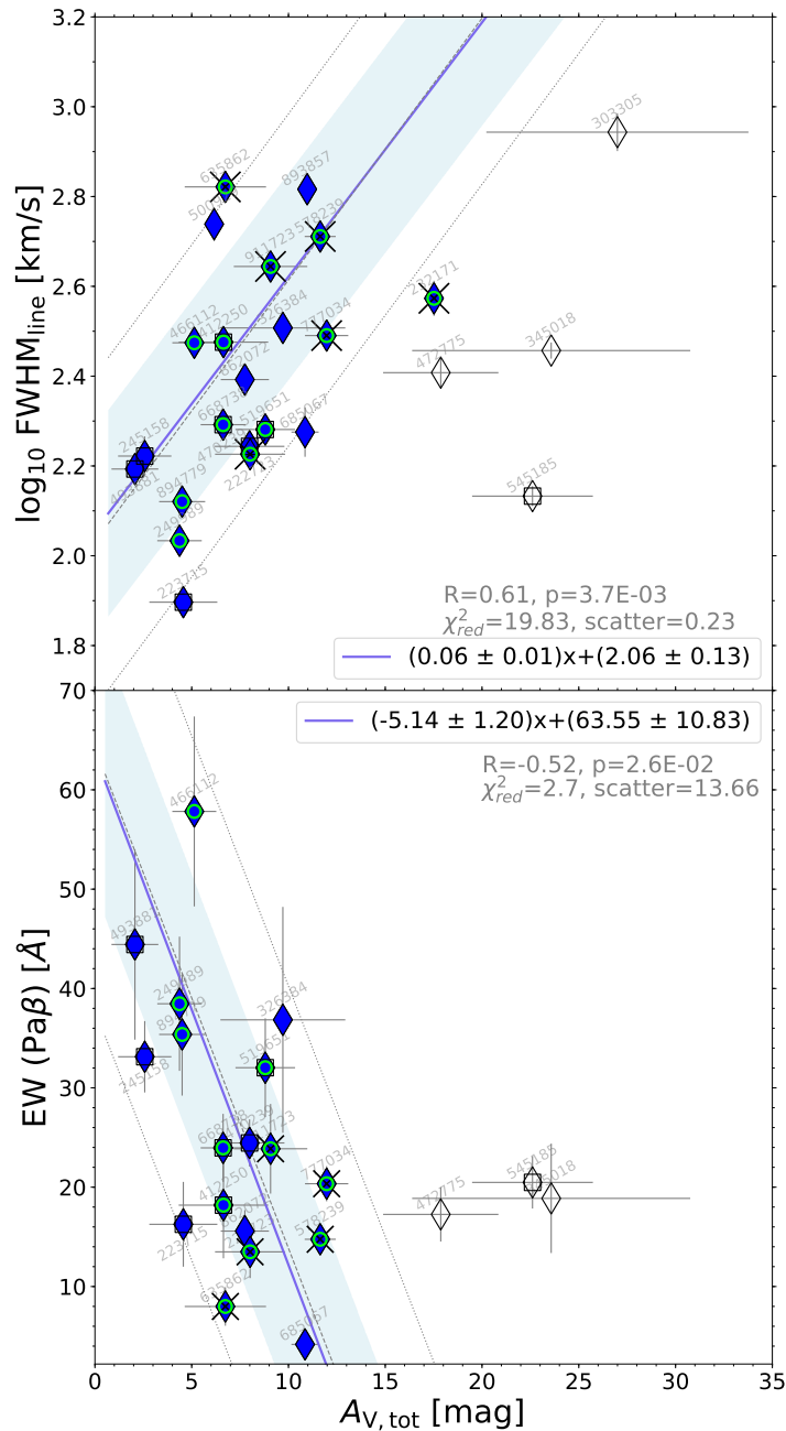
Figure 4.2: Correlations of A_{V,tot} with the line velocity width (top), and with the \text{EW}(\text{Pa}\beta) (bottom). In the last diagram, 4 galaxies without \text{EW}(\text{Pa}\beta) measurements are not considered. The details are the same as Fig. 4.1.
