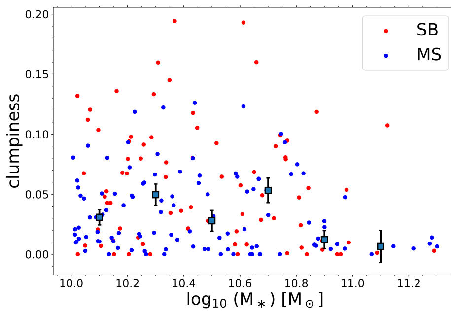
Figure 5.9: Stellar mass vs clumpiness for our final sample of MS and SB galaxies (in blue and red, respectively), with median clumpiness (and error) in 6 M_* bins superimposed with gray squares.
