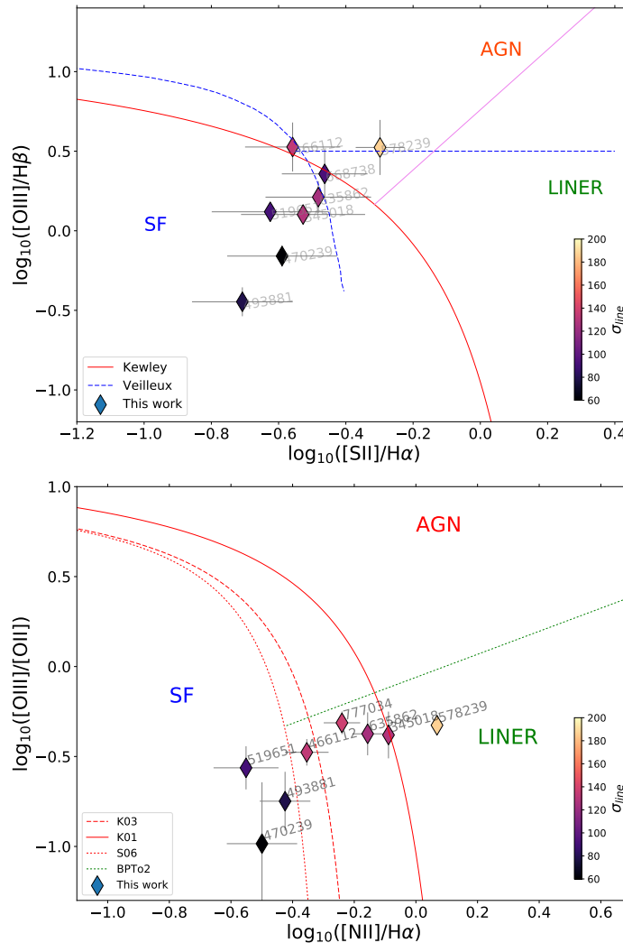
Figure 4.14: Diagram of [\text{OIII}]/\text{H}\beta compared to [\text{SII}]6717+6731/\text{H}\alpha ( Top ) and [\text{OIII}]5007/[\text{OII}]3727+3729 vs. [\text{NII}]6583/\text{H}\alpha ( bottom ) for 8 galaxies of the Magellan sample with optical spectra available and contemporary detection of [\text{OIII}] and one between [\text{SII}]+\text{H}\beta or [\text{OII}] . The two diagrams are also called the S2 and the O2 BPT diagrams, respectively. As in the classical BPT diagram in Fig. 4.5, they show that starbursts have different line excitation properties, and those with higher line velocity widths are generally shifted towards the AGN/LINER regions, according to empirical separation lines derived in the local ( z \lesssim 0.3 ) Universe.
