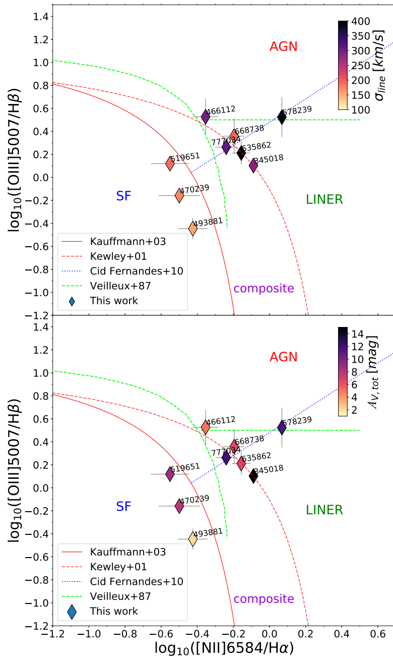
Figure 4.5: Top : BPT diagram of nine starbursts in my sample with optical spectra available (for one galaxy included in zCOSMOS, we did not detect both [\text{OIII}]\text{5007} and \text{H}\beta ). While three sources lie in the SF excitation region, the remaining galaxies are not consistent with SF, and their spectra show a mixture of composite, AGN and LINER properties. The color coding indicates that galaxies with higher N2 which are closer to the AGN and LINER regions also have increasingly higher line velocity widths ( \sigma_{\text{line}} ). Bottom : Same diagram as above, but here the galaxies are color coded according to their total dust attenuation A_{V,\text{tot}} . More obscured starbursts preferentially display AGN or LINER properties.
