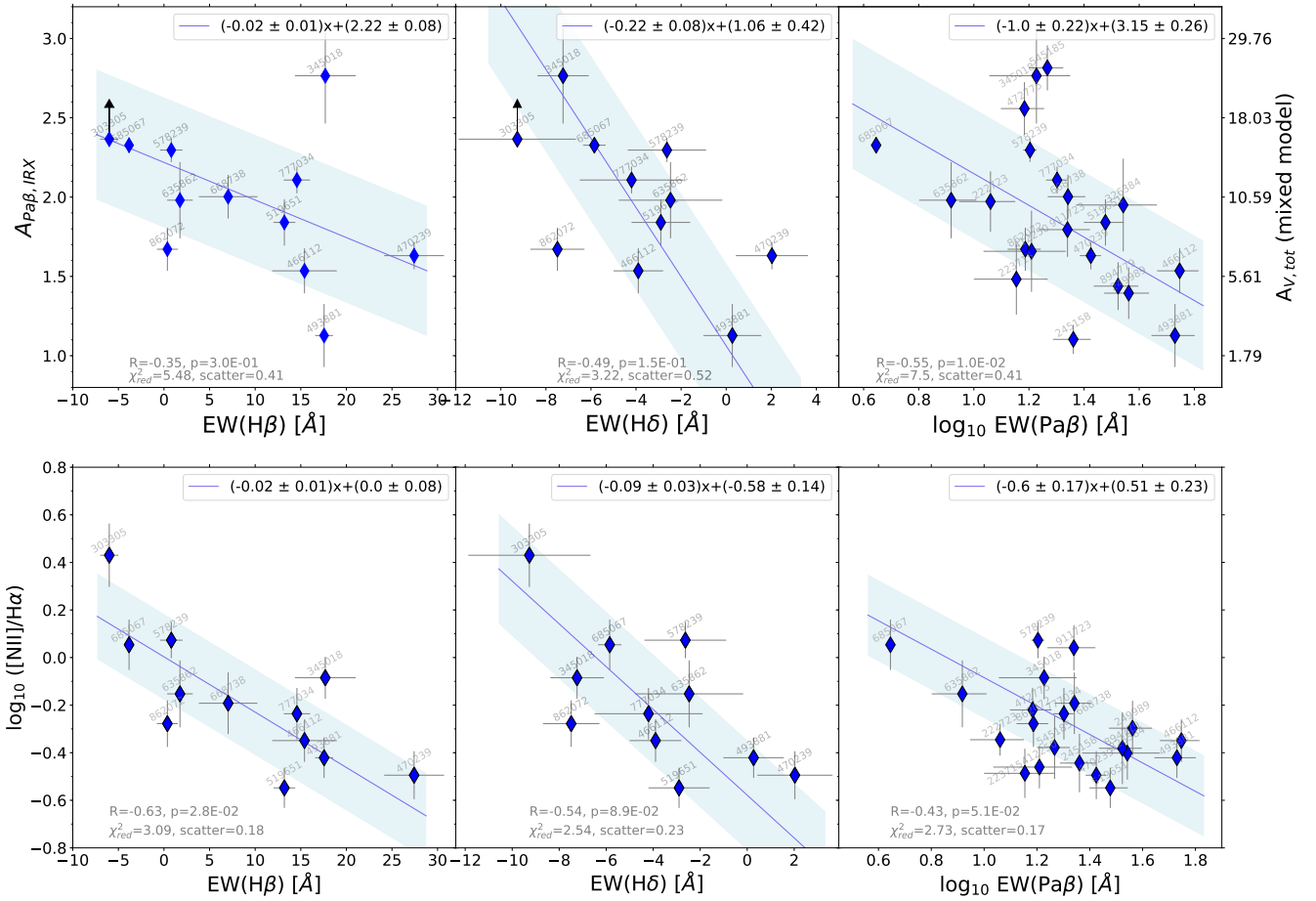
Fig. 8. Top panels: comparison between the EW of H\delta , H\beta and Pa\beta lines to the dust attenuation parameter A_{Pa\beta,IRX} , defined as 2.5 \times \log_{10}(1 + SFR_{IR}/SFR_{Pa\beta,obs}) (Paper I). We remark that the last panel is equivalent to the bottom-right plot in Fig. 3, even though a different scale has been used (the relation between A_{Pa\beta,IRX} and A_{V,tot} is given in Eq. (1)). Bottom panels: correlations between the EW of H\delta , H\beta , Pa\beta lines and the N2 index ( = \log_{10}([NII]/H\alpha) ). The blue continuous lines are the best-fit linear relations, determined as explained in Sect. 3, while the blue shaded area show the \pm 1\sigma scatter of our data around the best-fit relations.
