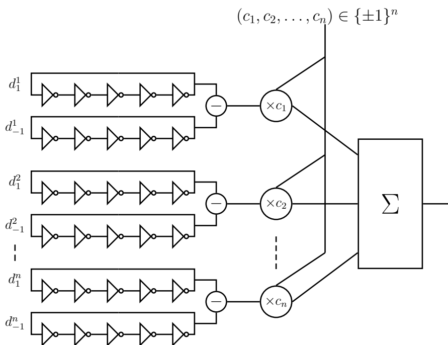
Figure 4.4: RO-sum PUF
