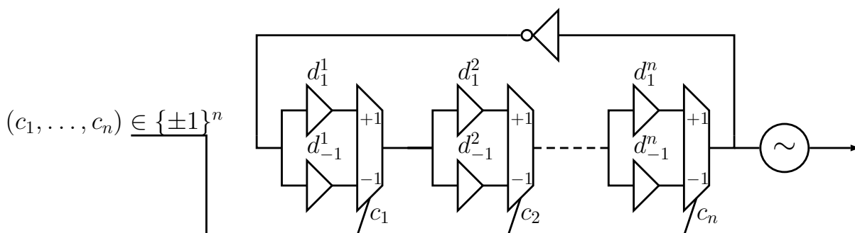
Figure 4.5: Loop PUF
