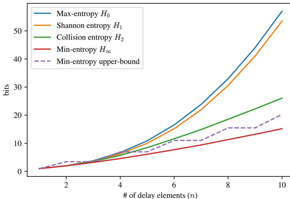
Figure 6.2: Entropy estimates for n \leq 10 . The upper bound of the min-entropy (dashed line) is taken from [1].
