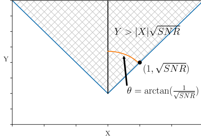
Figure 5.2: Polar representation of X and Y .
