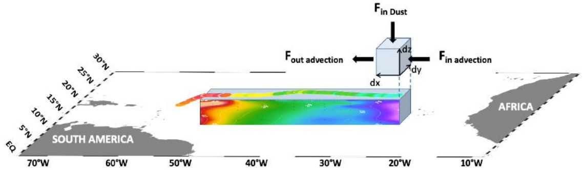
Figure 5. Schematic representation of how modelled advection, and dust deposition fluxes have been applied to the upper 100 m dissolved aluminum (dAl) data for GApr08. Input/output fluxes are designated by black arrows. The GApr08 upper 100 m dAl section as well as the towed fish dAl data are displayed on the map.
