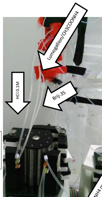
Mixing coil for LUM/reaction buffer & HCl 0.1M post-elution
