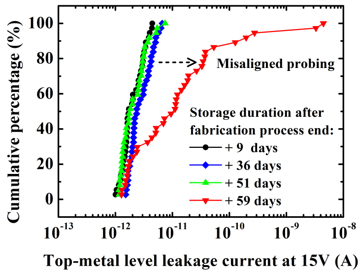
Figure 3.13: Cumulative leakage currents measured at 15V on 50 μm-wide pads.
