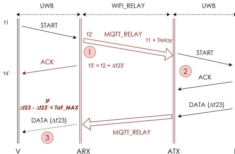
Fig. 28. Selective SAA with relay
