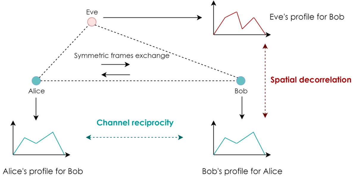
Fig. 52. Principles of Channel-based Key Extraction
