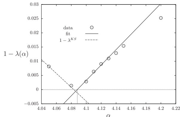
Figure 8.5: The stability parameter \lambda(\alpha) in the case of a continuous transition (here for k = 4 , \omega_0 = \omega_k = 0 , \omega_1 = \dots = \omega_{k-1} = 1 ). From the fit one obtains the result \alpha = 4.088 , which is in good agreement with the analytical one \alpha_{KS} = 4.083 .
