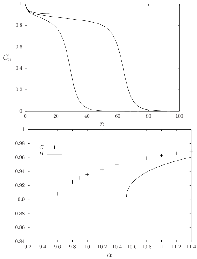
Figure 9.2: Top: the correlation function C_n(\alpha, k) as a function of n for k = 5 and from left to right \alpha = 9.2, \alpha = 9.4, \alpha = 9.6 . Bottom: the large n limit C(\alpha, k) = \lim_n C_n(\alpha, k) as a function of \alpha for k = 5 , along with the contribution of the hard fields H(\alpha, k) = \lim_n H_n(\alpha, k) discussed in Sec. 7.4. The first curve is non zero for \alpha \geq \alpha_d(k = 5) \approx 9.465 , the second one for \alpha \geq \alpha_r(k = 5) \approx 10.526 .
