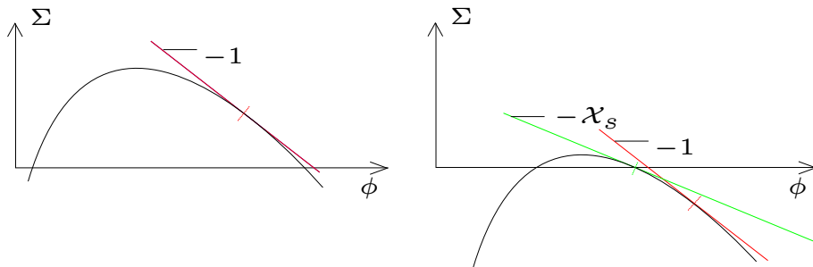
Figure 2.2: Left: uncondensed regime the supremum of (2.20) is achieved for \phi^* such that \Sigma(\phi^*) > 0 and (d\Sigma(\phi)/d\phi) = -1 (the red tangent has slope -1 ). Right: condensed regime, the supremum of (2.20) is achieved for \phi^* such that \Sigma(\phi^*) = 0 and (d\Sigma(\phi)/d\phi) = -\mathcal{X}_s (green tangent), the value of \phi such that (d\Sigma(\phi)/d\phi) = -1 has a negative complexity.
