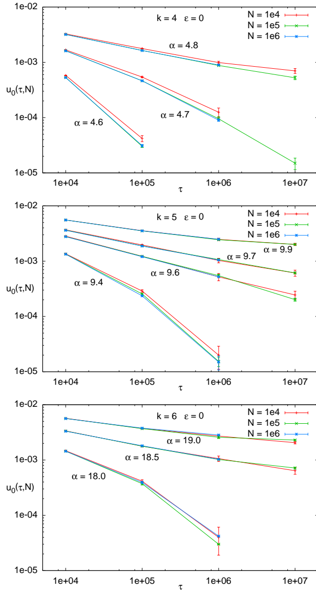
Figure 8.11: Plotting the lowest intensive energy reached by SA with no bias ( \epsilon = 0 ) as a function of \tau provides a better way to estimate the algorithmic threshold \alpha_{alg} : the decay is faster (resp. slower) than a power law if \alpha < \alpha_{alg} (resp. \alpha > \alpha_{alg} ).
