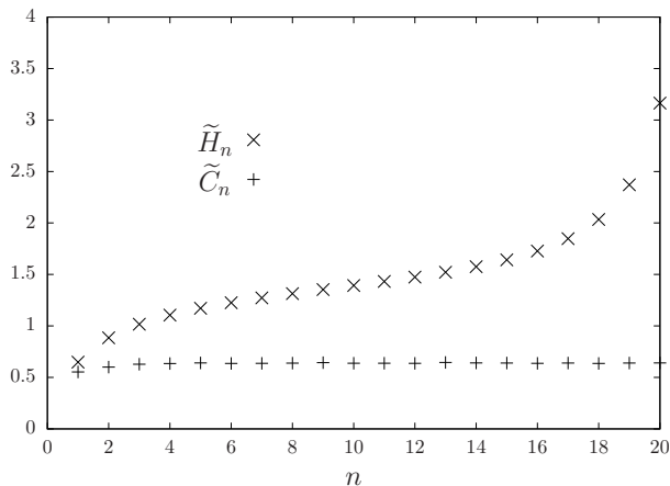
Figure 10.4: The reduced correlation function \tilde{C}_n and its hard-field contribution \tilde{H}_n as a function of the distance n for b = 0.4 , \tilde{\epsilon} = 0 and \gamma = 1.35 , slightly below the rigidity threshold.
