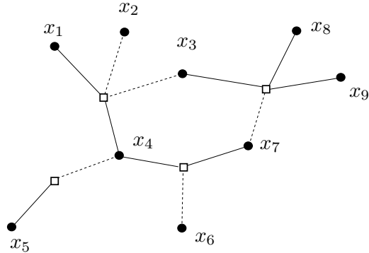
Figure 1.1: graphical representation of the SAT formula F = (x_1 \vee \overline{x_2} \vee \overline{x_3} \vee x_4) \wedge (\overline{x_4} \vee x_5) \wedge (x_4 \vee \overline{x_6} \vee x_7) \wedge (x_3 \vee \overline{x_7} \vee x_8 \vee x_9)
