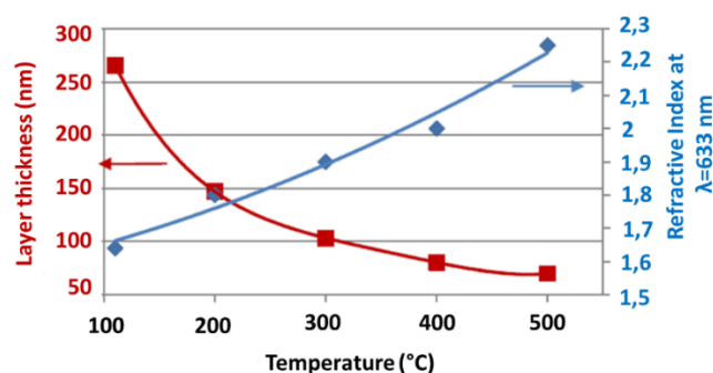
Figure 2.13: Interaction of layer thickness with refractive index and annealing temperature for a TiO 2 xerogel layer [30].
