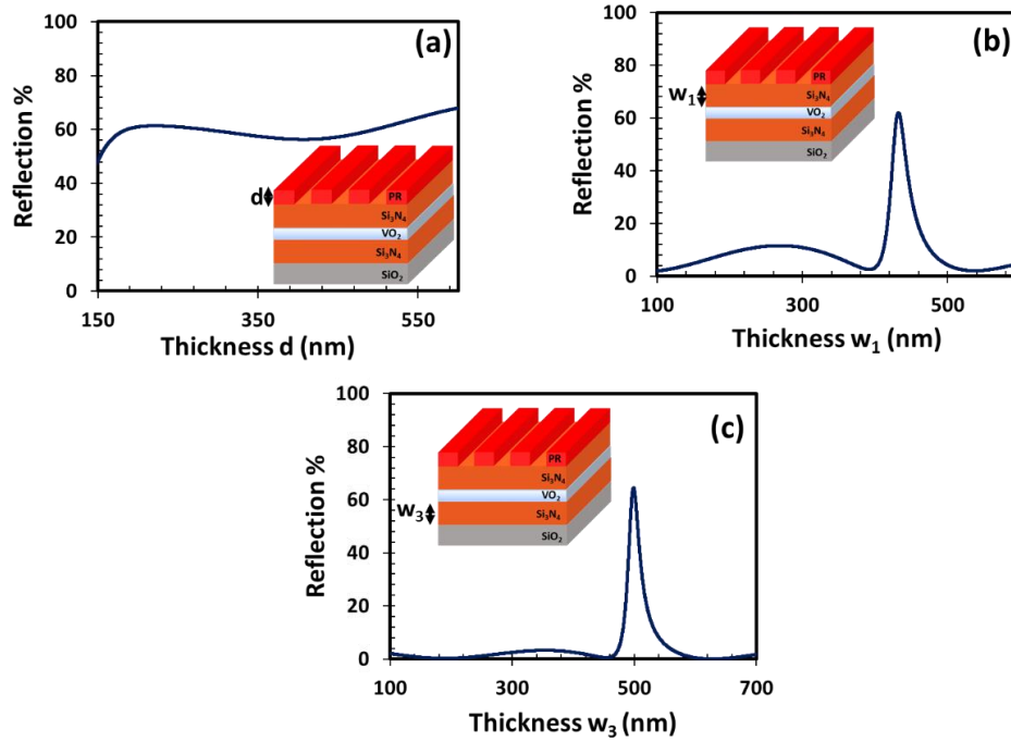
Figure 5.15: 1D scan for layer thickness determination of resist d ( w_1 = 440 nm and w_3 = 500 nm) (a), Si 3 N 4 thickness w_1 ( d = 200 nm and w_3 = 500 nm) (b) and Si 3 N 4 thickness w_3 ( w_1 = 440 nm and d = 200 nm) (c) for \lambda = 1500 nm, \Lambda = 950 nm, duty cycle 0.5 and w_2 = 80 nm.
