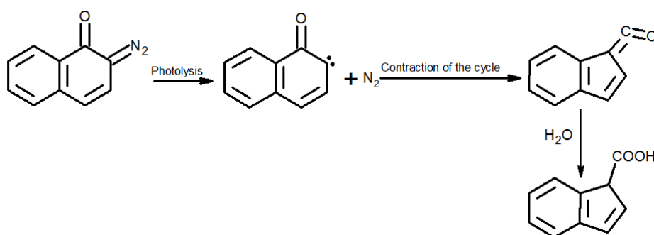
Figure 2.7: Conversion of the photoinitiator molecule (DNQ) into an indene carboxylic acid allowing the dissolubility to solubility transformation in the developer.
