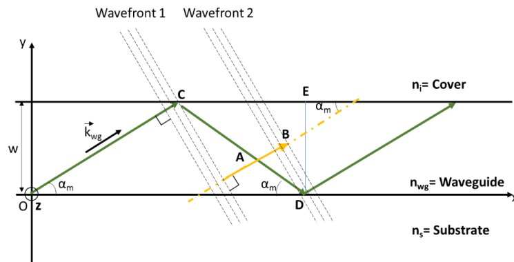
Figure 1.23: Representation of light propagation in a planar waveguide.
