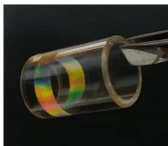
Figure 1: Micro patterned grating on a \text{TiO}_2 sol gel-made waveguide layer in the hollow of a fused silica tube.
