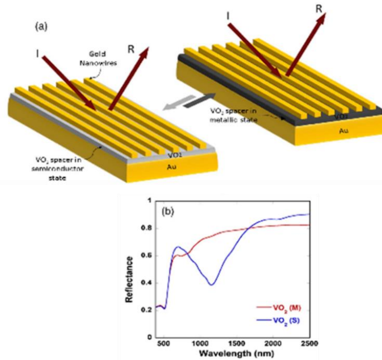
Figure 5.7: Simulated reflectance variation between metallic and semiconductor state for the proposed Au/VO 2 /Au grating structure.
