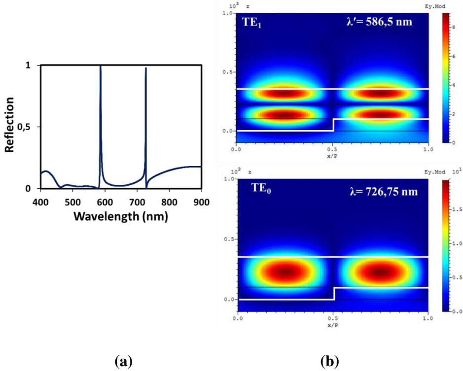
Figure 1.31: The left resonant wavelength peak corresponds to \lambda' = 586.5 nm and the right to \lambda = 726.75 nm exciting the TE 1 and TE 0 mode respectively (a), 2D electric field amplitude distributions on \lambda' and \lambda respectively scanned for a single period (b). The tested structure consists of a TiO 2 waveguide of w = 250 nm and a subwavelength binary resist grating of d = 100 nm, \Lambda = 340 nm and DC = 0.5.
