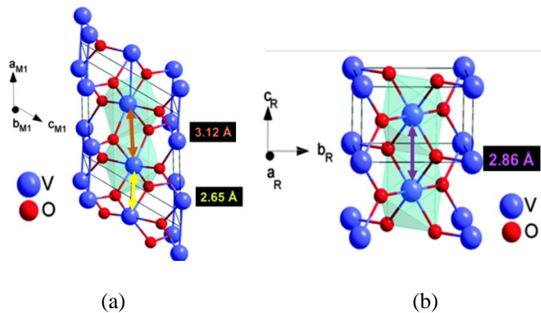
Figure 4.1: Crystal structure of VO 2 at T < 68 \text{ }^\circ\text{C} in the monoclinic phase (a) and T > 68 \text{ }^\circ\text{C} in the rutile-tetragonal phase (b) [5]
