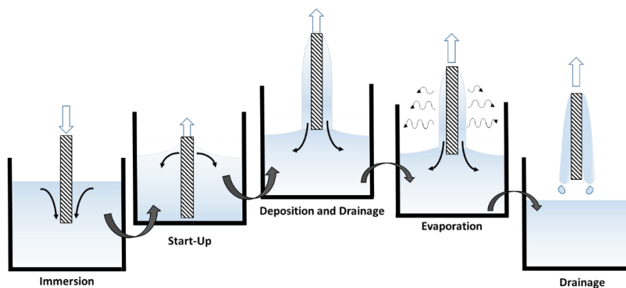
Figure 2.21: Principle steps of the dip coating process.
