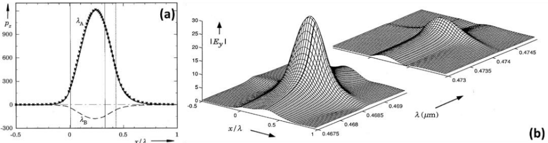
Figure 1.5: Power flux p_z (a) and transverse field amplitude (b) variation for a dielectric grating [23].
