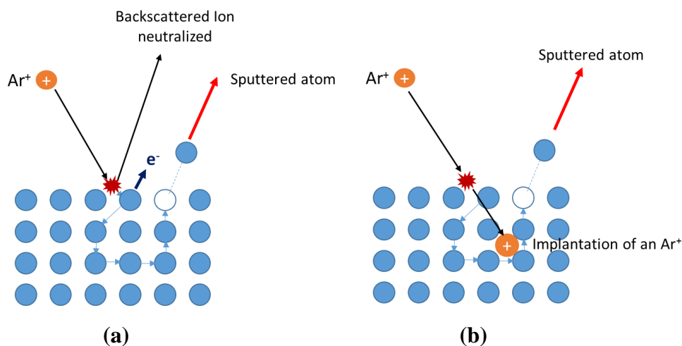
Figure 4.24: Low energy knock-on \text{Ar}^+ sputtering (a) and high-energy knock-on sputtering with ion implantation (b) and ejection of target atom by cascade collisions.
