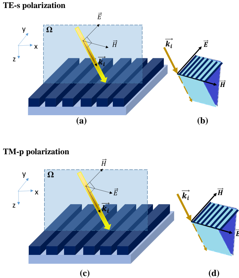
Figure 1.21: Polarization of incident light in relation to grating lines. TE (a) and TM polarization (c) of the incident \vec{k}_i light and representation of the vectors forming a trihedral (b), (d) respectively.
