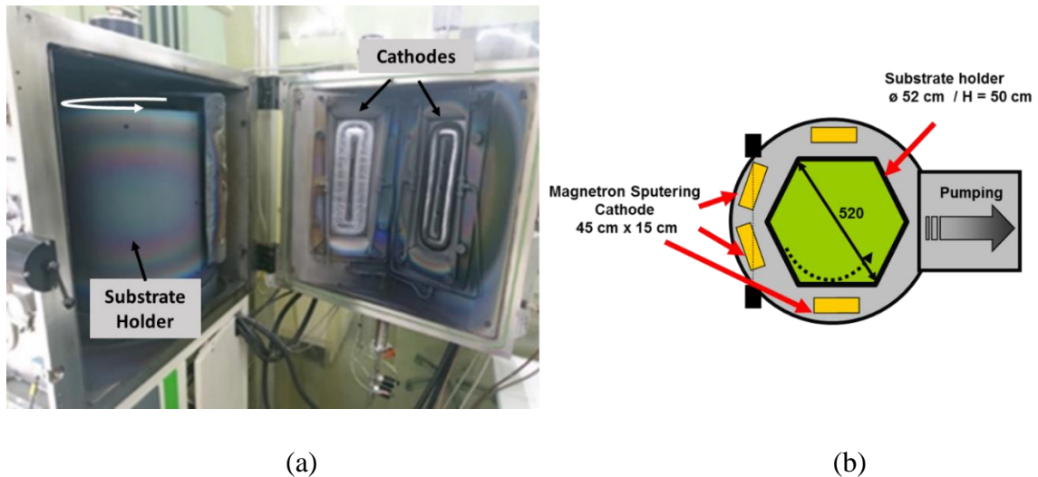
Figure 4.25: Image (a) and schematic (top view) (b) of the magnetron reactor.
