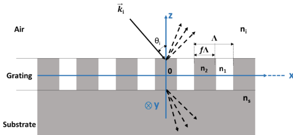
Figure 1.42: Schematic representation of the modal problem in a binary rectangular grating.
