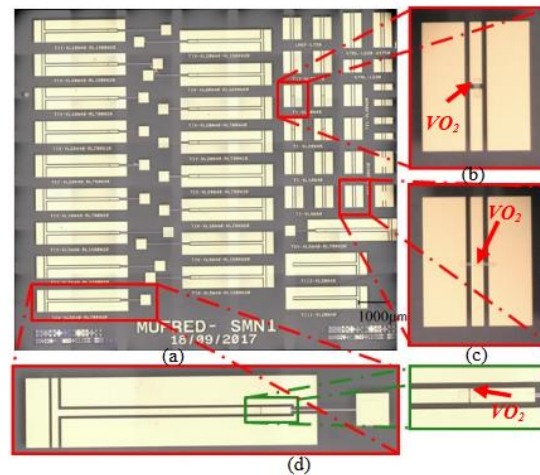
Figure 4.11: RF switches in series made with VO 2 based elements [23].
