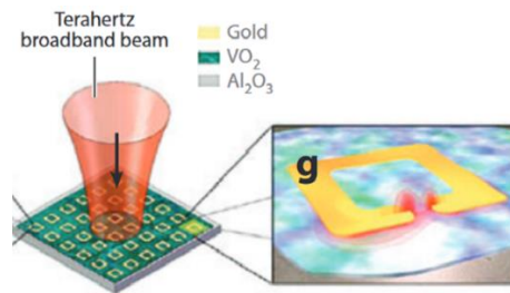
Figure 4.8: Experimental set-up and close up of the Split Ring Resonator lying on a sapphire substrate coated with VO 2 thin film [19].
