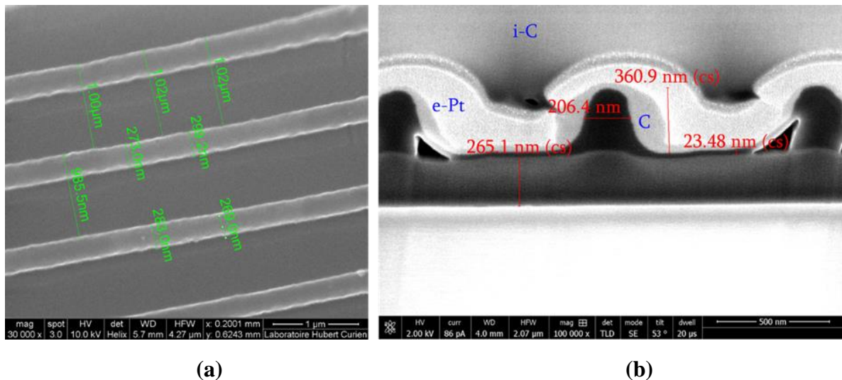
Figure 3.14: SEM top view (a) and FIB cross section images (b) of the waveguide grating assisted by carbon ex-situ (i-C) for metallization, e-Pt for protection and a final ionic deposition with C precursor for surface sputtering and cross-section.
