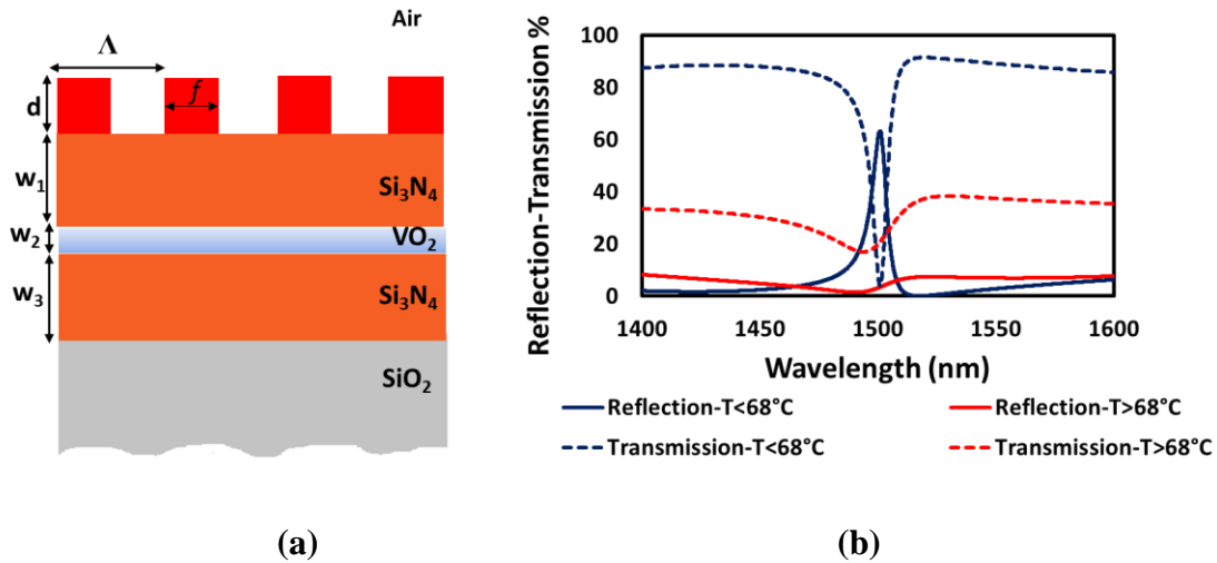
Figure 5.16: Final structure for a resonance at \lambda = 1500 nm under normal incidence and TE polarization; d = 225 nm, w_1 = 435 nm, w_2 = 80 nm, w_3 = 502 nm, \Lambda = 950 nm and f = 475 nm (a), Simulated reflection and transmission amplitude of the structure when VO 2 layer is in dielectric or/and metallic phase (b).
