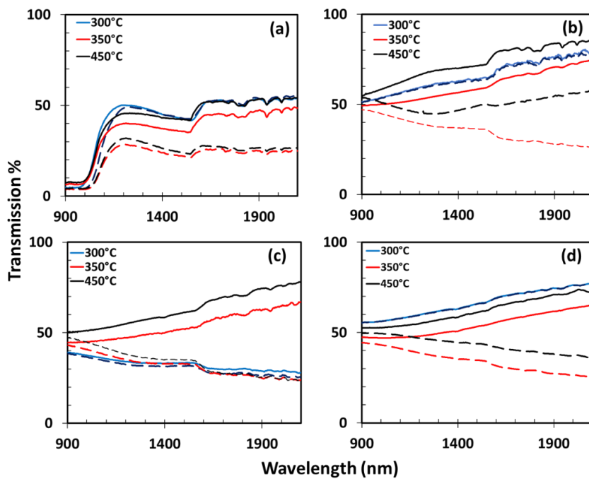
Figure 4.18: Optical transmittance spectra in the spectral range 900 nm-2000 nm recorded at two different temperature: ambient temperature (plain line) and 100 °C (dashed line) of VO x annealed at different temperatures on various substrates: Si (a), Quartz (b), SiO 2 (c), SiO 2 -TiO 2 (d).
