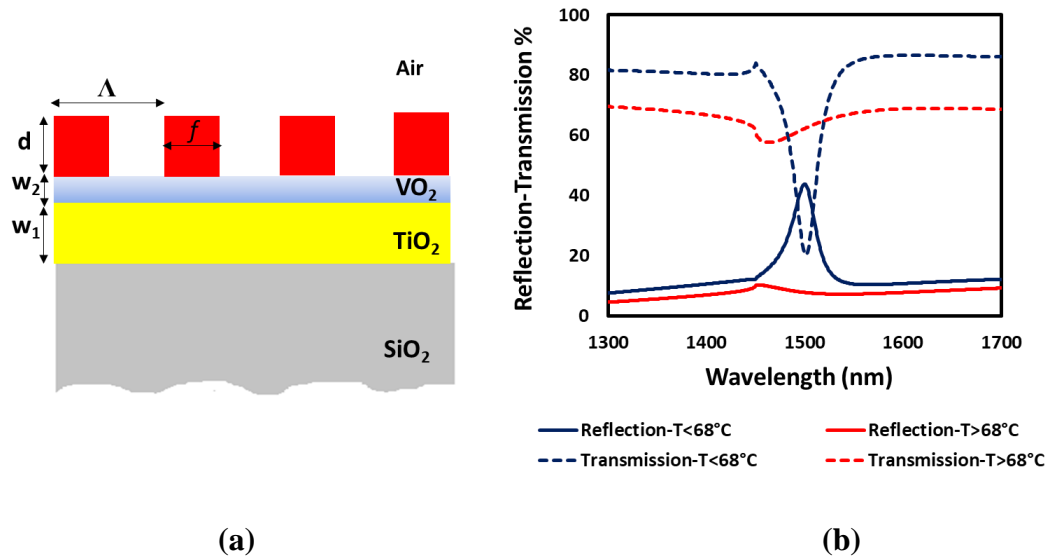
Figure 5.24: Final structure for a resonance at \lambda = 1500 nm under normal incidence and TE polarization; d = 216 nm, w_2 = 27 nm, w_1 = 75 nm, \Lambda = 1000 nm and f = 440 nm (a), Simulated reflection and transmission amplitudes of the structure when VO 2 is in dielectric or metallic phase (b).
