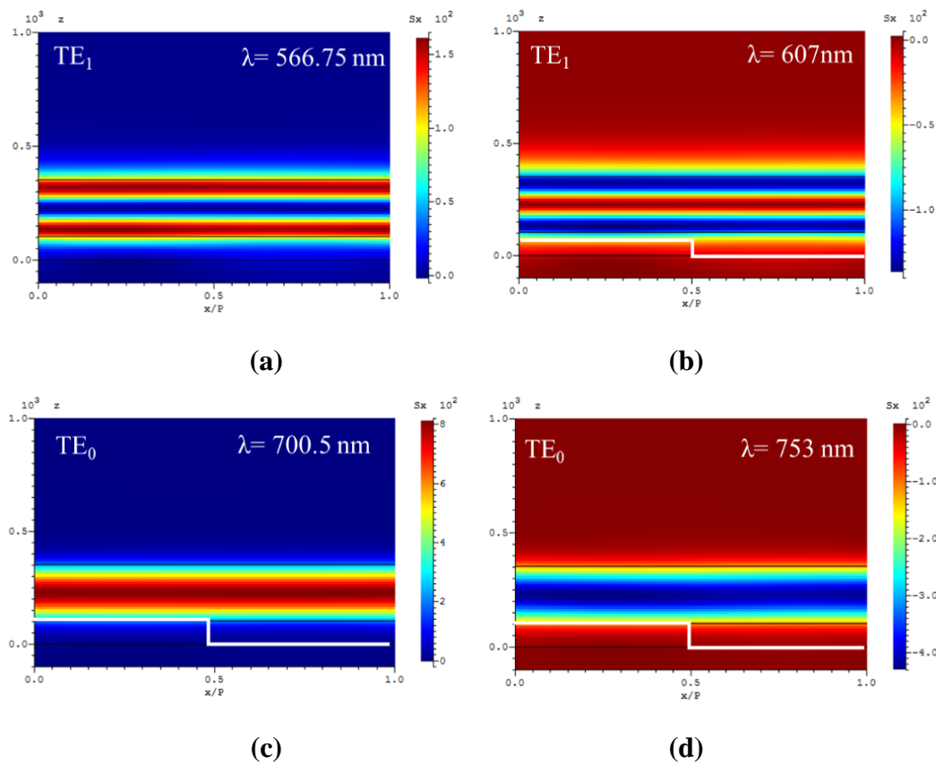
Figure 1.37: Power flow distribution along x-axis exhibiting the TE 1 and TE 0 forward (a), (c) and backward mode (b), (d) respectively.
