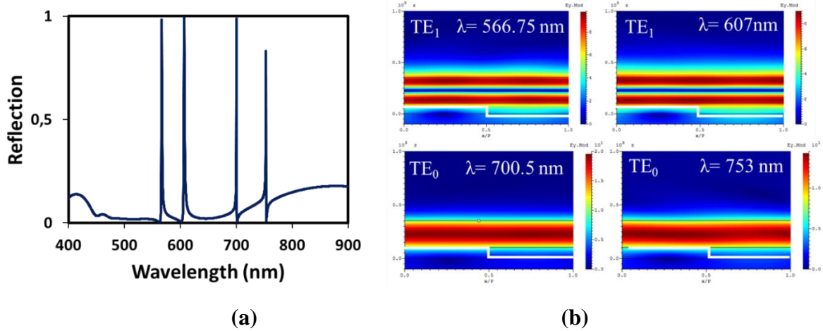
Figure 1.36: Bimodal waveguide with excitation mode resonances that correspond to \lambda_{TE1}=566.75 nm, \lambda_{TE1}=607 nm, \lambda_{TE0}=700.5 nm and \lambda_{TE0}=753 nm (a) with the corresponding fields amplitude starting from top left (b). The structure consists of d = 102 nm PR, w = 250 nm waveguide, \Lambda = 340 nm period, DC = 0.5 and \theta_1 = 5^\circ .
