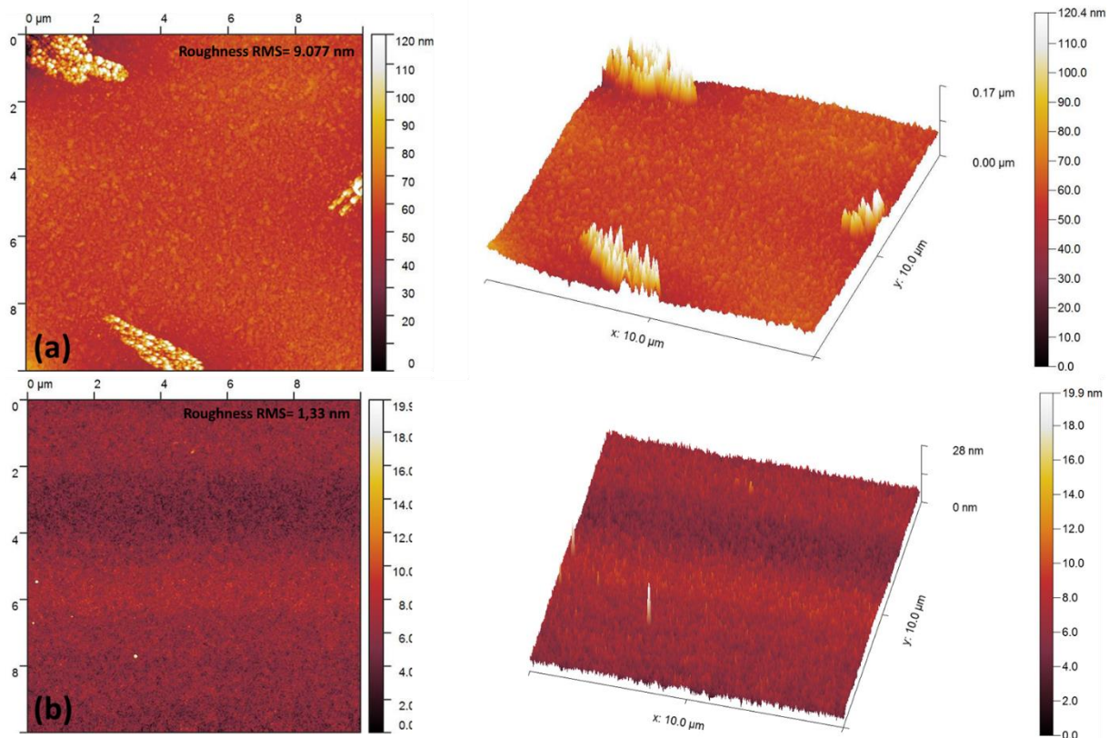
Figure 4.28: AFM surface images for Si 3 N 4 /VO 2 (a) and TiO 2 (A)/VO 2 (b).
