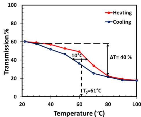
Figure 4.27: Hysteresis curve of the Si 3 N 4 /VO 2 bilayer at \lambda=1500 nm.
