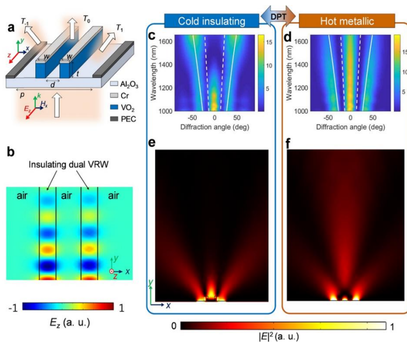
Figure 5.4: Design of the proposed structure consisted of a dual VO 2 ridge waveguide (VRW) (a) and electric field distribution of the TE 0 mode at 1400 nm (b), diffraction angles of the unit cell of the VRW in insulating and metallic phase (c),(d) with the normalized electric field distribution respectively (e),(f) [11].
