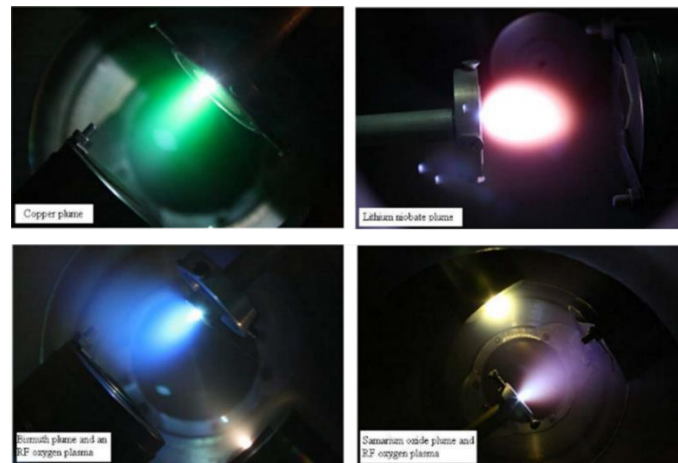
Figure 4.15: Plasma plumes by gas assisted PLD in the chamber [53].
