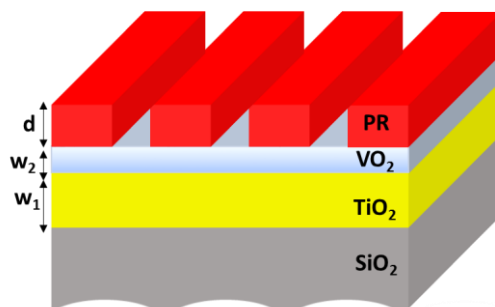
Figure 5.18: Design of the targeted PLD configuration.
