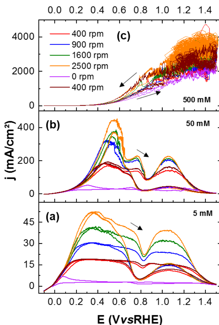
Figure III.3. Ohmic-drop corrected CVs measured on Pt mirror-polished polycrystalline electrodes ( S_{\text{geo}} = 0.031 cm 2 ) in RDE configuration at three different borohydride concentrations: 1 M NaOH + (a) 5 mM, (b) 50 mM, (c) 500 mM NaBH 4 and various rotating rate of the electrode following this cycle: [400; 900; 1600; 2500; 0; 400] rpm. Ar-saturated electrolytes, v_s = 20 mV.s -1 , T = 20^\circ\text{C}
