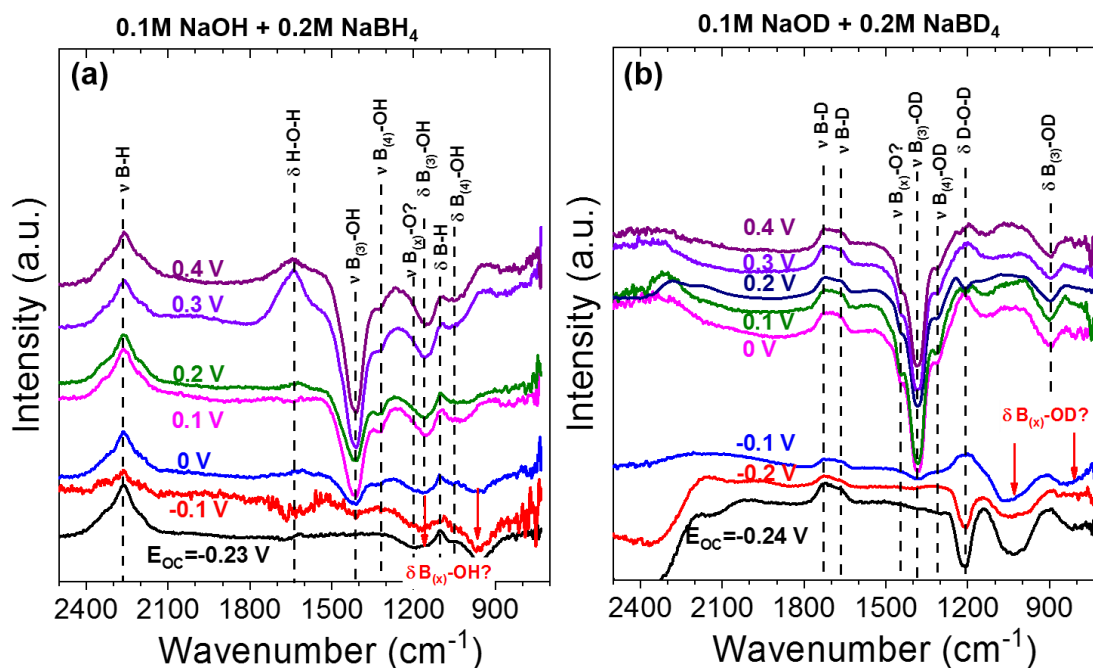
Figure IV.24. In-situ FTIR spectra obtained using a ZnSe prism on a Ni electrode in (a) 0.1 M NaOH + 0.2 M NaBH 4 or (b) 0.1 M NaOD + 0.2 M NaBD 4 electrolytes at potentials increasing from E_{\text{OC}} to E = 0.4 \text{ V} vs RHE.
