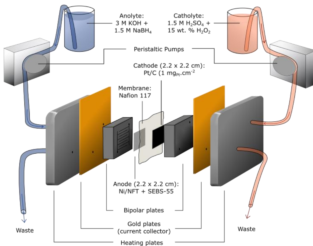
Figure II.21. Schematic representation of the \text{BH}_4^-/\text{H}_2\text{O}_2 DBFC setup. The flow rate of both electrolytes are controlled by two peristaltic pumps. Interdigitated channels were used to ensure the electrolytes passing through the electrodes.
