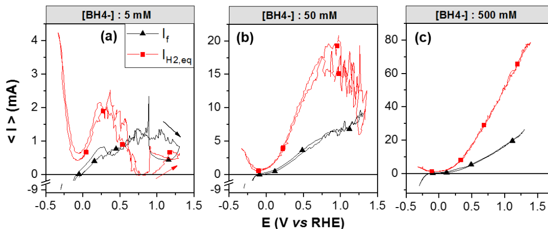
Figure III.15. Faradic current of the BOR on sputtered Pd ( ca. 50 nm thick) and corresponding H_2 escape current ( I_{H_2,eq} ) obtained from the I_{m/z=2} signal and the DEMS calibration (see section II.3.3.1) for (a) 5 mM, (b) 50 mM and (c) 500 mM in 1 M NaOH. (note the presence of a break in the faradic current axis of the HER, for 5 mM and 50 mM NaBH_4 , to observe the oxidation currents more easily). Reprinted from [212].
