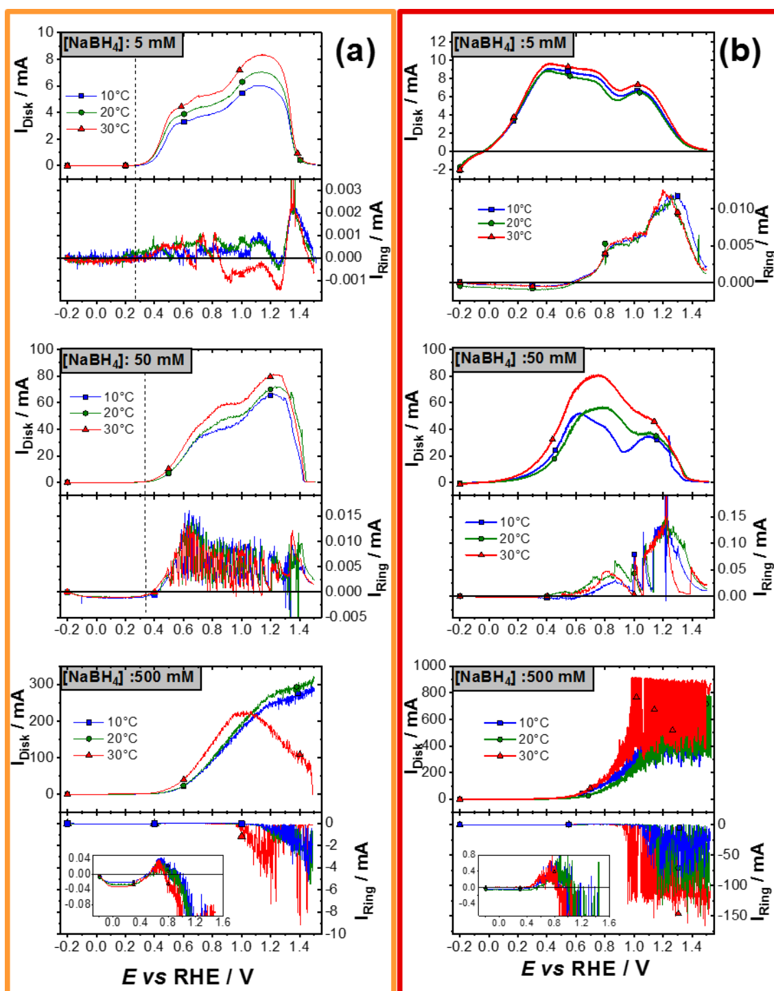
Figure III.8. Ohmic drop-corrected (in dynamic mode) positive scans of the BOR on (a, yellow border) Au and (b, red border) Pt disk electrode for 5, 50 and 500 mM \text{NaBH}_4 in 1 M NaOH, and their corresponding current measured on a Au ring at T = [10, 20, 30]^\circ\text{C} and \omega = 2500 rpm. Ring currents were initially measured with a chronoamperometry at a potential of E = 0.2 V vs RHE and subsequently corrected to fit the potential during the BOR. An inset corresponding to a focus on the low ring currents is presented for 500 mM \text{NaBH}_4 . Reprinted from Ref. [212].
