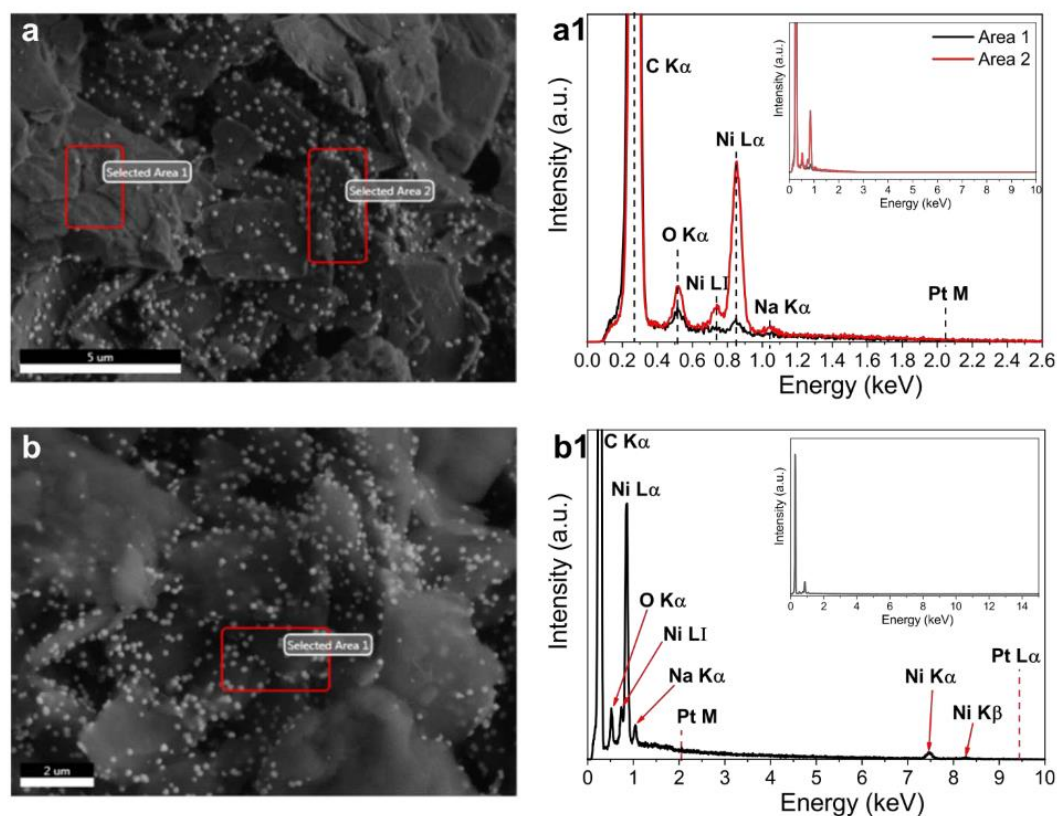
Figure V.3. SEM images of Ni ED /GDE-L sample obtained at (a) 3 kV to scan the low energies region or (b) 10 kV to scan energies high enough to reveal Pt L \alpha and Ni K bands, and corresponding X-EDS analysis from the marked areas (a1, b1).
