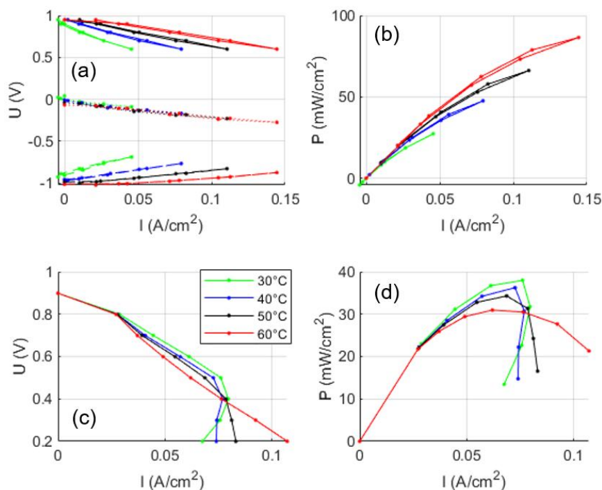
Figure V.7. I - U curves (a, c) and I - P curves (b, d) of a \text{Ni}_{\text{ED}}/\text{GDE} anode in DBFC operation conditions while (a, b) keeping the cell voltage above 0.5 V and (c, d) using the same electrode down to 0.2 V. On panel (a) the local potential of both the anode and cathode, measured using an in situ \text{H}_2 reference are represented.
