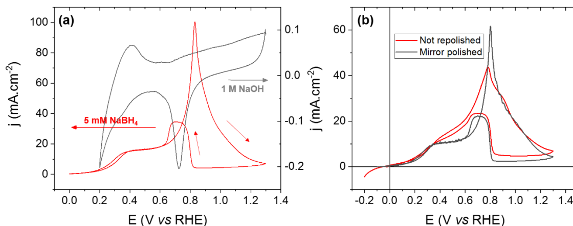
Figure III.16. (a) CV of polycrystalline Pd electrode ( S_{\text{geo}} = 0.031 \text{ cm}^2 ) in supporting electrolyte (grey line) and in presence of 5 mM \text{NaBH}_4 (red line) at \omega = 1600 \text{ rpm} . (b) Comparison of the BOR at 5 mM \text{NaBH}_4 on a polycrystalline Pd mirror-polished prior the measurement (grey line) or the same electrode used after several BOR characterization, without being re-polished (red line) at \omega = 1600 \text{ rpm} . Ar-saturated electrolytes, T = 20^\circ\text{C} , v_s = 20 \text{ mV}\cdot\text{s}^{-1} .
