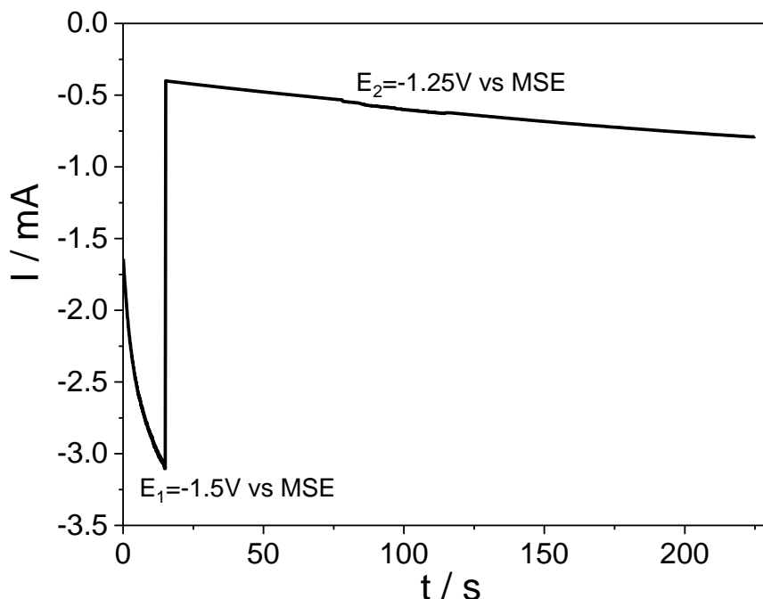
Figure II.5. Ni deposition transients obtained for Ni ED /XC-72R in a deaerated 0.1 M (NH 4 ) 2 SO 4 + 0.01 M NiSO 4 bath. The deposition parameters are as follows E_1 = -1.5 \text{ V} (15 s), E_2 = -1.25 \text{ V} (210 s), \omega = 400 \text{ rpm} , T = 25^\circ\text{C} . Formation of gas bubbles (due to the simultaneous H 2 evolution) was observed during the deposition.
