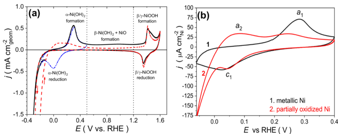
Figure IV.1. (a) CVs of a polycrystalline Ni electrode in N_2 -saturated 0.1 \text{ mol.L}^{-1} NaOH at a sweep rate v_s = 50 \text{ mV.s}^{-1} and T = 25^\circ\text{C} . The first CV in panel a (dash-dotted blue curve) covers the potential range from E = -0.2 to 0.5 \text{ V vs RHE} , while two other CVs (first scan – solid black curve and second scan – dashed red curve) cover the potential range from E = -0.3 to 1.6 \text{ V vs RHE} . (b) CVs obtained for metallic and partially oxidized polycrystalline Ni electrodes in N_2 -saturated 0.1 \text{ mol.L}^{-1} NaOH at a sweep rate v_s = 20 \text{ mV.s}^{-1} and T = 25^\circ\text{C} . Adapted from Ref. [186] with permission from Springer.
