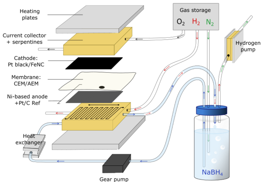
Figure II.20. Schematic representation of the BH_4^-/O_2 DBFC setup. The analyte is recirculated in the system and its flow is ensured by a gear pump. The amount of H_2 escaping the cell is measured in situ using an in-line half PEMFC cell in the hydrogen pump mode.
