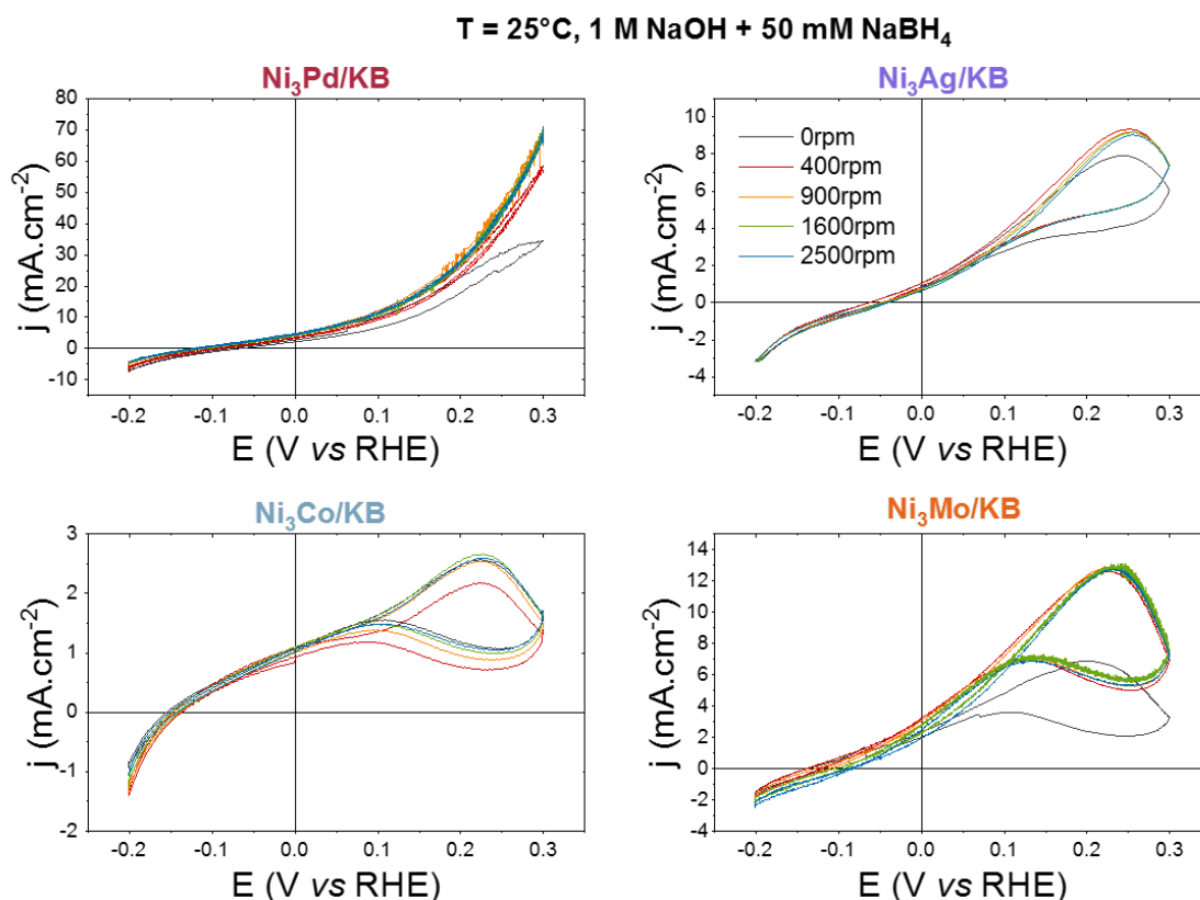
Figure IV.8. CVs of Ni 3 M/KB catalysts from UNM [195,196] at increasing rotation rate of the RDE in BOR conditions: 1 M NaOH + 50 mM NaBH 4 , v_s = 20 mV.s -1 , room temperature, Ar-saturated electrolyte, metal loading: I_{\text{metal}} = 100 \mu\text{g.cm}^{-2} .
