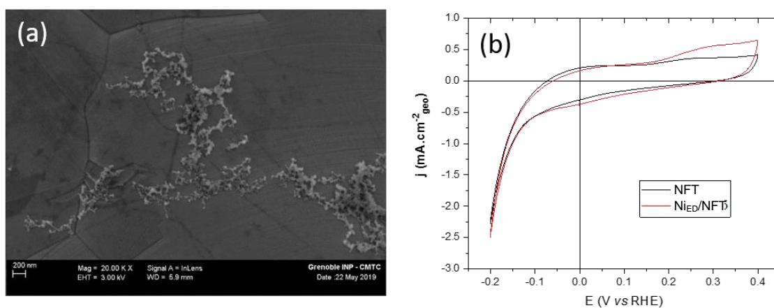
Figure V.11. (a) SEM image of Ni electrodeposited on NFT (F 0.5) without etching at \times 20k magnification. (b) Corresponding electrochemical profiles of the felt before and after Ni ED in 1 M NaOH at v_s = 20 \text{ mV.s}^{-1} and T = 25^\circ\text{C} . No major improvement of the peak at 0.25 V vs RHE is observed.
