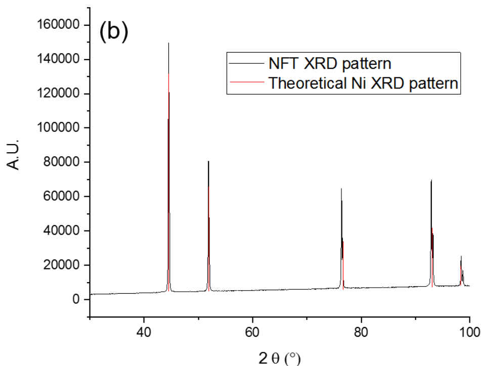
Figure II.13. XRD pattern of (a) the NFM and (b) the NFT, compared to the theoretical pattern of Ni (cubic Fm-3m (225)) (red lines).
