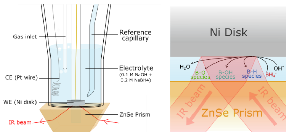
Figure II.16. Schematic representation of the in situ FTIRS setup using a ZnSe prism. The thin layer is detailed on the right-hand side with the expected intermediates or final products of the BOR.
