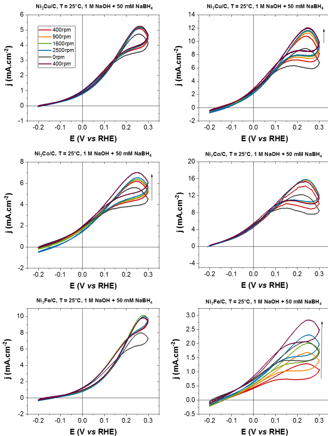
Figure IV.9. CVs of Ni x M/C catalysts from Technion [283] at increasing rotation rate of the RDE in BOR conditions: 1 M NaOH + 50 mM NaBH 4 , v_s = 20 \text{ mV.s}^{-1} , room temperature, Ar-saturated electrolyte, metal loading: I_{\text{metal}} = 100 \mu\text{g.cm}^{-2} .
