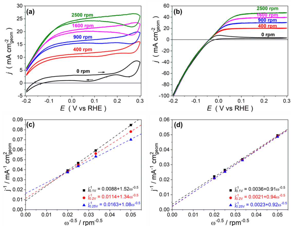
Figure IV.17. CV curves obtained for (a) NiED/C and (b) Pt/C using rotating disk electrode in \text{N}_2 -saturated 1.0 M NaOH + 5 mM \text{NaBH}_4 electrolyte at v_s = 20 \text{ mV}\cdot\text{s}^{-1} and various rotation speeds. (c, d) Corresponding Koutecky-Levich plots at various potentials.
