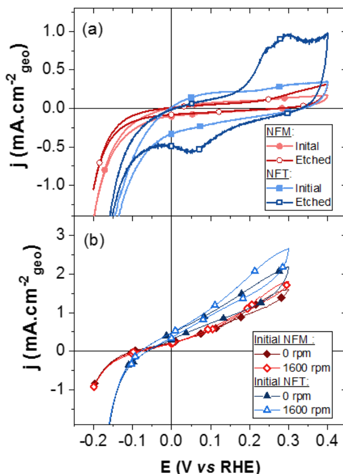
Figure V.10. Cyclic voltammograms at v_s = 20 \text{ mV}\cdot\text{s}^{-1} of NFM and NFT in (a) Ar-saturated supporting electrolyte (1 M NaOH, T = 25^\circ\text{C} ) showing their electrochemical profile at their initial state and after acid etching for 2 hours in 2 M \text{C}_6\text{H}_8\text{O}_6 and in (b) BOR conditions (Ar-saturated 50 mM \text{NaBH}_4 + 1 \text{ M NaOH} , T = 25^\circ\text{C} ) showing their performance with or without rotation of the RDE ( \omega = 0 or 1600 rpm) at their initial state. Reprinted from Ref. [391].
