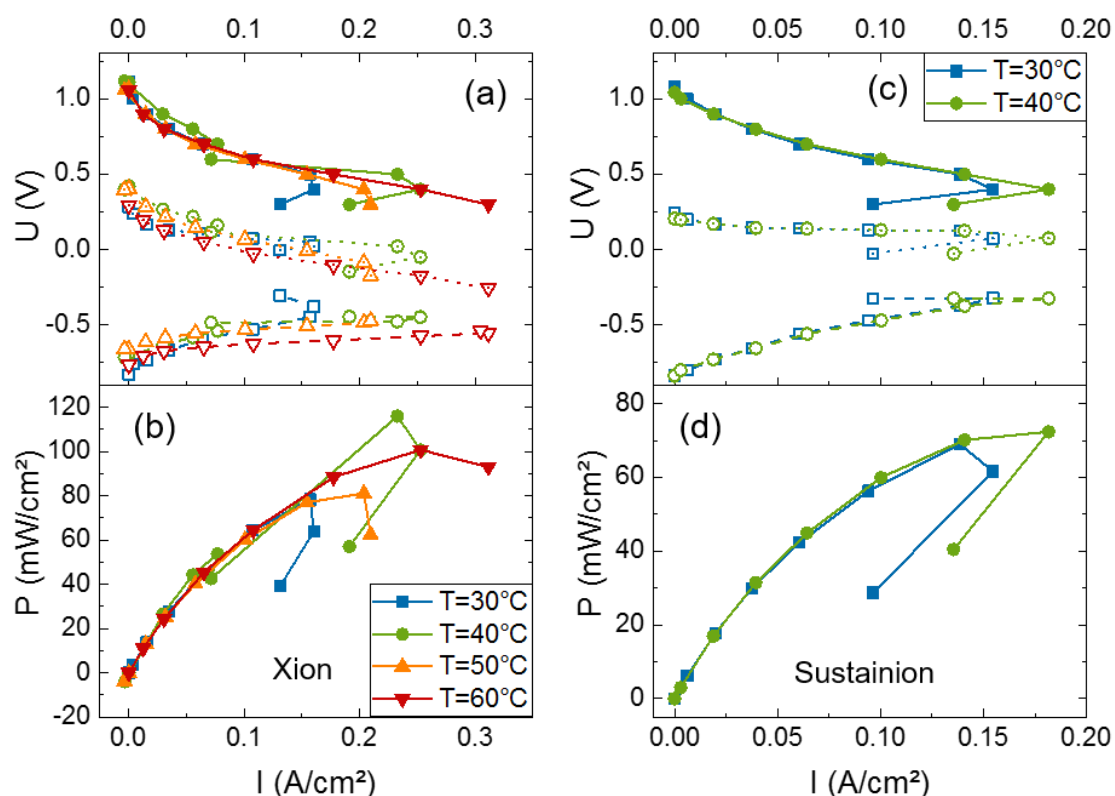
Figure V.21. (a, c) I - U curves with cathode (dotted lines) and anode (dash lines) potentials measured using an in situ \text{H}_2 reference and (b, d) I - P curves of DBFC using \text{Ni}_{\text{ED}}/\text{eNFT} anodes and Fe-N-C (Sustainion binder) cathodes in alkaline conditions. Performance obtained using (a, b) a commercial Xion AEM and (c, d) a commercial Sustainion AEM.
