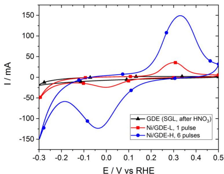
Figure V.1. CVs obtained in N 2 -saturated 1 M NaOH at v_s = 20 \text{ mV} \cdot \text{s}^{-1} for SGL (black curve) and new Ni ED -based electrodes. Ni ED /GDE-L (red curve, ECSA = 537 cm 2 ) is obtained with 1 pulse and Ni ED /GDE-H (blue curve, ECSA = 2823 cm 2 ) with 6 pulses of electrodeposition.
