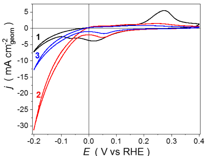
Figure II.7. CVs of Ni ED /C electrode in supporting electrolyte (1 M NaOH) at the three different oxidation states: (1) metallic; (2) partially oxidized; (3) strongly oxidized. N 2 -saturated electrolyte, v_s = 20 mV.s -1 , \omega = 0 rpm, T = 25 °C.
