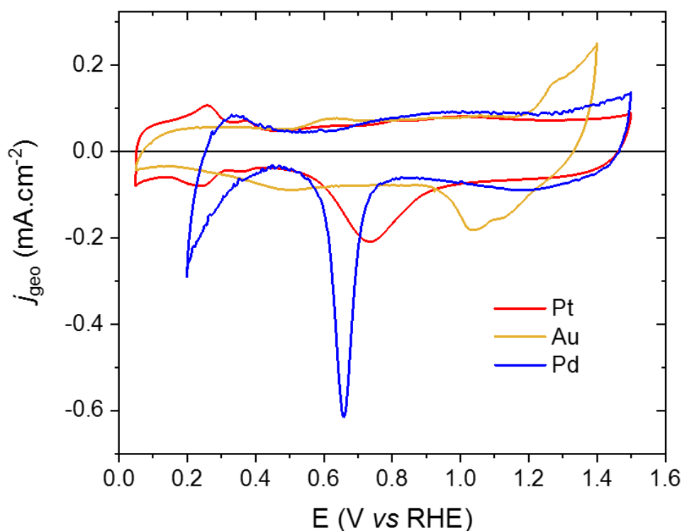
Figure II.2. CVs in supporting electrolyte (1 M NaOH) of noble mirror-polished noble metal electrodes: Pt, Au and Pd. S_{\text{geo}} = 0.031 \text{ cm}^2 , v_s = 20 \text{ mV}\cdot\text{s}^{-1} , \omega = 0 \text{ rpm} , T = 20^\circ\text{C} , Ar-saturated electrolyte.
