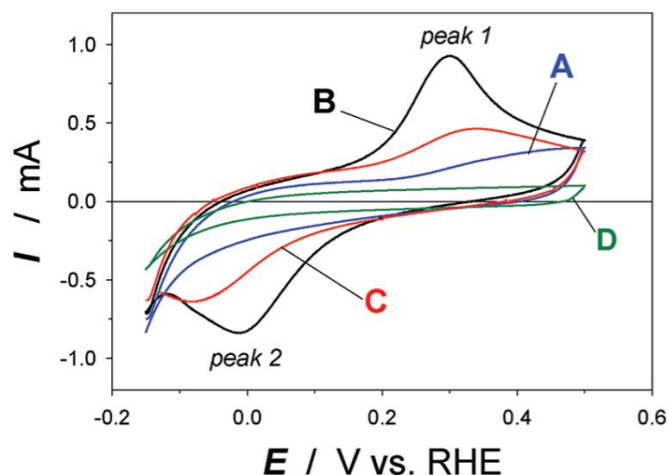
Figure V.12. Cyclic voltammograms in 0.5 M aqueous KOH solution obtained at T = 298\text{ K} and v_s = 100\text{ mV}\cdot\text{s}^{-1} in the -0.15 \leq E \leq 0.50\text{ V} potential range for (A) the “as-received” Ni foam, (B) the “etched” Ni foam for 2 min, (C) the “reduced” Ni foam, and (D) the “passivated” Ni foam. Figure reproduced from Grdeń et al [189].
