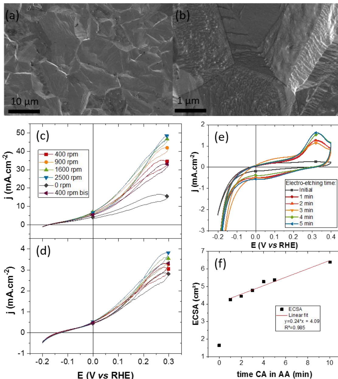
Figure V.13. SEM images (a, b) of NFT after 2 h etching in 2 M C 6 H 8 O 6 at (a) ×200 and (b) ×2000 magnification. (c, d) Cyclic voltamograms of NFT (c) and NFM (d) in 50 mM NaBH 4 + 1 M NaOH ( T = 25^\circ\text{C} ) after 2 h etching in 2 M C 6 H 8 O 6 with RDE rotation variation: [0, 400, 900, 1600, 2500] rpm. (e) CVs of NFT in supporting electrolyte (1 M NaOH, T = 25^\circ\text{C} ) probing the surface modifications between 1 min electro-assisted etching steps (1 min CA at 0.715 V vs RHE in 2 M C 6 H 8 O 6 + 0.1 M (NH 4 ) 2 SO 4 ). (f) Linear fit of the ECSA increase with the CA time in 2 M C 6 H 8 O 6 + 0.1 M (NH 4 ) 2 SO 4 . Reprinted from Ref. [391].
