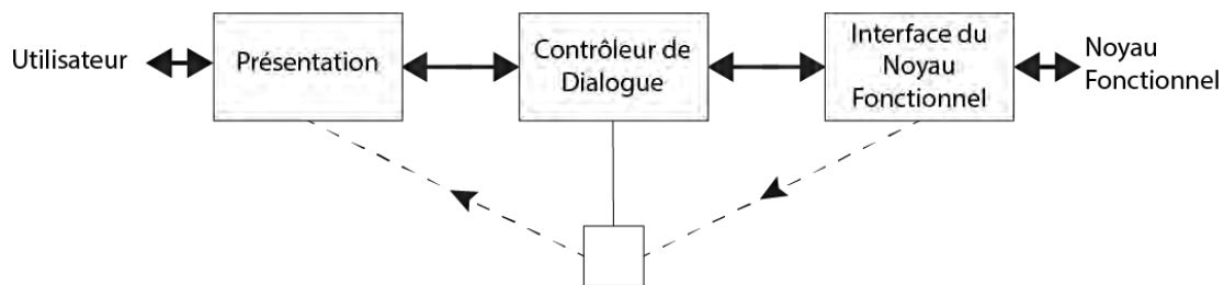
Figure 3. Architecture Seeheim
