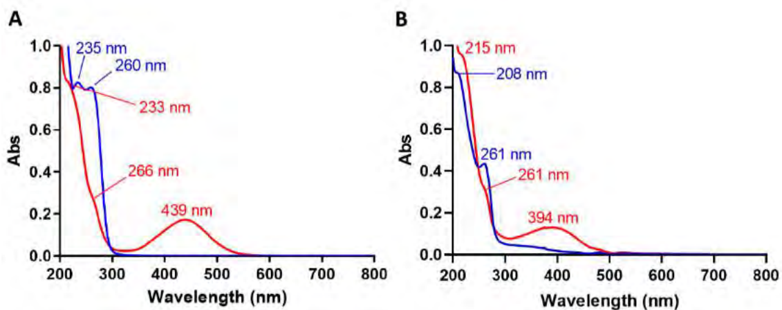
Figure 45. UV-Visible absorption spectra of the (A) ligand 5 ( 217 \mu\text{M} , blue) and complex 6H + ( 50 \mu\text{M} , red), and (B) ligand 10 ( 105 \mu\text{M} , blue) and complex 13H + ( 47 \mu\text{M} , red), in water solution, at pH = 6.8.
