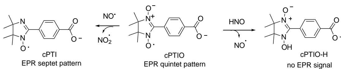
Figure S3. Reactions of cPTIO with \text{NO}\cdot or \text{HNO} , and EPR patterns of the products.
