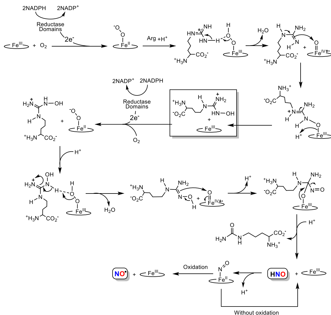
Scheme 2. The biological synthesis of NO• and likely production of HNO by NOS, references [51,78,80,83,84].
