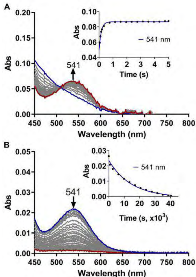
Fig. 6. Spectral changes investigated by stopped-flow measurement during the reaction of trans\text{-}[\text{Fe}(\text{cyclam})(\text{NO})\text{Cl}]^{2+} (5 mM) with GSH (150 mM) (A) and the same reaction between trans\text{-}[\text{Fe}(\text{cyclam})(\text{NO})\text{Cl}]^{2+} (300 \mu\text{M} ) with GSH (9 mM) by UV-Vis (B) in 0.5 M phosphate buffer pH 7.4 solution at 37 °C and under aerobic conditions. Inset: kinetic curve monitored at 541 nm (first order equation fit, in A k_{\text{obs}} = 6.31 \text{ s}^{-1} , R^2 = 0.9936 , in B k_{\text{obs}} = 6.93 \times 10^{-5} , R^2 = 0.9830 ).
