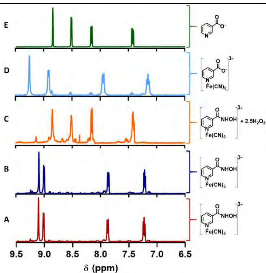
Figure 49. 1 H-NMR spectra at 400 MHz: of the complex 13H + (20 mM) at 0 h (A) and at 52 h (B) without addition of \text{H}_2\text{O}_2 , at 52 h after reaction of 13H + with \text{H}_2\text{O}_2 (50 mM) (C), and 15 complex (20 mM) (D) and nicotinic carboxylate ( 12 ) (20 mM) (E). Solutions in 40 mM phosphate buffer, pH 7.4, at 25 °C.
