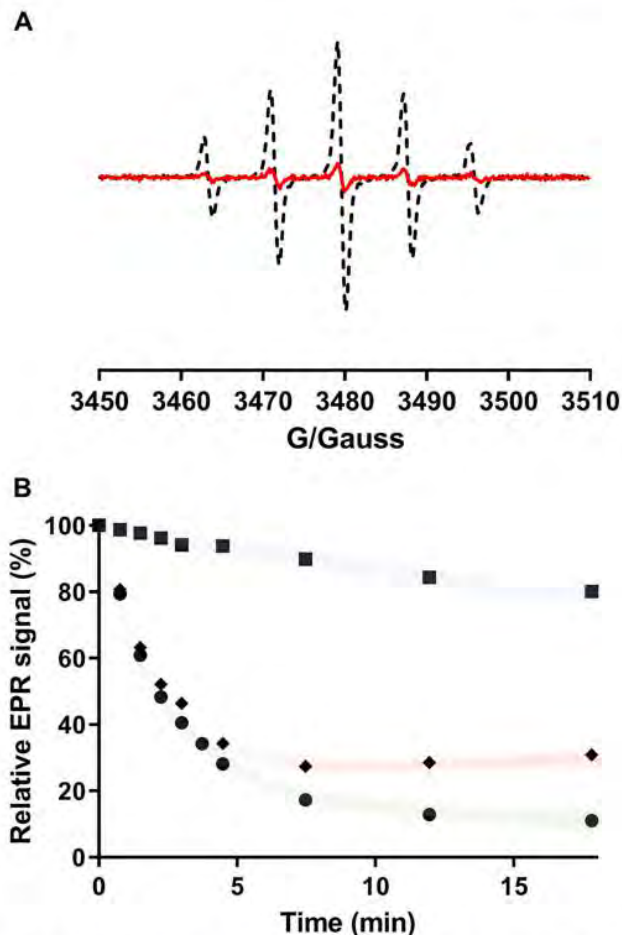
Fig. 5. EPR monitoring of the reaction of 1 (400 \mu\text{M} ) with GSH (4 mM) using cPTIO (200 \mu\text{M} ) as probe, in 0.1 mM phosphate buffer pH 7.4 solution, at 25 °C, and aerobic conditions. A. EPR spectra right before (dashed line) and after (solid line) 18 min of reaction. B. A trend of the EPR signal of reaction of cPTIO with trans -[Fe(cyclam)(NO)Cl] ^{2+} and GSH (circles) for 18 min; control reaction of GSH with cPTIO (square); result of the subtraction of the first and second measurements described above (diamond).
