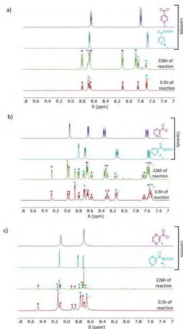
Fig. 2 ^1H NMR spectra of the K_3[Fe^{III}(CN)_6] -mediated oxidation of (a) isonicotinohydroxamic acid (b) nicotinohydroxamic acid and (c) pyrazino-hydroxamic acid at 0.5 h and 226 h using K_3[Fe^{III}(CN)_6] in D_2O , at room temperature and authentic samples of (a) isonicotinohydroxamic acid and sodium isonicotinoate, (b) nicotinohydroxamic acid and sodium nicotinoate and (c) pyrazinohydroxamic acid and sodium pyrazinoate. Symbols: blue squares: starting hydroxamic acid, red stars: intermediate product, pink triangle: final carboxylic acid under carboxylate salt form.
