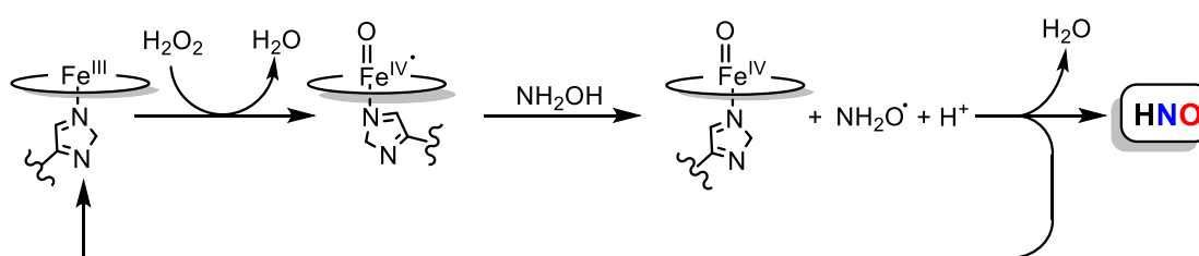
Scheme 4. HNO synthesis via oxidation of hydroxylamine ( \text{NH}_2\text{OH} ) mediated by heme proteins and \text{H}_2\text{O}_2 [112,117-120].
