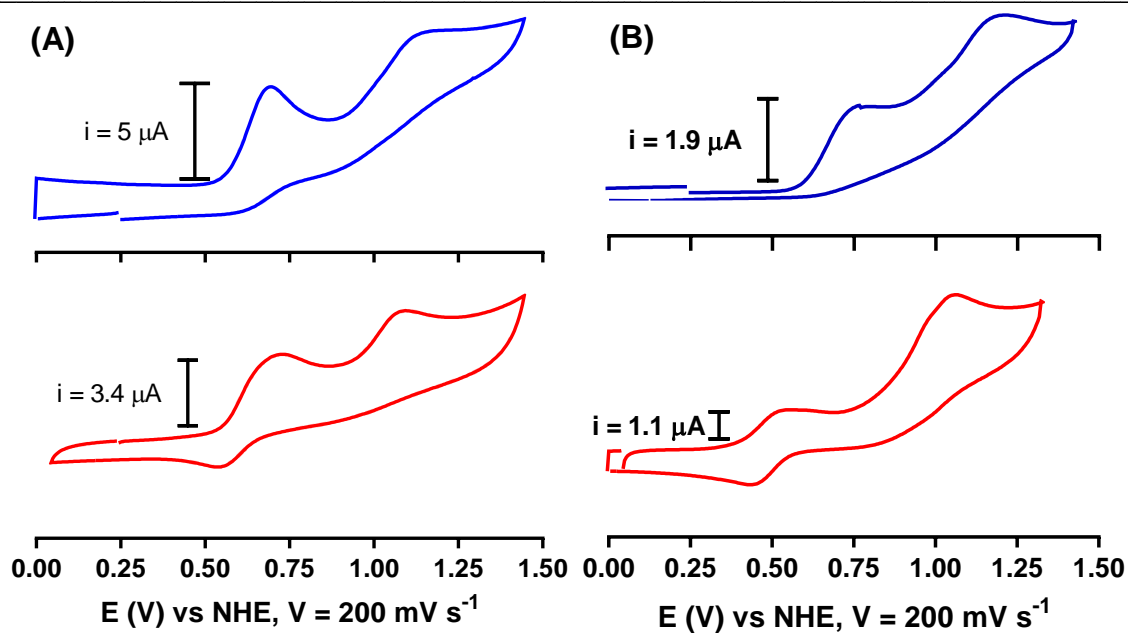
Figure S2 - Cyclic voltammograms of glassy carbon electrode in solution of compound [\text{Fe}^{\text{II}}(\text{CN})_5(\text{PyZCONHO})]^{3-} (A) and [\text{Fe}^{\text{II}}(\text{CN})_5(\text{PyCONHO})]^{3-} (B), using vitreous carbon electrode as work, platinum electrode as auxiliary electrode and saturated calomel electrode (SCE) as reference, in phosphate buffer 0.1M pH 7.4 as electrolyte. Scan speed of 200 \text{ mV s}^{-1} . Potential values were plotted from SCE to NHE for comparative purposes. Ligands in blue and complex in red.
