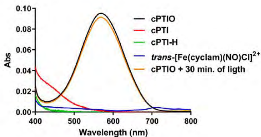
Fig. S7 Electronic spectra of cPTIO (—), cPTI (—) (resulted of cPTIO in reaction with \text{NO}^\bullet , from a \text{NO}^\bullet saturated solution), cPTIO-H (—) (resulted of cPTIO in reaction with \text{HNO} by using Angeli's salt ( 200\ \mu\text{M} )), trans\text{-}[\text{Fe}(\text{cyclam})(\text{NO})\text{Cl}]^{2+} (—) ( 200\ \mu\text{M} ) after 30 min of light irradiation at 365 nm and cPTIO (—) after 30 min of light irradiation at 365 nm. All electronic spectra were obtained in 0.1 M phosphate buffer pH 7.4 solution at 37\ ^\circ\text{C} , under aerobic conditions. The concentration of cPTIO used in all assays was 100\ \mu\text{M} .
