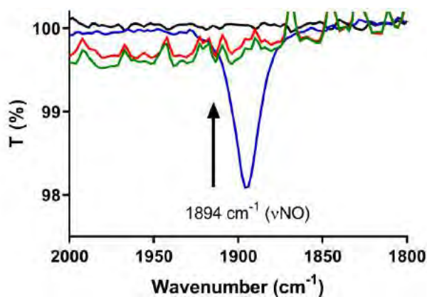
Fig. S10 Investigation of the reaction of trans -[Fe(cyclam)(NO)Cl] 2+ (10 mM) with glutathione (GSH, 100 mM) in 0.1 M phosphate buffer pH 7.4 solution monitored by FTIR-ATR at 25 °C, under aerobic conditions. Phosphate buffer (—), GSH (—), complex trans -[Fe(cyclam)(NO)Cl] 2+ (—) and mixture containing the complex and GSH after 5 min of reaction (—).
