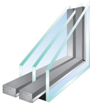
Fig. 2-5 Triple glazed windows of the Passive House UPB
