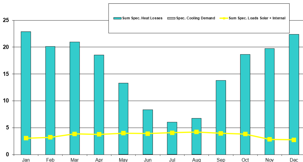
Fig. 4-6 Specific losses, loads and cooling demand (kWh/m 2 month)
