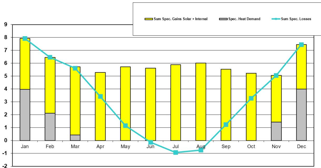
Fig. 4-4 Specific losses, gains, heating demand (kWh/m 2 month - Reference to habitable area)
