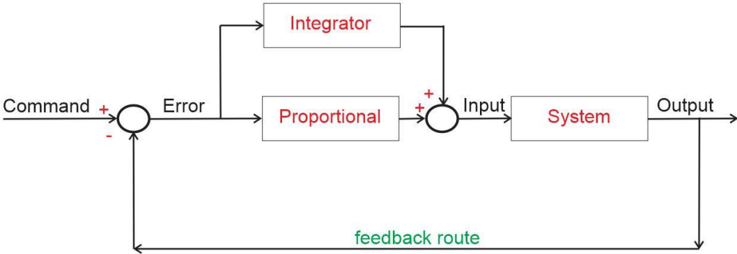
Fig. 1-11 PID controller with feedback and integrator
