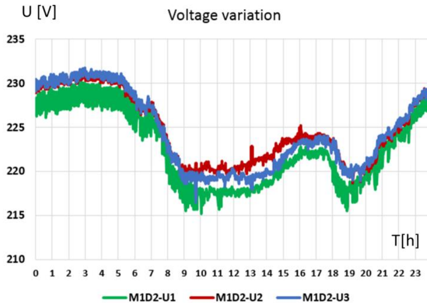
Fig. 3-26 Voltage evolution [99]
