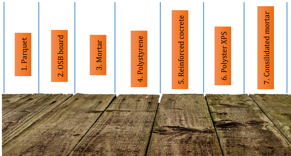
Fig. 2-6 Floor slab of the building
