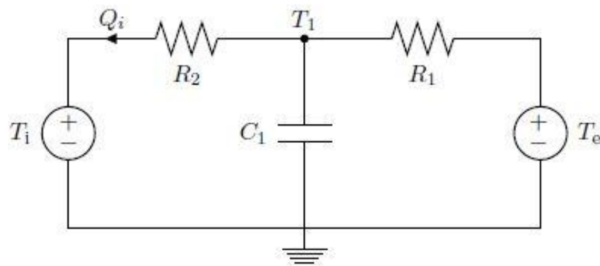
Fig. 4-8 RC diagram
