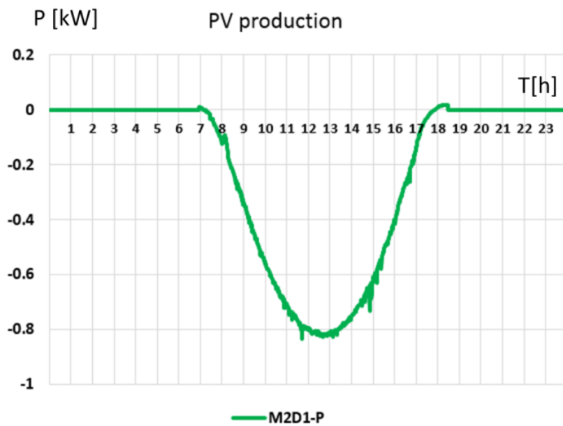
Fig. 3-29 PV Production [99]
