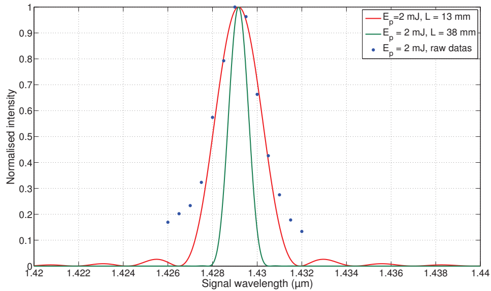
(a) The best agreement is obtained for \lambda_s = 1.428 \mu\text{m} when an interaction length L = 13 \text{ mm} is considered in Equation (178).
