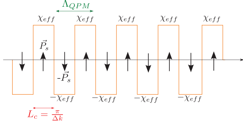
Figure 10: Modulation of the direction of the spontaneous polarization \vec{P}_s and of the sign of the effective coefficient \chi_{eff} of an ideal periodically poled material, i.e. with a duty ratio of 0.5.
