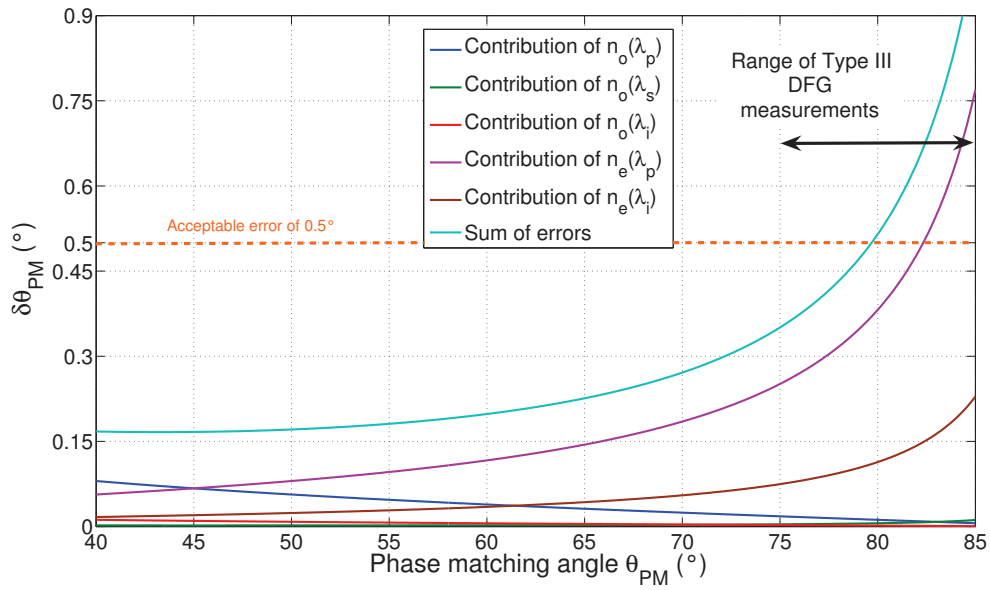
Figure 34: Plot of the absolute values of the different contributions of the principal refractive indices to the phase-mismatch error as a function of the phase-matching angle for type III DFG in CdSiP 2 , when an error of 0.0001 is assumed on each refractive index. The birefringence is -0.05.
