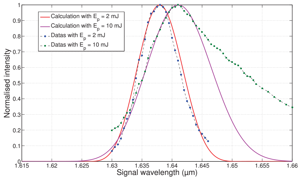
(b) Spectral broadening around 1.64 \mu\text{m} . The length of the crystal used for calculation corresponds to that determined on Figure (75) i.e. L = 19 mm here.
