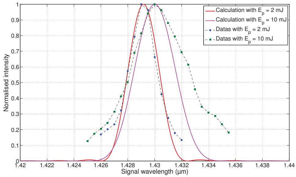
(a) Spectral broadening around 1.43 \mu\text{m} . The length of the crystal used for calculation corresponds to that determined on Figure (75) i.e. L = 13 mm here.
