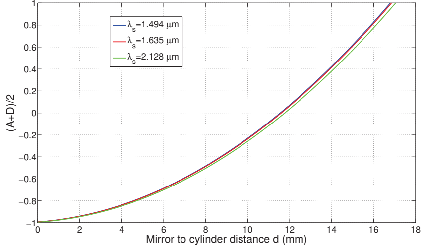
Figure 54: Stability condition of the cavity studied in this work.
