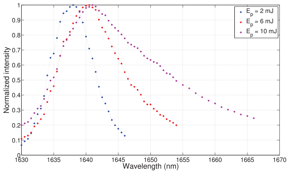
Figure 71: Spectrum of the generated signal around 1.64 μm for different pump intensities.
