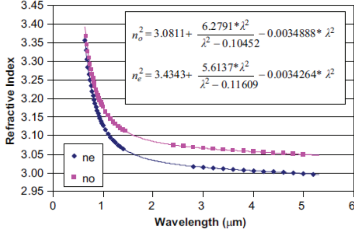
Figure 20: Measured and extrapolated values of the principal refractive indices of CSP, from [42]
