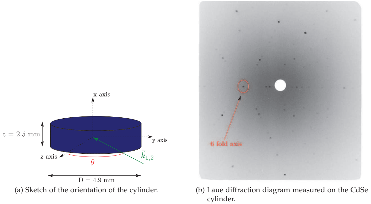
Figure 102: Crystallographical orientation of the 4.9-mm-diameter CdSe cylinder.
