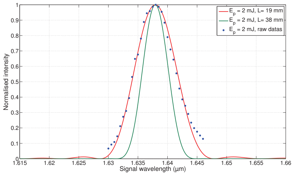
(b) The best agreement is obtained at \lambda_s = 1.64 \mu\text{m} when an interaction length L = 19 \text{ mm} is considered in Equation (178).
