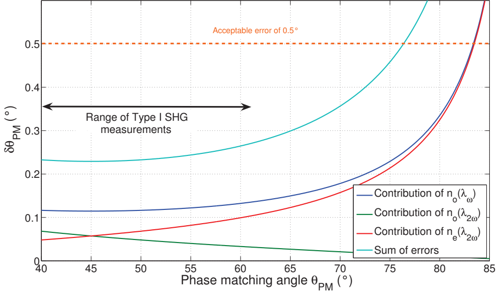
Figure 30: Plot of the absolute values of the different contributions of the principal refractive indices to the phase-mismatch error as a function of the phase-matching angle for type I SHG in CdSiP 2 . An error of 0.0001 is assumed on each refractive index, the fundamental wavelength is set at 6 μm for the calculations presented here. The birefringence is -0.05.
