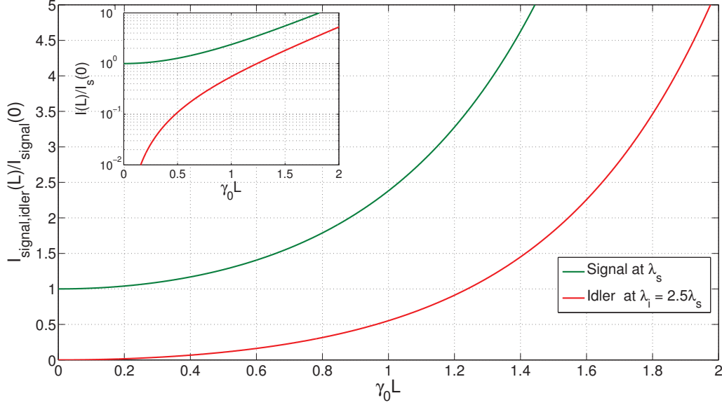
Figure 6: Example of intensities of the amplified signal and generated idler waves in an Optical Parametric Amplifier. The exponential behavior at high gains predicted in Equation (55) is shown in insert on a logarithmic plot.
