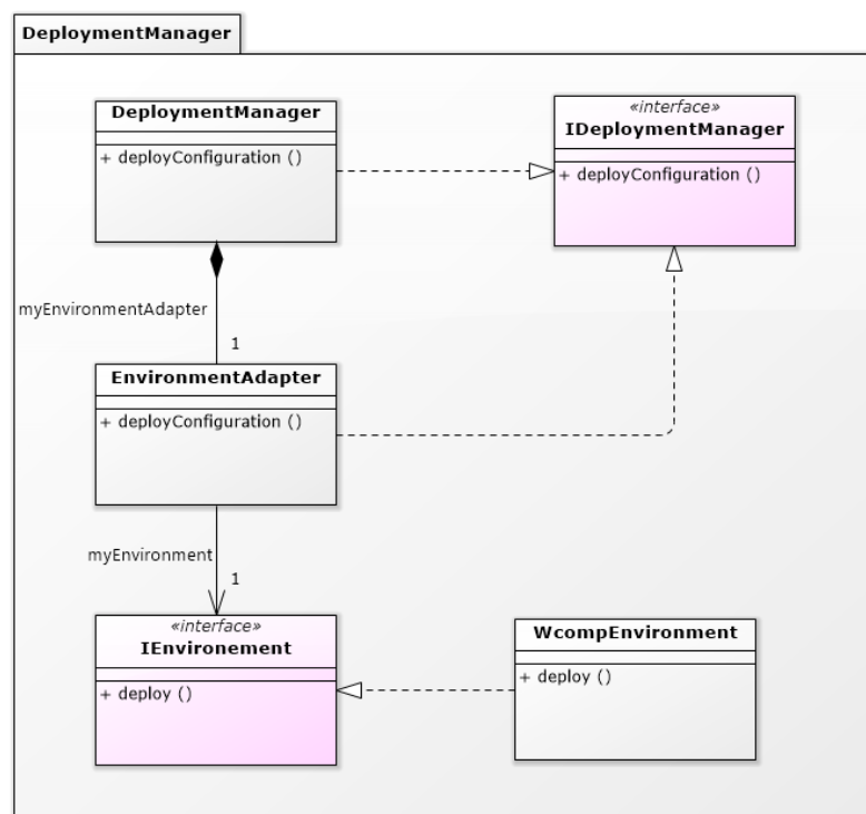
Figure 9.5 – Diagramme de classes du DeploymentManager
