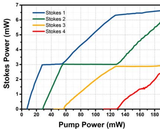
Figure 4.5: Power characterization of MBL_{HQ} cavity
