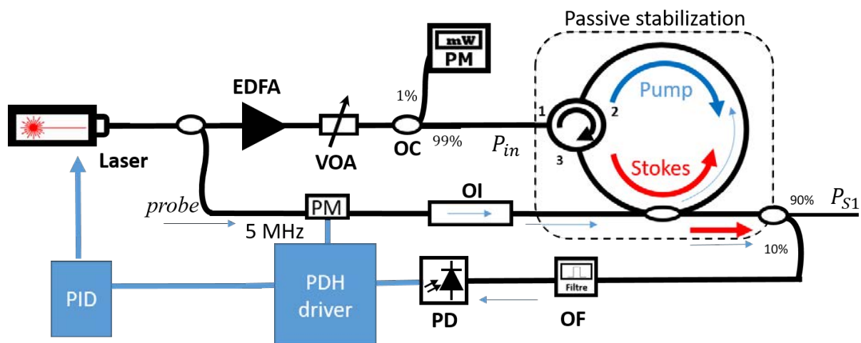
Figure 3.6: Experimental setup of BFL cavity with active PDH locking on cavity a resonances. EDFA: Erbium-doped fiber amplifier, VOA: Variable optical attenuator, OC: Optical coupler, PD: Photodetector, PM: Phase modulator, OI: Optical isolator, OF: Optical filter.
