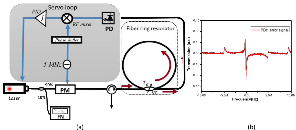
Figure 1.11: (a) General scheme of PDH frequency stabilization. (b) Experimental Oscilloscope traces for PDH error signal. PM: Phase modulator, PD: photodetector, PID: Proportional–integral–derivative controller, VC: Variable coupler, FN: Frequency noise measurement bench.
