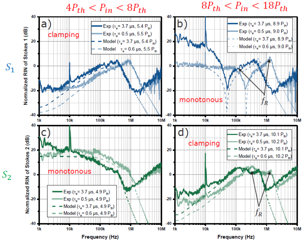
Figure 4.9: Normalized RIN of Stokes 1 (a, b) and Stokes 2 (c, d) lines for various input pump power. Full and dashed lines hold for experimental and simulation results respectively. Deep and light colors referred to high ( \tau_0 = 1.4 \mu\text{s} , \tau_e = 3.7 \mu\text{s} ) and low-Q factors ( \tau_0 = 1.4 \mu\text{s} , \tau_e = 0.5 \mu\text{s} ) respectively.
