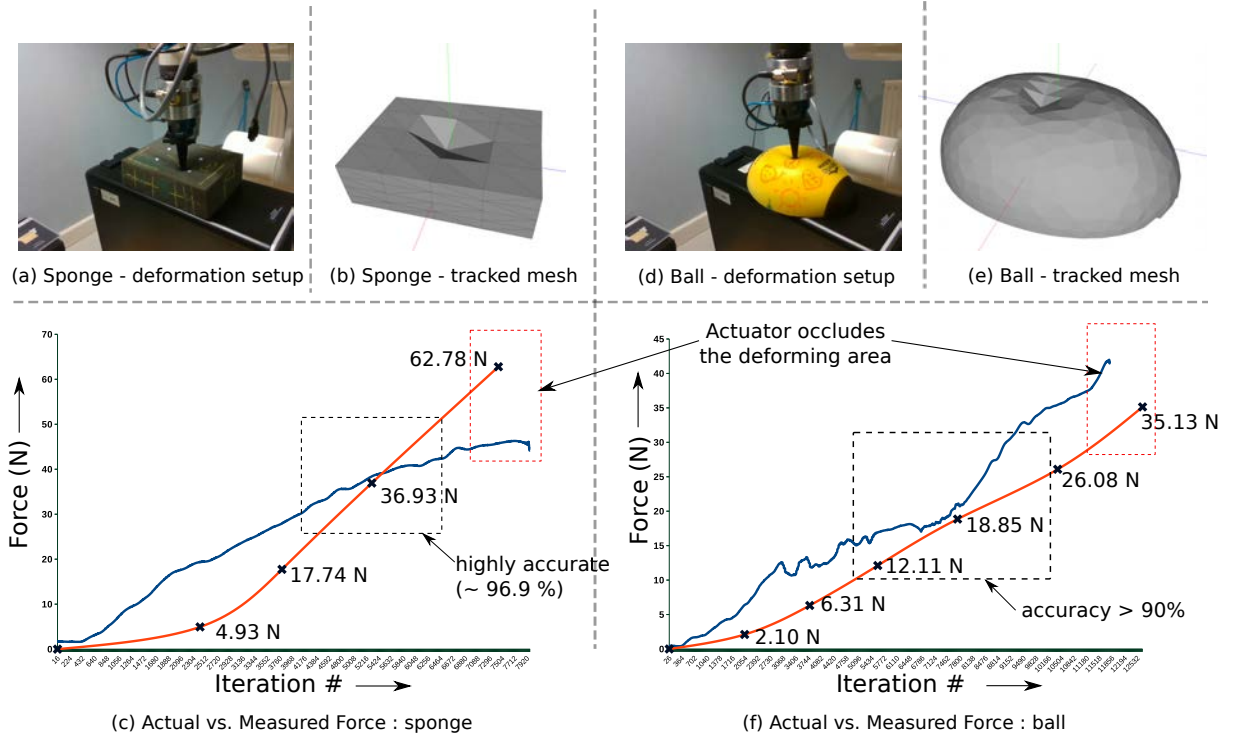
FIGURE 4.5 – Setup and results for force tracking on the sponge . The Viper 850 robot is being used deform the object while being tracked. The red plot is the force measurement from the robot’s force sensor, the blue plot is the estimated force reported by the proposed approach
