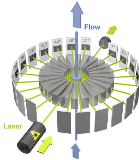
Fig. 26. Scheme of a multi-angle laser light scattering detector.
