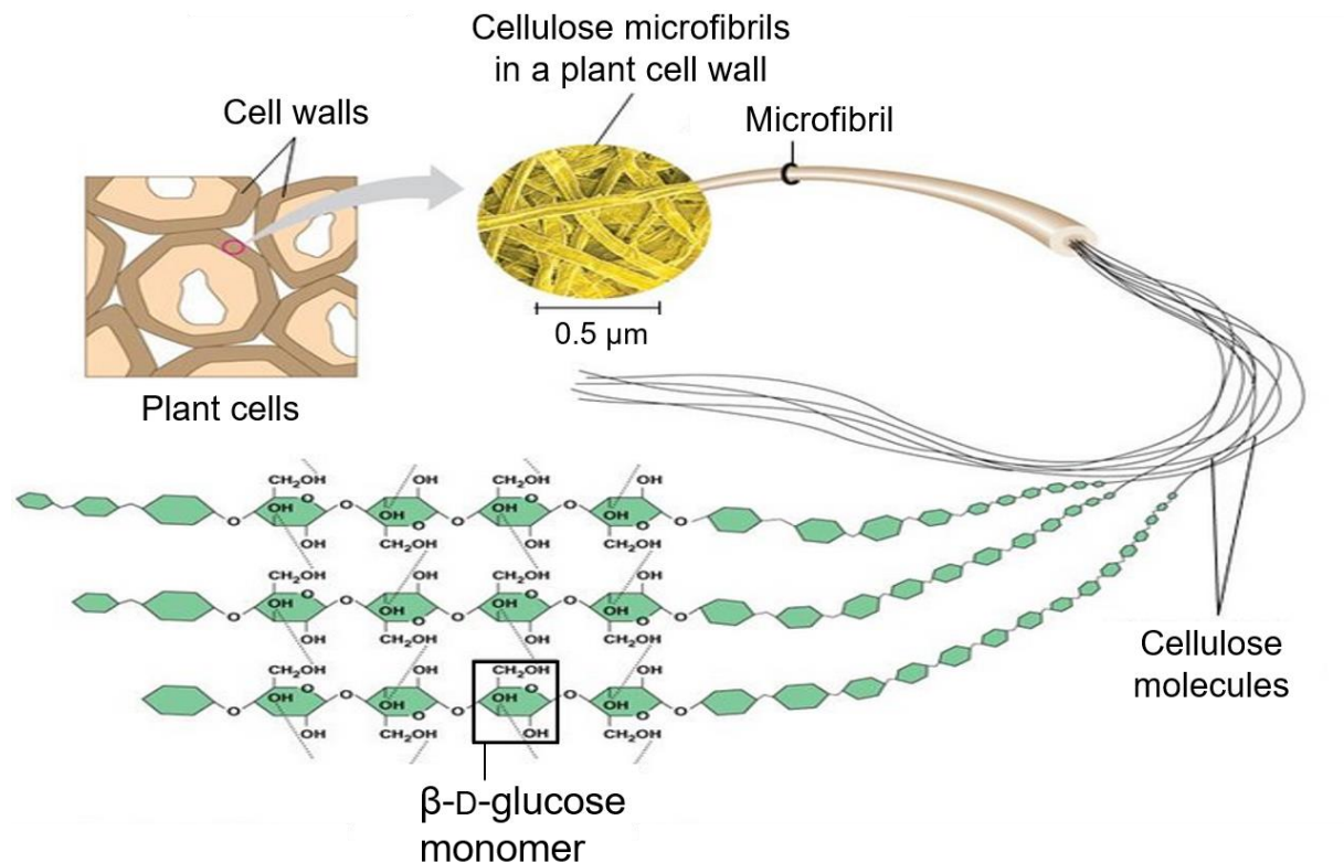
Fig. 9. Chemical structure of cellulose.
