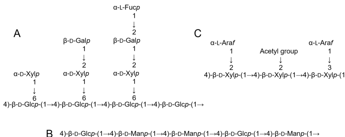
Fig. 10. Chemical structure of xyloglucan (A), glucomannan (B) and arabinoxylan (C). Ara: Arabinose; Gal: Galactose; Glc: Glucose; Man: Mannose; Xyl: Xylose.
