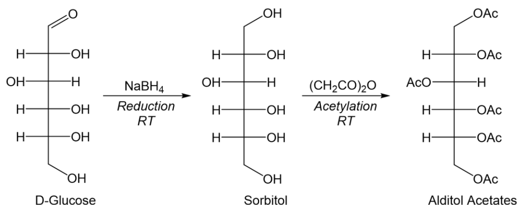
Fig. 53. Main reactions during neutral sugar determination by GC-FID.
