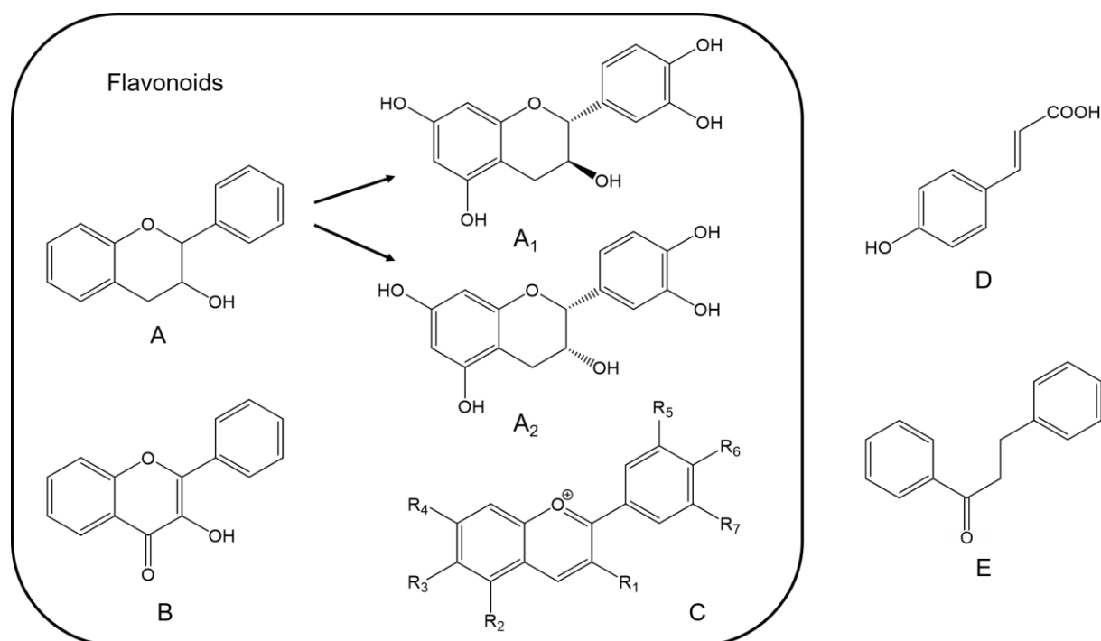
Fig. 4. Chemical structure of common polyphenols in apples.
