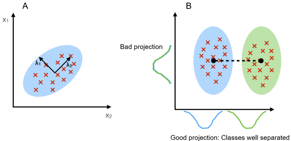
Fig. 60. Comparison between principal component analysis (PCA, A) and linear discriminant analysis (LDA, B).
