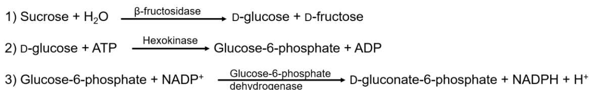
Fig. 51. Scheme of enzymatic reactions during quantification of glucose (A), fructose (B) and sucrose (C).
