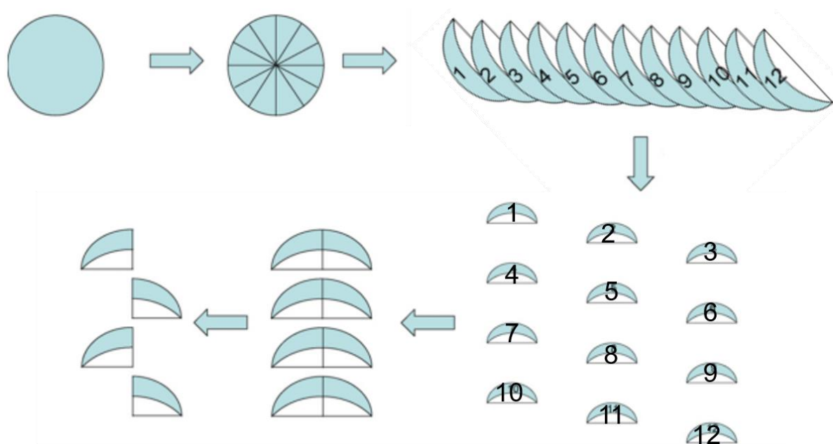
Fig. 52. Scheme of systematic apple fractionation for AIS analysis.
