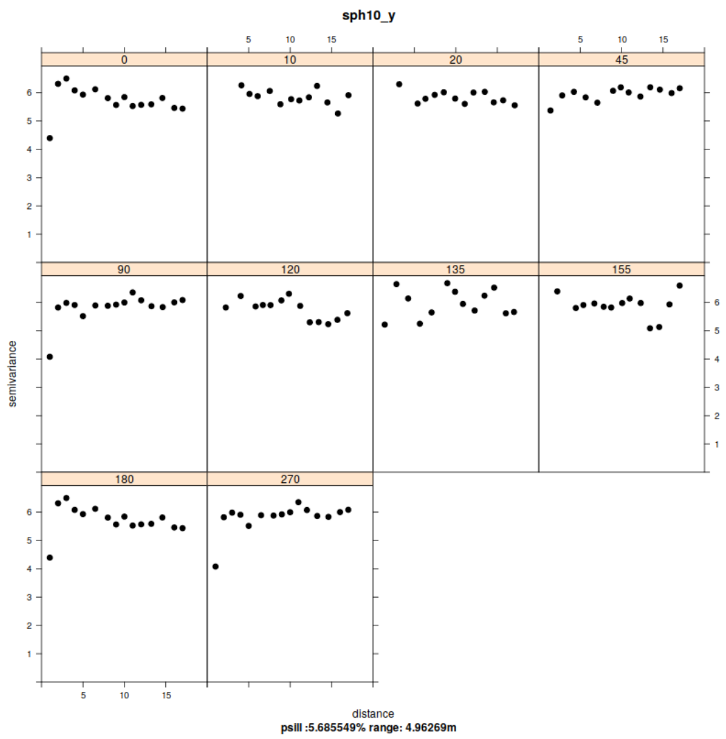
Figure 8.46: Directional variogram analysis of N-S profile of the simulation spherical (10m) nr. 204.
