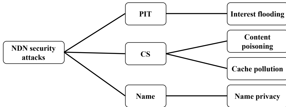
FIGURE 2.1: Proposed taxonomy for NDN security attacks
