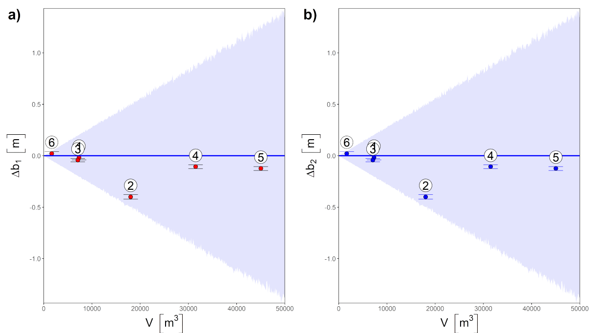
Figure 4.6: Relation \Delta b_1 \leftrightarrow V (a) and \Delta b_2 \leftrightarrow V (b) for the Ardèche River at Meyras, France. Calibration data are the estimated \Delta b and V for each reference morphogenic event. The number above the calibration data represent the index of the reference event. The blue line represents the maximum a posteriori and the blue ribbon illustrates the total uncertainty at 95 %.
