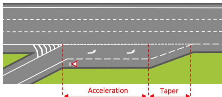
FIGURE 5-4 – Entrance Lane of highway.
