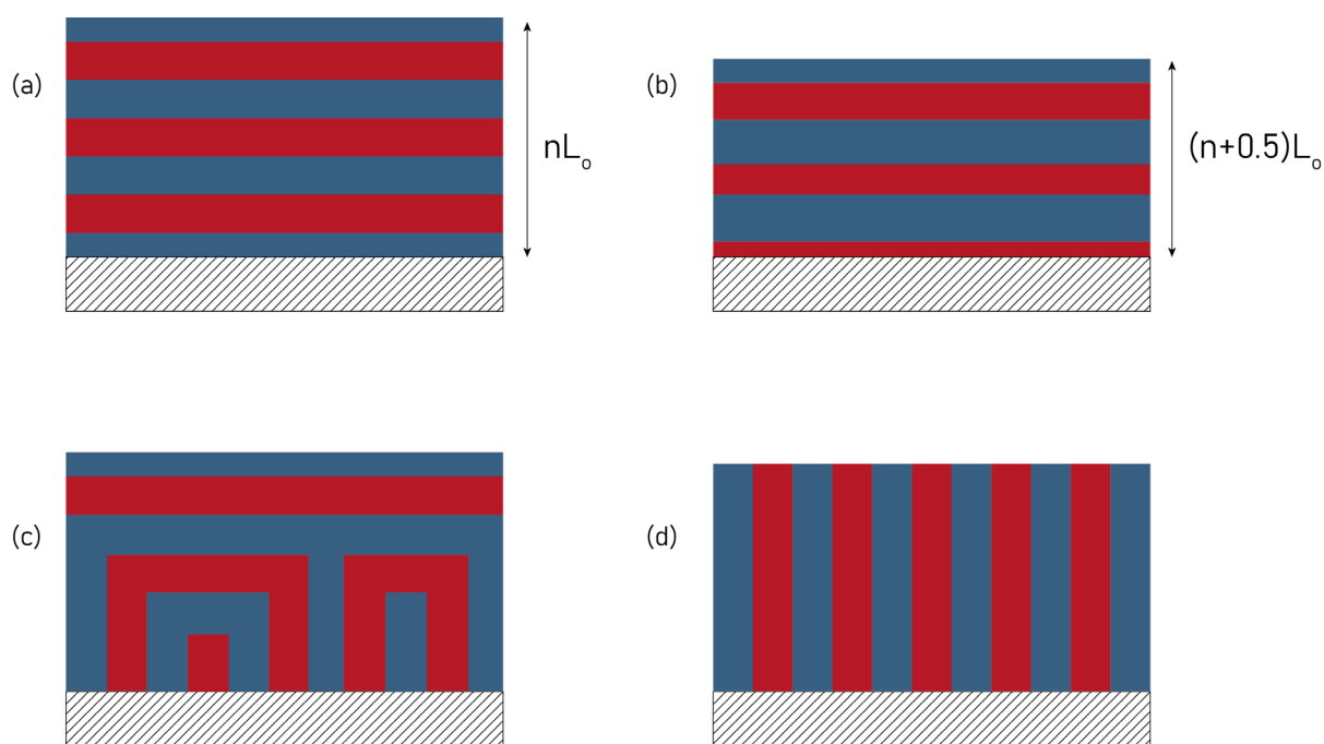
Figure V-2 Orientation of the BCP domains regarding the commensurability of L_0 with the film thickness and the affinity of the blocks for the interfaces. (a) symmetric wetting, (b) asymmetric wetting, (c) neutral wetting with blue block preferentiality for the air surface, (d) neutral wetting.
