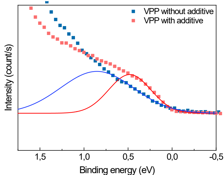
Figure IV-7 Gaussian fits of the valence band tail showing the broadening of the DoS tail around the Fermi level.
