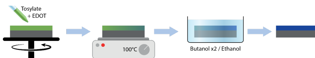
Figure II-1 Scheme of in-situ polymerization. Deposition of the solution of monomers with oxidants and additives, thermal activation of the polymerization, removing of the excess of products by rinsing steps.
