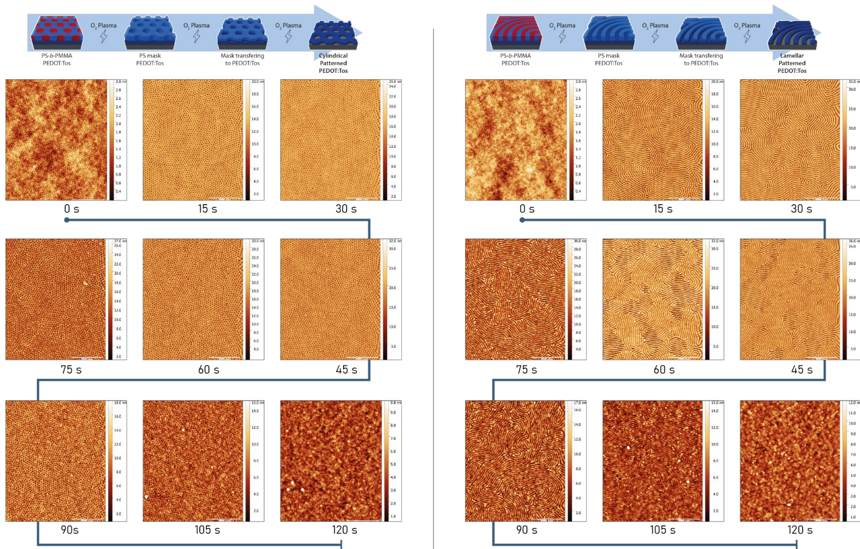
Figure V-9 Topographical AFM image 2 \times 2 \mu m^2 of PEDOT:Tos /PS-b-PMMA films after several O_2 plasma exposure for cylindrical and lamellar morphologies.
