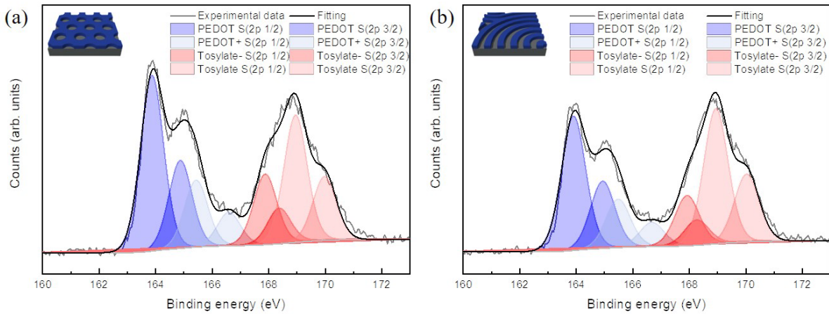
Figure V-6 XPS S 2p spectra of patterned PEDOT:Tos film with (a) cylindrical BCP and (b) lamellar BCP, under O 2 plasma. Blue and red areas represent the signals linked to S 2p in PEDOT and S 2p in tosylate, respectively.
