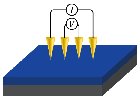
Figure II-3 Scheme of the 4-point probes techniques with characteristic parameters
