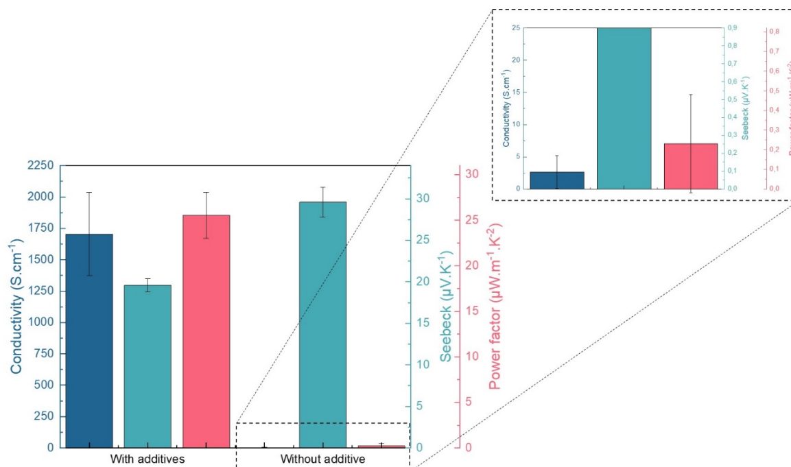
Figure IV-5 Thermoelectric properties of PEDOT:Tos films made by VPP with and without additives. The electrical conductivity, the Seebeck coefficient and the power factor are represented in dark blue, light blue and pink respectively.
