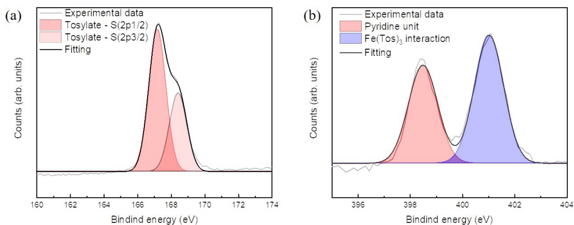
Figure V-20 XPS (a) S2p and (b) N1s spectra of PS- b -P2VP film after incorporation of tosylate
