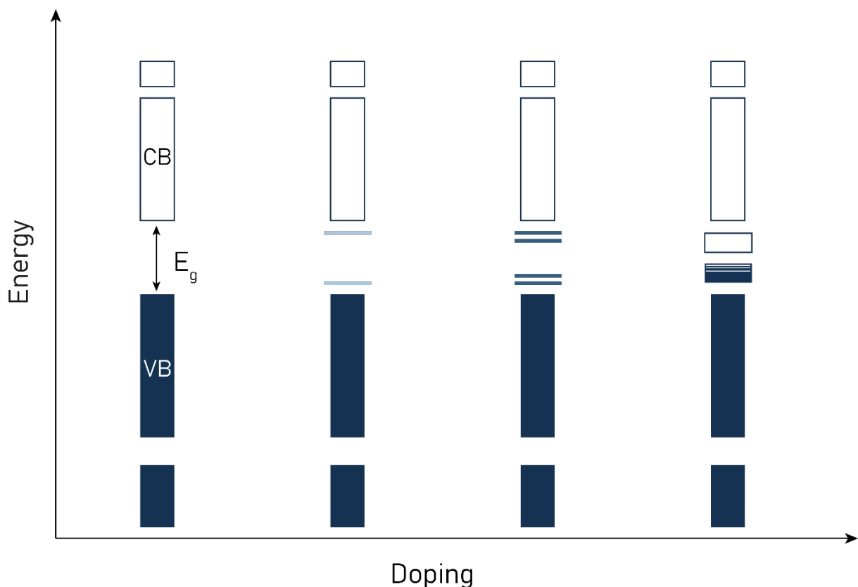
Figure I-11 Formation of localized states in the band gap with doping. At a certain doping, there is the creation of a polaron band. Adapted from [16].
