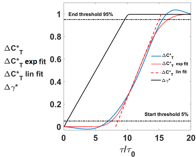
Figure 4.13 – Example of cycle-averaged thrust coefficient history during yaw manoeuvre for configuration HIT2a P2 during a positive yaw variation. Symbols: — \Delta\gamma^* , — \Delta C_T^* , - - - \Delta C_T^* linear, — \Delta C_T^* exp fitted, - - start and end thresholds. Data fitted for \tau > \tau_{lag} .
