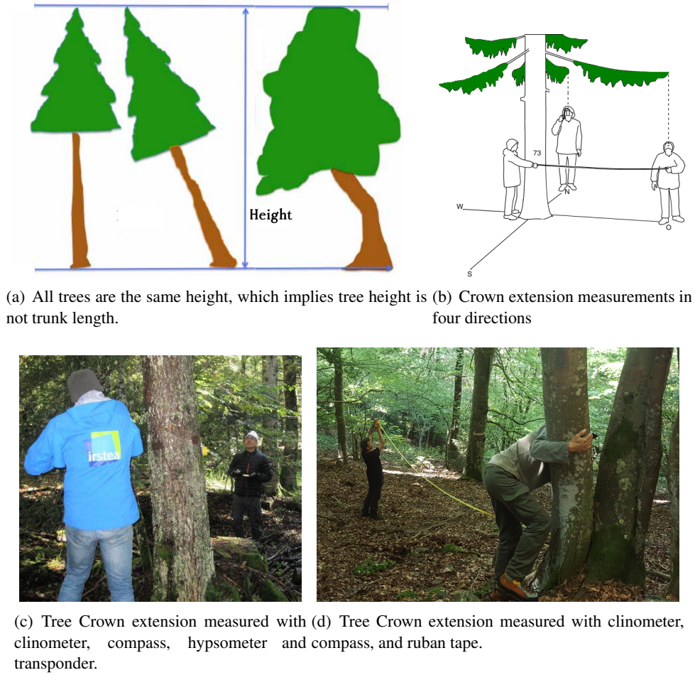
Figure 3.3: Tree height and crown spread measurements generated from the field survey in the site of Chamrousse, France.
