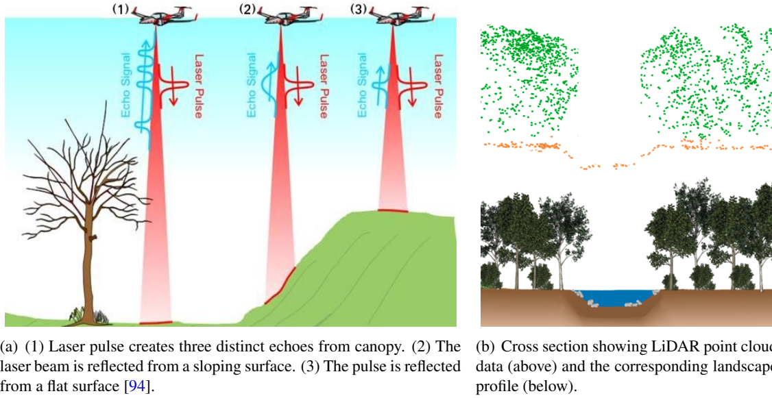
Figure 1.8: (a) LiDAR data acquisition for three scenarios. (b) LiDAR point cloud profile visualization.
