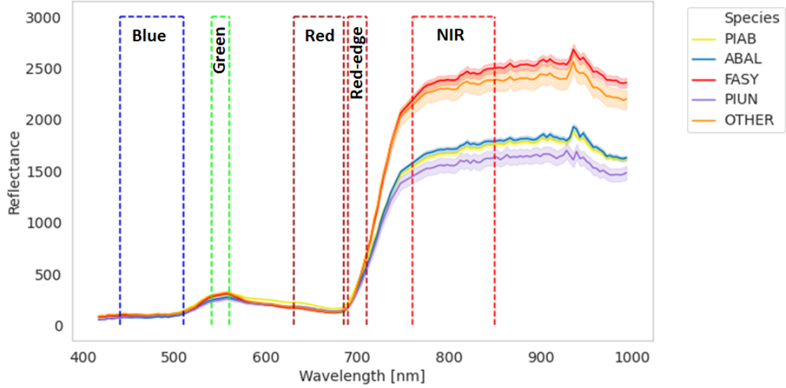
Figure 1.7: Mean spectral signatures of four main species located in the Chamrousse site, in the Northern Alps, France: ● Abies alba (ABAL), ● Fagus sylvatica (FASY), ● Picea abies (PIAB), ● Pinus uncinata (PIUN) and ● “other” species. The spectral bands of blue, green, red, red-edge and NIR are highlighted in their respective ranges.
