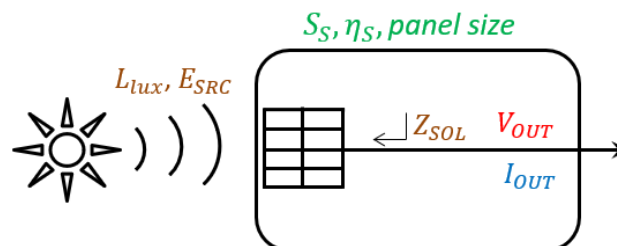
Figure 42 – Solar panel metrics.
