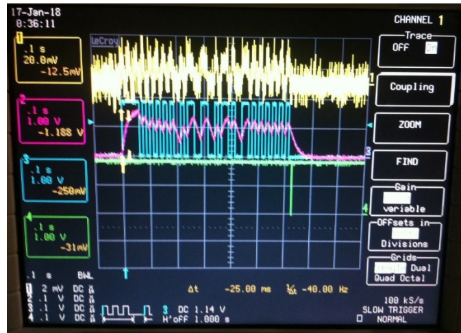
Figure 106 – Example of a signal outputted by the node during a message reception sequence, as captured by the oscilloscope.
