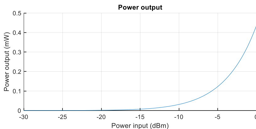
Figure 39 – Power output as a function of RF power input for the 1-stage rectifier.
