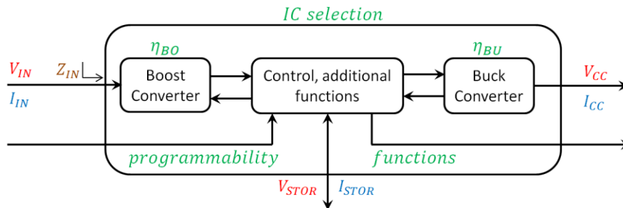
Figure 54 – Power management metrics.
