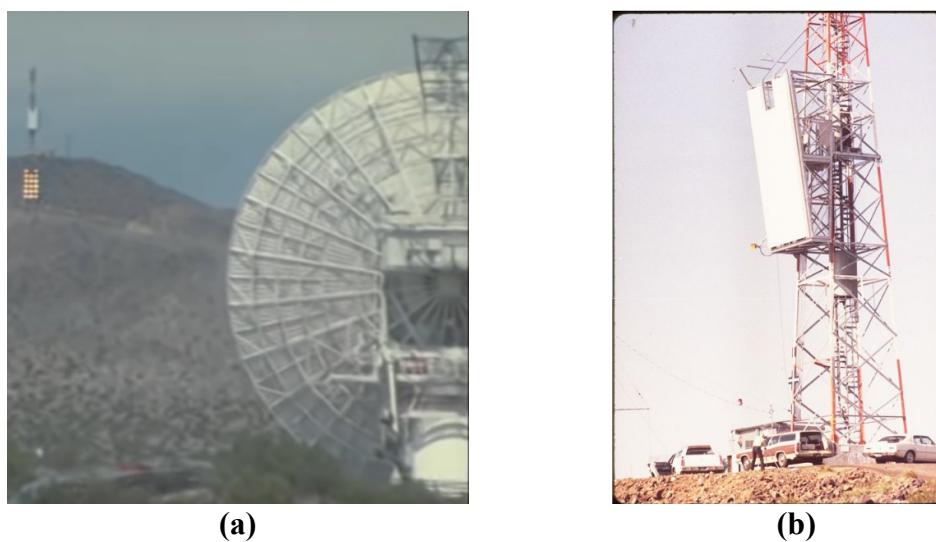
Figure 9 – The NASA JPL experiment at Goldstone. (a) shows the receiver on the far left, and the emitter on the right. (b) is an up-close view of the receiver array [33].
