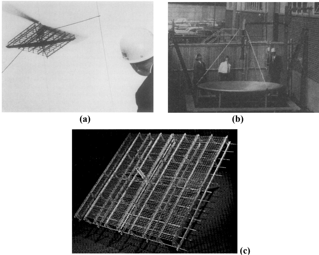
Figure 8 – Wirelessly powered helicopter. (a) shows the helicopter in operation, maintained stable by visible guide rails. (b) is the source, a magnetron emitting at 2450 MHz with 5 kW of power. (c) is the actual rectenna on the helicopter, made of 4480 1N82G point-contact diodes [32].
