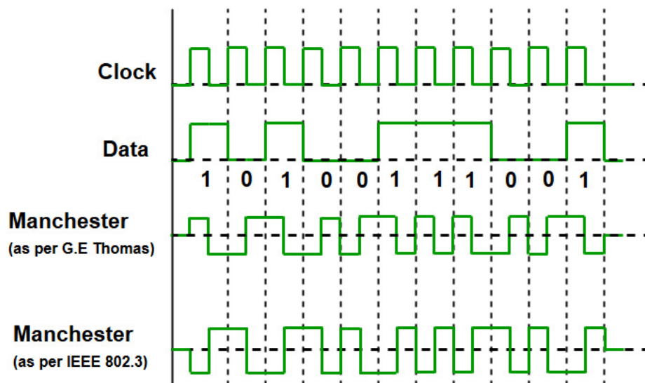
Figure 68 – Manchester encoding, with the two different polarity schemes.
