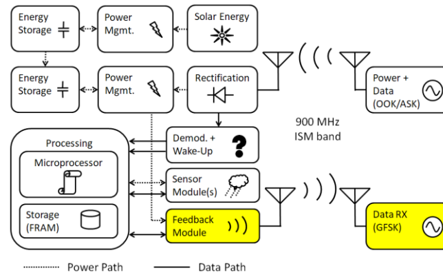
Figure 83 – Position of the data transmission module in the node.
