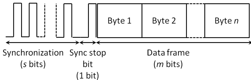
Figure 69 – Data frame format for the node.
