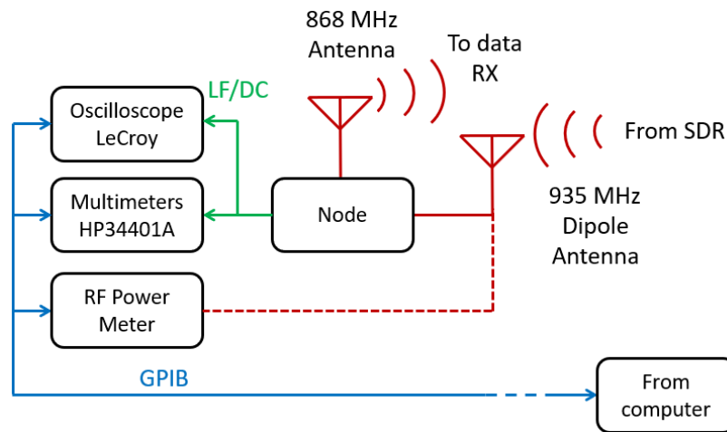
Figure 104 -- Overview of the “back-end” of the node test bench.
