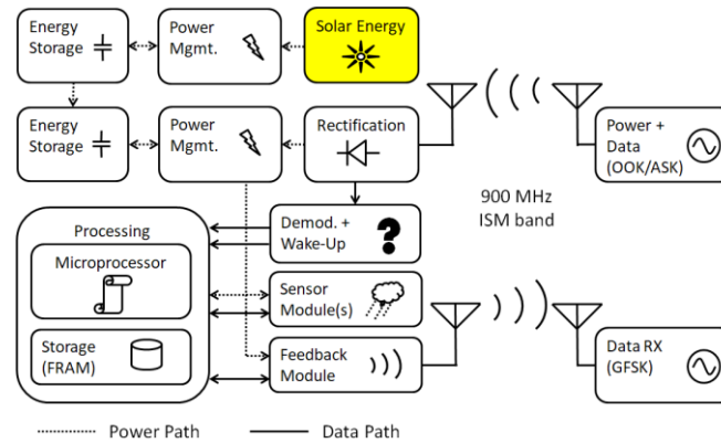
Figure 41 – Position of the solar energy module in the node.
