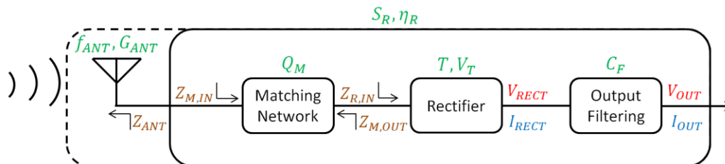
Figure 16 – General rectifier topology for an RF to DC module and associated metrics.
