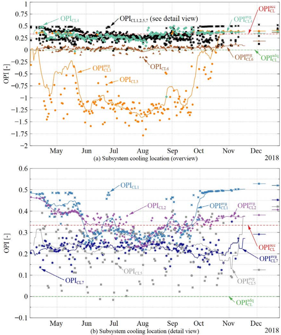
Figure 5.16 – Optimization potential index OPI_{CL} of the subsystem CL in refrigeration machine operation with adequate (green dashed line) and acceptable (red dashed line) boundary: (a) overview and (b) detail view representation. The data points represent the daily OPI values and the solid lines indicate the 14-days moving average of the OPI .
