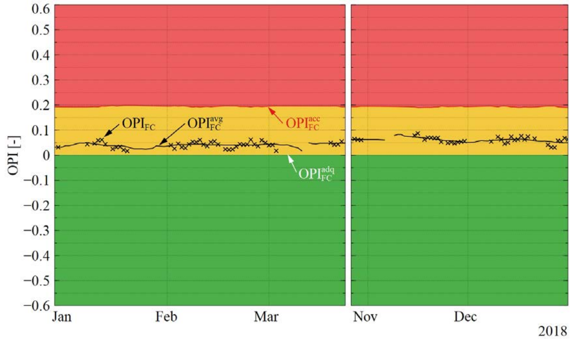
Figure 5.19 – Optimization potential index OPI_{FC} of the subsystem FC (free cooling module) with adequate (green), acceptable (yellow) and inadequate (red) operation range. The data points (black crosses) represent the daily OPI values and the black solid line indicates the 14-days moving average of the OPI .
