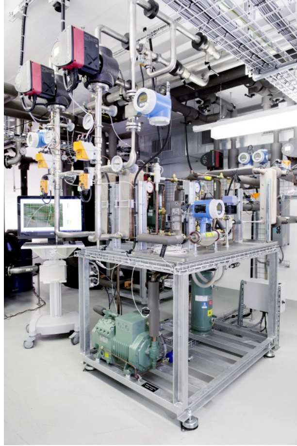
Figure 4.2 – Overview of the R134a refrigeration machine test rig.
