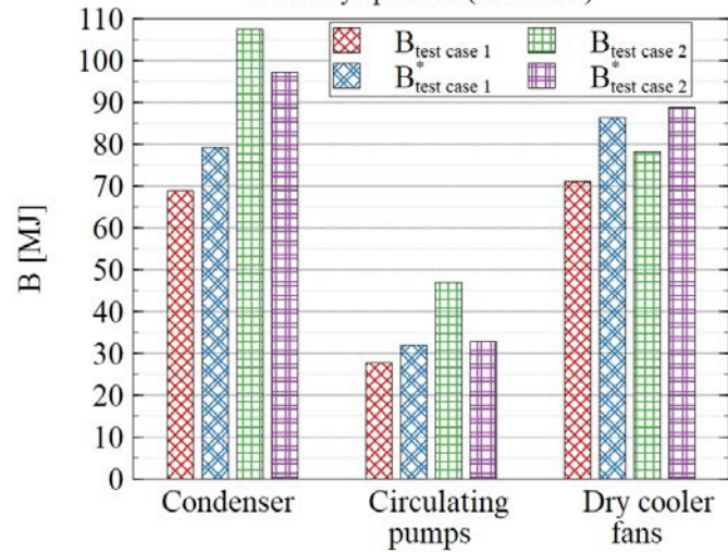
(b) Actual and reference daily exergy sum of the subsystem DC in adequate (test case 1) and faulty operation (test case 2)
