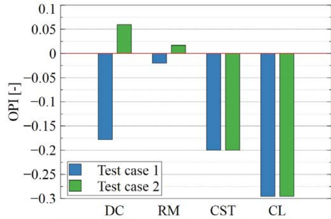
(a) OPI of the different subsystems in adequate (test case 1) and faulty operation (test case 2)
