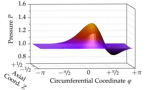
(b) Pressure field ( N_\varphi \times N_Z = 49 \times 7 , N_P = 1 ).
