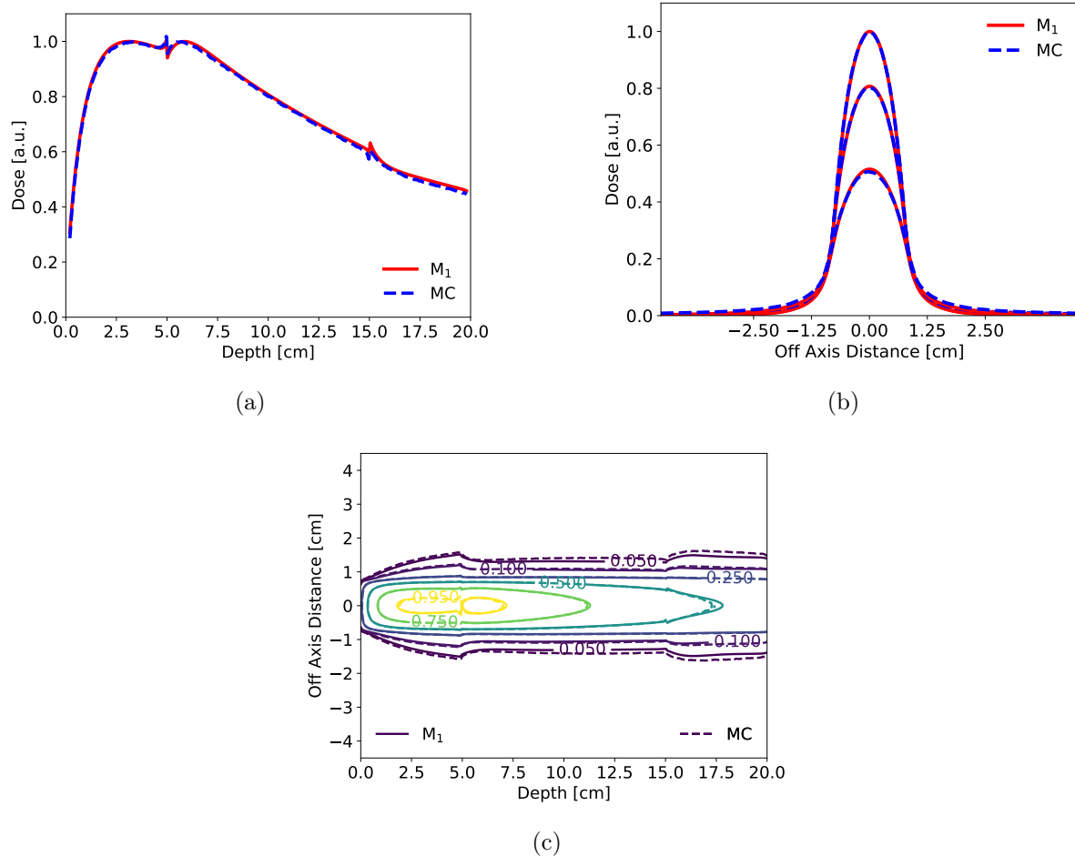
Figure 5.8: 18 MV photon beam coming from the left in a water phantom with a bone insert between 5 cm and 15 cm: (a) depth dose distribution along the central axis, (b) transverse dose profiles at the center of the beam ( z = 0 ) taken at depths of 3.2, 10 and 17 cm and (c) 2D isodose map at z = 0 in the xy plane. In this case the M1 model is slightly less diffusive than the Monte Carlo code. In depth dose profile our model reproduces the second build-up after the first interface in bone but overestimates the discontinuity at the second interface.
