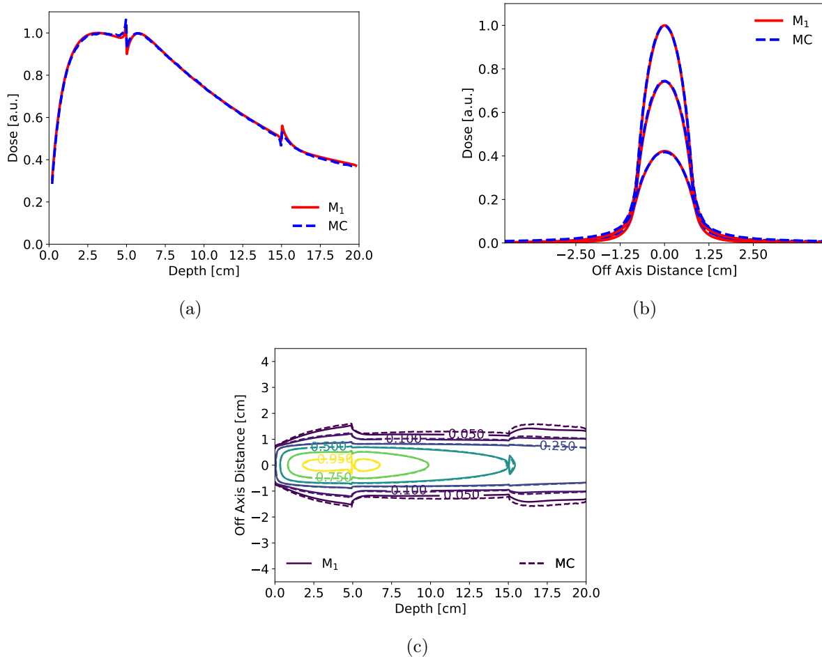
Figure 5.13: 18 MV photon beam coming from the left in a water phantom with a aluminium insert between 5 cm and 15 cm: (a) depth dose distribution along the central axis, (b) transverse dose profiles at the center of the beam ( z = 0 ) taken at depths of 3.2, 10 and 17 cm and (c) 2D isodose map at z = 0 in the xy plane.
