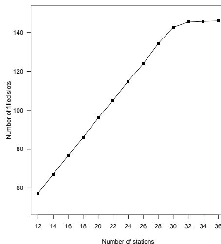
Figure 4.17: Average ring occupancy versus number of stations.
