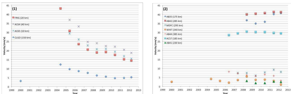
Figure 67 : Time evolution of 2-year GPS horizontal velocity. (1) Selection of permanent stations within 150 km of the Denali 2002 earthquake rupture. (2) Selection of permanent stations farther than 150 km from the Denali 2002 earthquake rupture.
