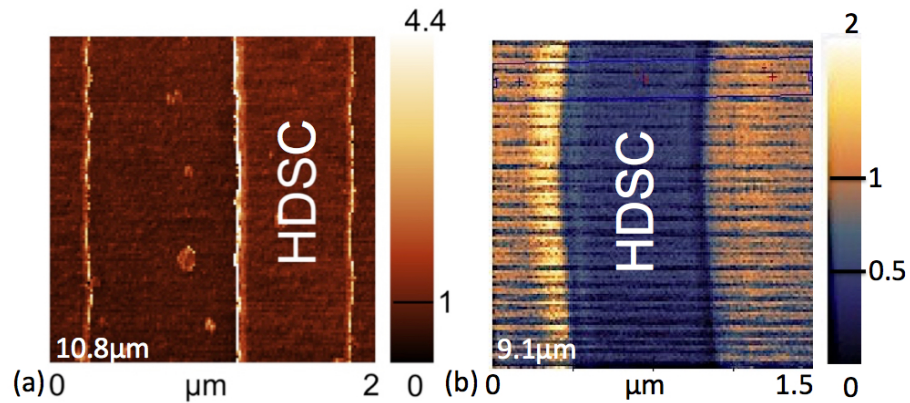
Figure 4.2.9.: PiFM image with modified laser system: (a) PiFM image with horizontal system at 10.8 μm (modified CW mode QCL ranging from 10.4 μm to 11.51 μm); (b) PiFM image with vertical system at 9.1 μm (modified CW mode QCL ranging from 9.05 μm to 9.69 μm).
