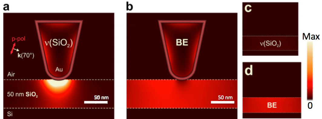
Figure 1.1.10.: Simulation with RSoft: (a) tip induced absorption at \nu(SiO_2) ; (b) BE absorption in a 50 nm SiO_2 film on Si under p-polarized illumination at 70^\circ ; Corresponding simulations without the tip are shown in (c) and (d), respectively. Adapted from[49].
