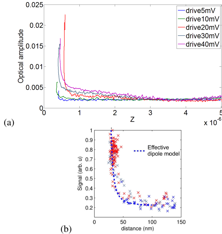
Figure 4.2.4.: Approach curve of s-SNOM: (a) Approach curve of s-SNOM at different probe oscillation amplitude, taken at 11 \mu\text{m} with probe above HDSC gratings; (b) Reconstructed approach curve on polymer/gold grating, adapted from [178].
