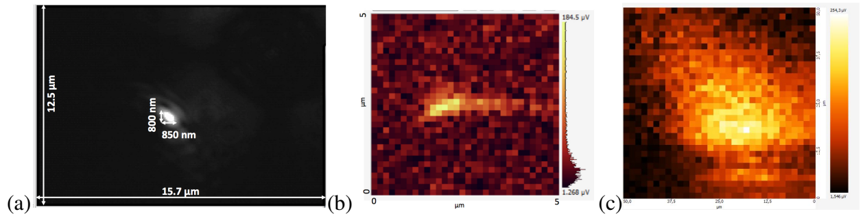
Figure 4.2.15.: Laser spot imaging in reflection mode: (a) camera view of the focused spot by parabolic mirror (633 nm); (b) PiFM image (633 nm); (c) PiFM image (5780 nm, image from MolecularVista).
