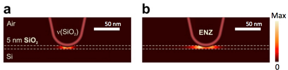
Figure 1.1.11.: Simulation with RSoft: (a) tip induced absorption at \nu(SiO_2) ; (b) ENZ absorption in a 5 nm SiO_2 film on Si under p-polarized illumination at 70^\circ . Adapted from[49].
