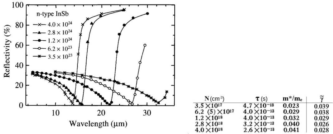
Figure 1.1.2.: Example of plasma edges measured on n-doped III-V semiconductor. The spectra can be correctly fitted using the Drude model parameters on the right table. The electron density is in \text{cm}^{-3} in the table, the other values are in USI. Adapted from[39].
