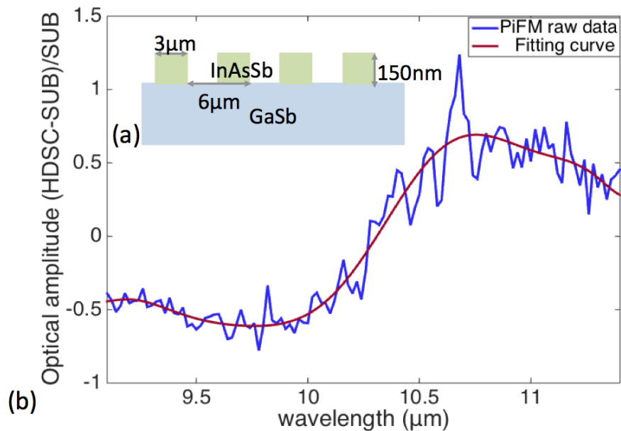
Figure 5.1.6.: HDSC Gratings with lower plasma frequency (corresponding wavelength 9.4 \mu\text{m} ): (a) Scheme of sample; (b) Optical amplitude spectrum: blue curve is raw experimental data and red curve is a fitting curve showing the form of the raw data.
