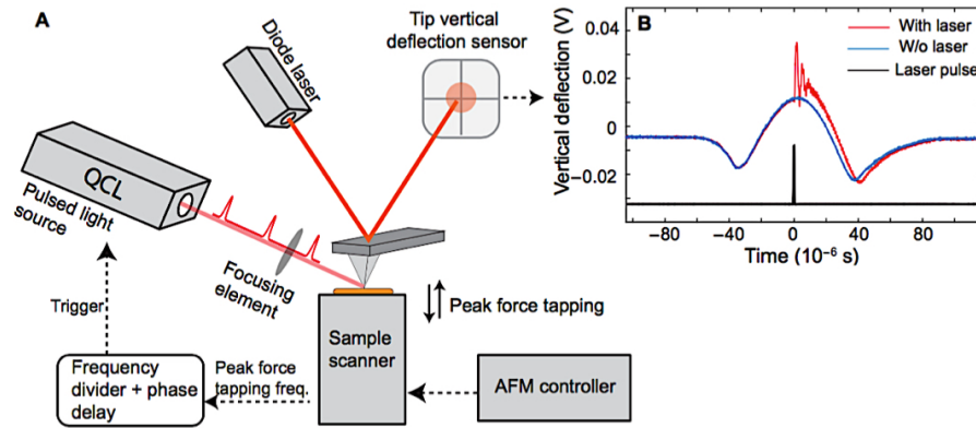
Figure 3.2.2.: Operational scheme of PFIR microscopy: (A) Operation diagram of PFIR; (B) Gate-averaged traces of vertical deflections of the cantilever with the laser interaction (red curve) and without the laser interaction (blue curve). The timing of the infrared laser pulse (black curve) is chosen to be within the contact regime of the peak force tapping cycle. Subtraction of the two vertical deflection traces (red and blue, with and without laser respectively) is used to obtain the PFIR trace. From[27].
