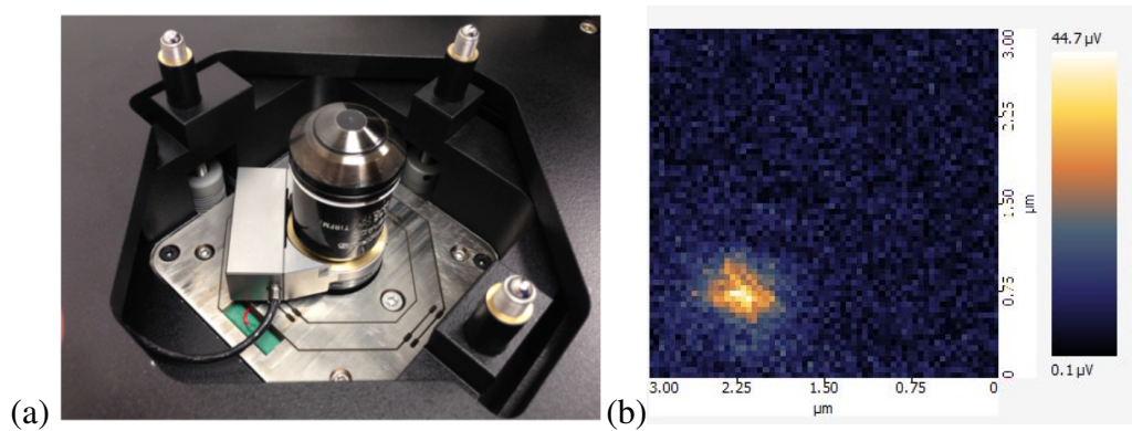
Figure 4.2.11.: Visible PiFM with objective scan: (a) inverted objective lens with 3D scanning stage; (b) laser spot imaging with PiFM.
