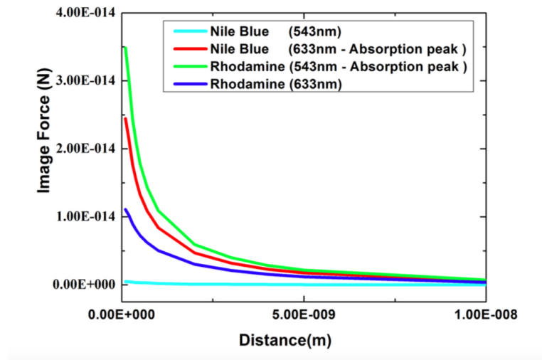
Figure 3.3.1.: Simulation of force vs distance relationship of photo-induced force, from[158].
