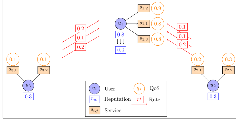
Figure 3.1: Example of Bad-Mouthing Attack.
