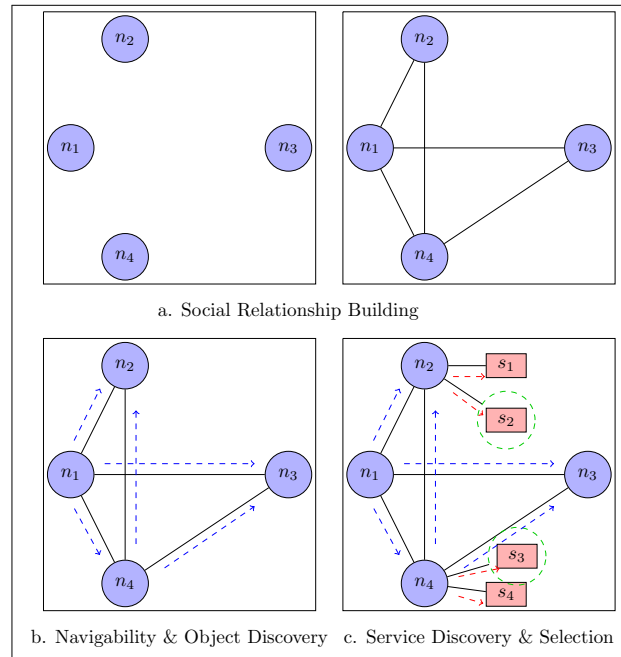
Figure 1.7: Service Discovery in SIoT.
