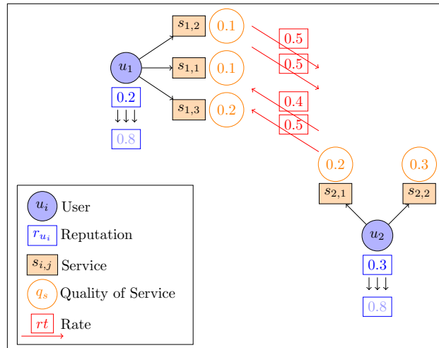
Figure 3.2: Example of Ballot-Stuffing Attack.
