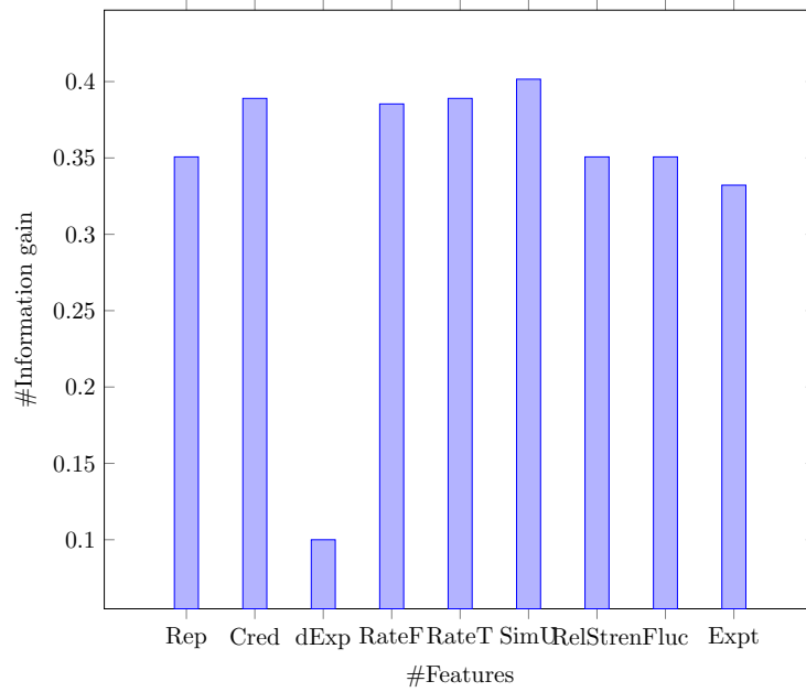
Figure 5.1: Information gain for single feature performance.
