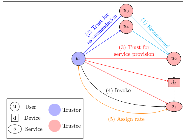
Figure 2.4: Example of interaction scheme.
