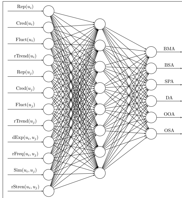
Figure 4.3: Deep-Learning Model for Type-Attack detection.
