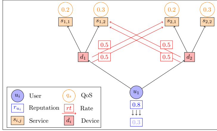
Figure 3.3: Example of Self-Promoting Attack.
