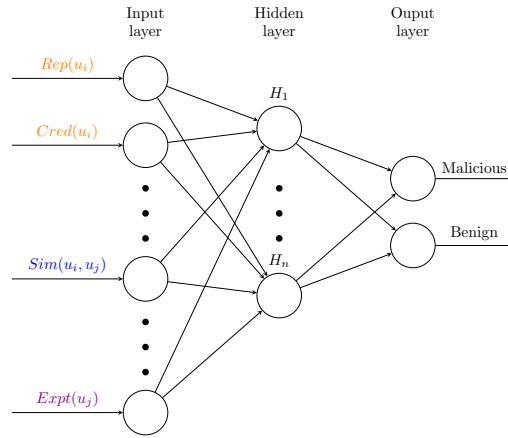
Figure 4.1: Trust-Aggregation based on Machine Learning.
