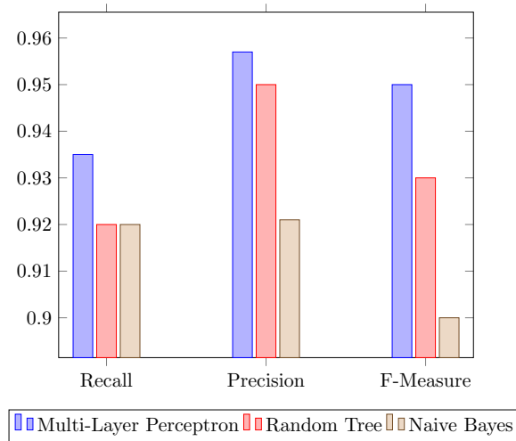
Figure 4.2: Classification results obtained with machine-learning algorithms trained with the proposed features.
