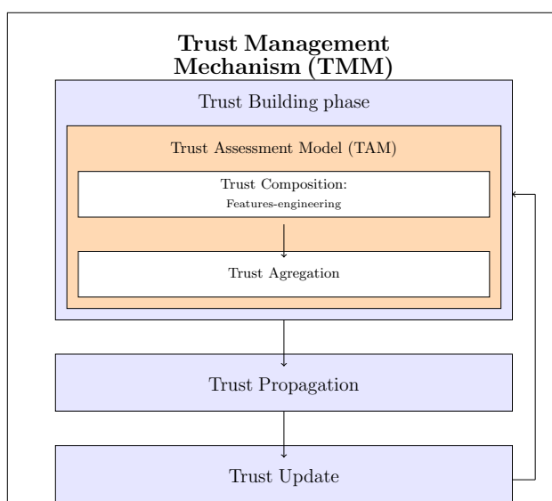
Figure 2.2: Trust-Management process
