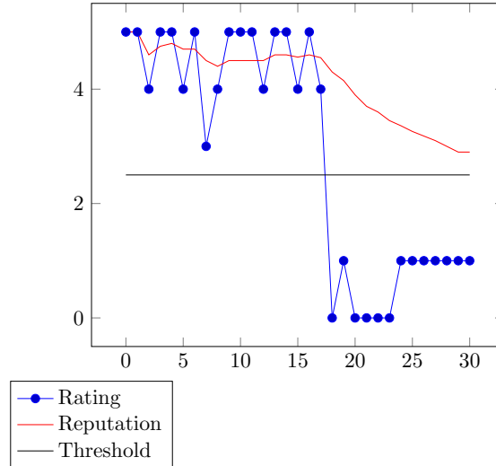
Figure 3.6: Example of Opportunistic Service Attack.
