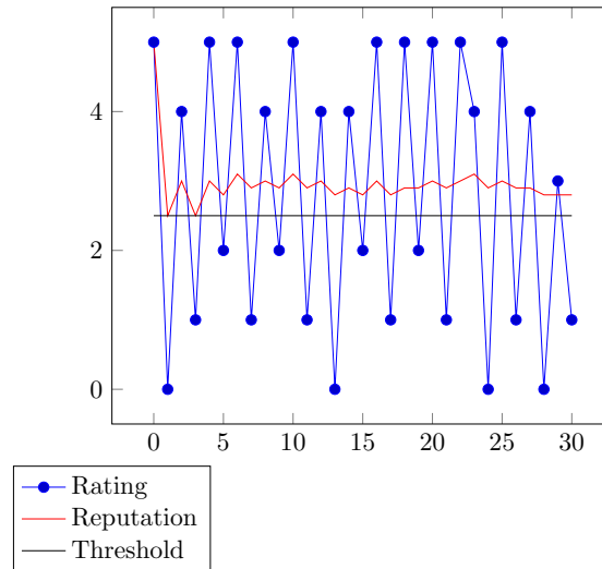
Figure 3.5: Example of On-Off Attack.
