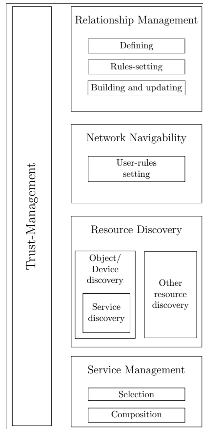
Figure 1.6: SIoT Architecture.
