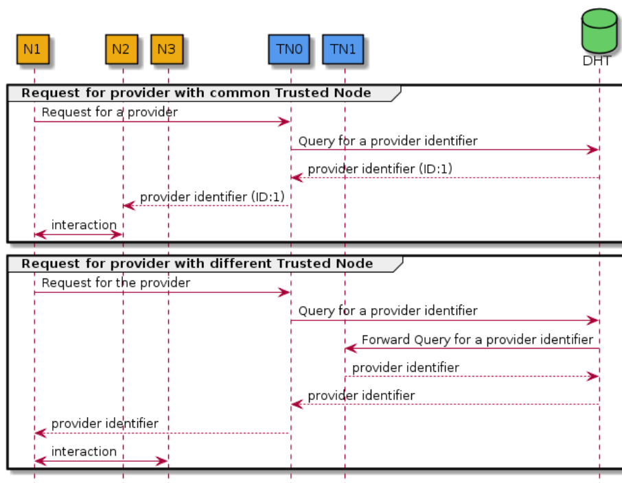
Figure 4.7: Sequence diagram of Hybrid propagation based on Distributed Hash Table.
