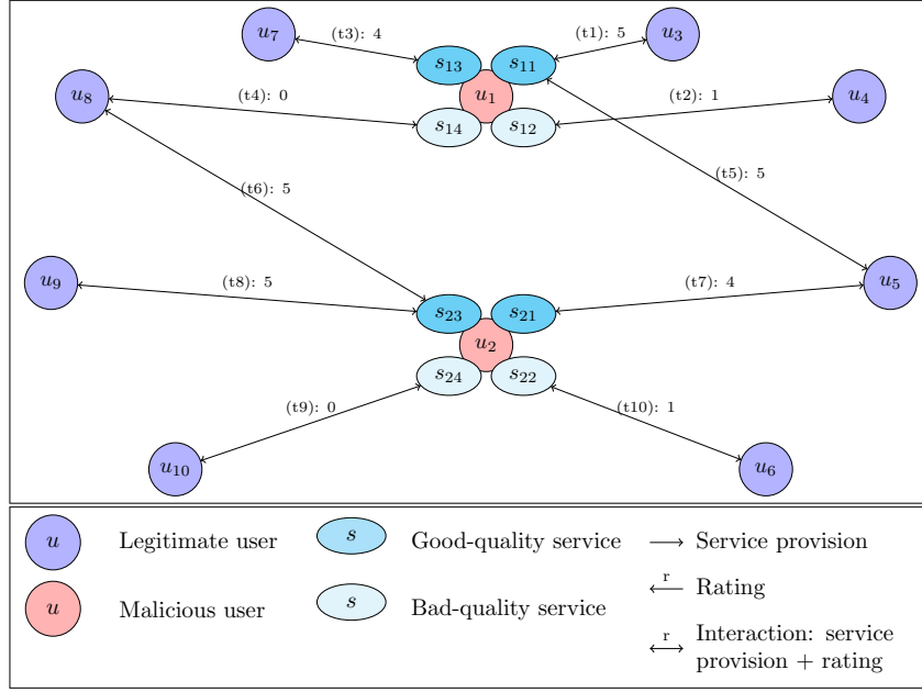
Figure 4.5: Malicious Provider Attacks Countering.
