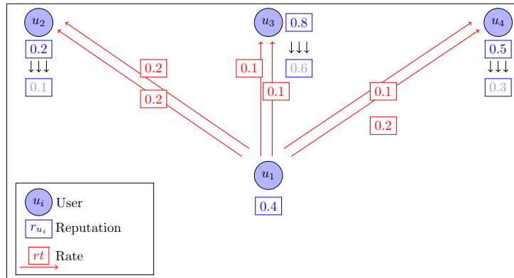
Figure 3.4: Example of Discriminatory Attack.
