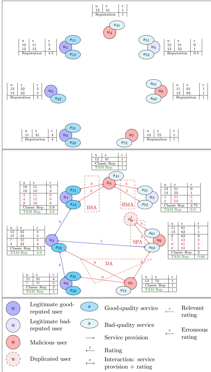
Figure 4.4: Malicious Recommender Attacks Countering.
