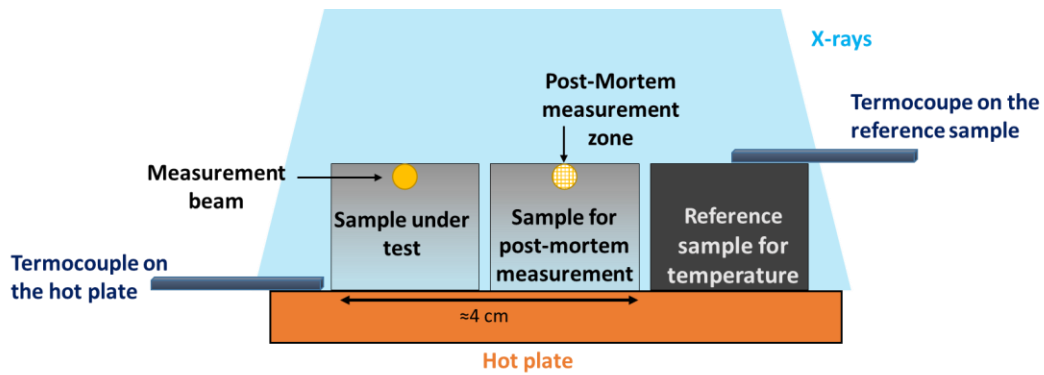
Fig. 112: Irradiation set-up to measure the influence of optical bleaching on the RIA, view at the exit faces of the samples.
