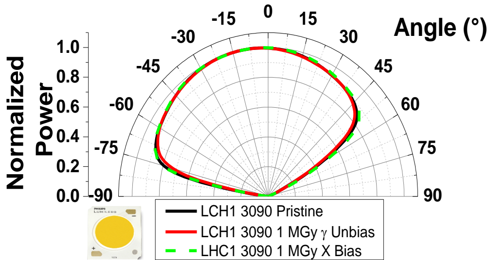
Fig. 46: Angular luminous intensity of the LCH1 3090 LED before and after irradiation in several conditions and a picture of the LED. Here the “Pristine” is an average of the measurement of the 3 LEDs before irradiation.
