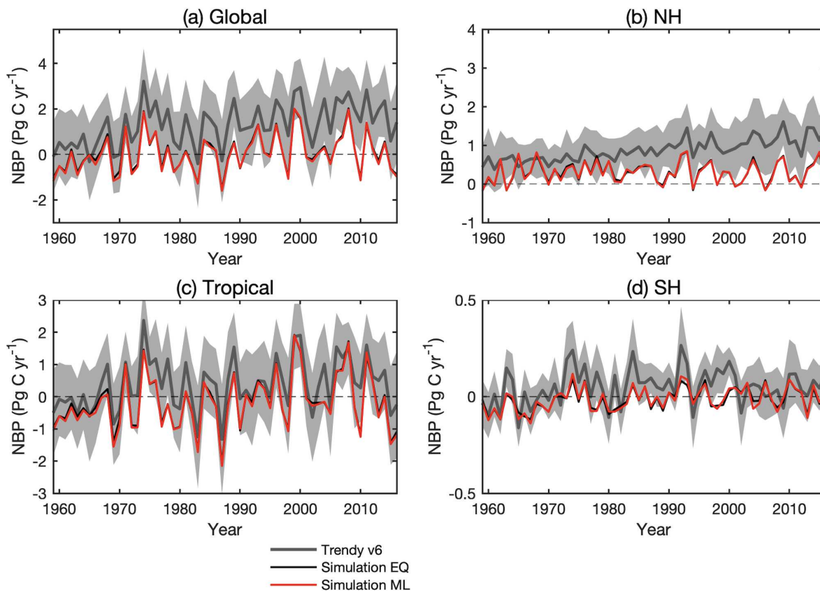
Figure S4.15 Changes in total yearly net biome productivity (NBP) during 1959-2016 from Simulation EQ and two Simulation ML and Trendy v6 model for global (a), North Hemisphere (NH; 30oN - 90oN; b), Tropical (30oS - 30oN; c), and South Hemisphere (SH; 30oS - 90oS; d). Grey shading indicates \pm 1\sigma uncertainty of DGVM results for Trendy v6.
