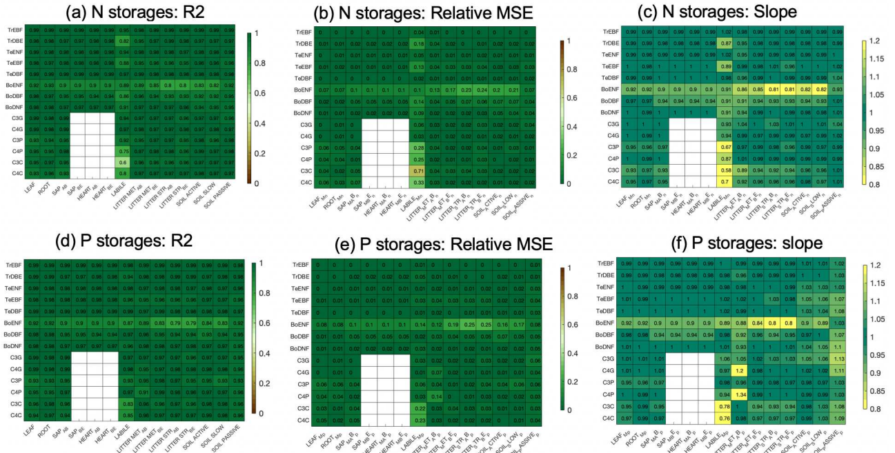
Figure S4.18 Performances of machine learning models (ML)-based historical simulation (i.e. Simulation ML) on mean N and P storages across 2000-2010, compared to Simulation EQ. The statistics are the same with Figure 3-5.
