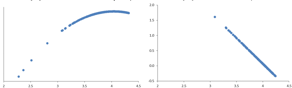
Figure A - IV.3: The estimated relationship between PS and CO2 [DMG approach] (3a) the estimated relationship CO2/PS (3b) the derivative dCO_2/dPS
