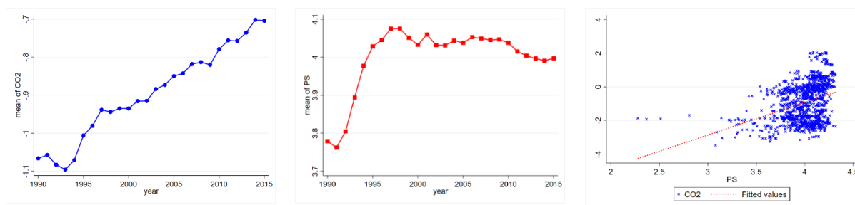
Figure IV.2: CO2 and PS evolution over time and scatterplot [full sample]
