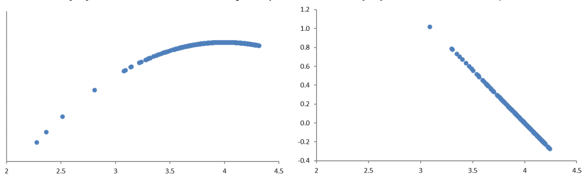
Figure A - IV.1: The estimated relationship between PS and CO2 [CS-ARDL-PMG approach] (1a) the estimated relationship CO2/PS (1b) the derivative dCO_2/dPS
