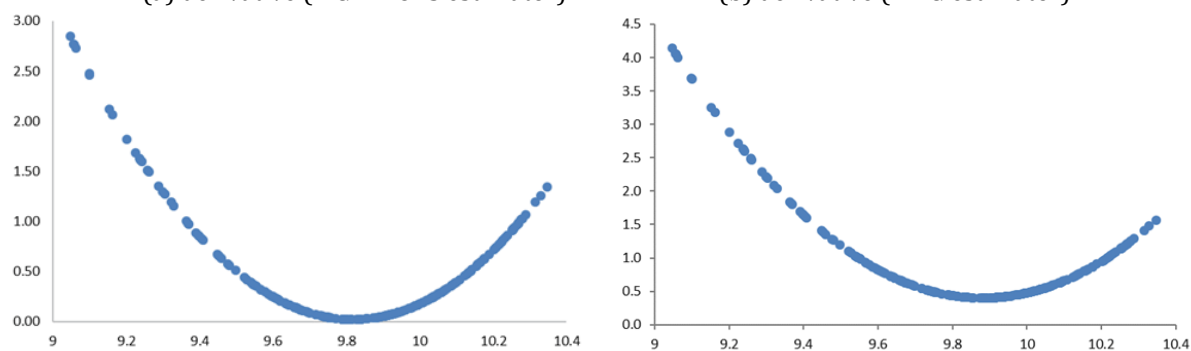
Figure II.5: The estimated relationship between GDP and CO2 [aggregated analysis: robustness] (a) derivative (MG-FMOLS estimator) (b) derivative (AMG estimator)
