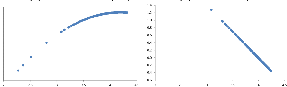
Figure A - IV.2: The estimated relationship between PS and CO2 [AMG approach] (2a) the estimated relationship CO2/PS (2b) the derivative dCO_2/dPS
