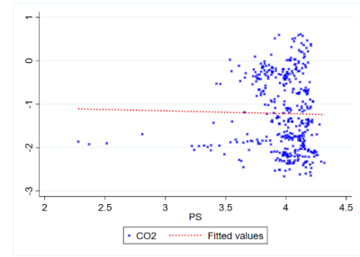
(c) CO2 versus PS
