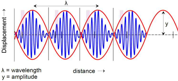
Fig. 1.2.d. Representations of wave packets (wave trains) with a direction of propagation to the right. In this figure, the wave envelope is represented in red. Adapted from Fig. 1.2.c. Source: Etienne Bonnet
