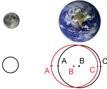
Fig. 1.9.4.3.a. Illustration of the Earth-Moon system and the sketch of the positions of the Earth and the Moon. The red circle represents the greatly exaggerated effects of gravity we could expect because of the gravitational gradient. Source: Etienne Bonniec.
