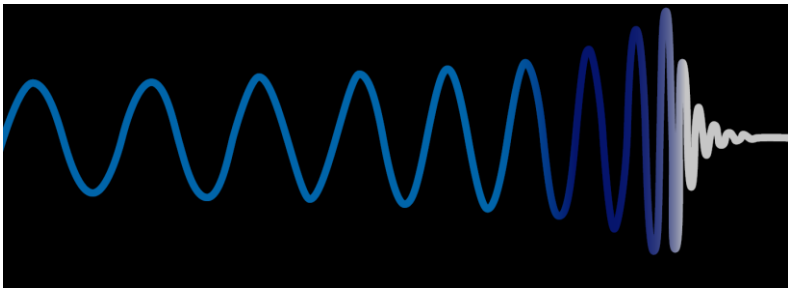
Fig. 1.9.3.a. Illustration of the “chirp” signal given by a binary black hole merger. Source: Etienne Bonniec.
