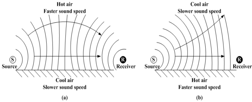
Fig. 1.6.2.e. Illustration of the bending of soundwaves happening due to a gradient in temperature in the air. Source: Etienne Bonniec.
