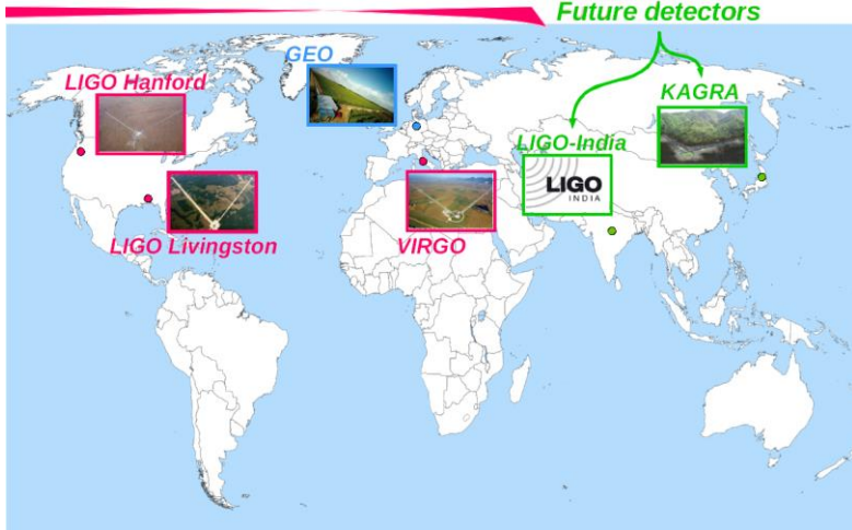
Fig. 5.2. Map of the gravitational waves detectors network. Source: Courtesy of Julia Casanueva.
