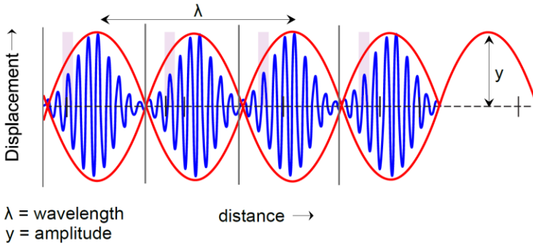
Fig. 1.2.d. Representations of wave packets (wave trains) with a direction of propagation to the right. In this figure, the wave envelope is represented in red. Adapted from Fig. 1.2.c. Source: Etienne Bonnet
