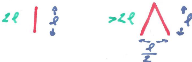
Fig. 3.2.1.1.c. In this drawing, the path of our photon, in red, as seen by the experimenter ( left ) and as seen by our observer ( right ). Source: PV, handmade.
