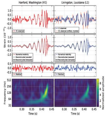
FIG. 3. The gravitational-wave event GW150914 observed by the LIGO Hanford (H1, left column panels) and Livingston (L1, right column panels) detectors. Time is shown relative to September 14, 2015 at 09:50:45 UTC. For visualization, all time series are filtered with a 35–350 Hz bandpass filter to suppress large fluctuations outside the detectors’ most sensitive frequency band, and band-pass filters to remove the strong instrument spectral lines seen in Fig. 3 spectra. Top row, left–H1 strain. Top row, right–L1 strain. GW150914 arrived first at L1 and 6.92 ms later at H1, for a total separation. The H1 data are also shown, shifted in time by this amount and inverted to account for the detectors’ relative orientations. Second row–Gravitational-wave strain projected onto each detector in the 35–350 Hz band. Solid lines show numerical relativity waveforms for a system with parameters consistent with those recovered from GW150914 [37–39], conditioned to 99.9% by an independent calculation based on [15]. Shaded areas show 90% credible regions for two independent waveform reconstructions. Our (black gray) model fits the signal using binary black hole template waveforms [19]. The other (light gray) lines are not an astrophysical model, but instead calculate the strain signal as a linear combination of zero-Gaussian modes [40, 41]. These reconstructions have a 94% overlap, as shown in [35]. Third row–Residuals after subtracting the filtered numerical relativity waveform from the filtered detector time series. Bottom row–A time-frequency representation [42] of the strain data, showing the signal frequency increasing over time.
