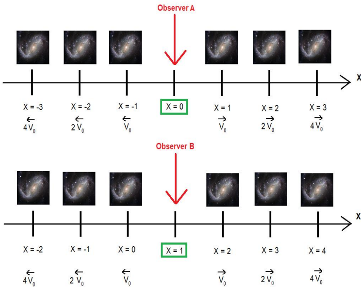
Fig 5.3.h. Illustration of the expansion of the Universe from the point of view of observers located in different galaxies. Source: PV, MS Paint.
