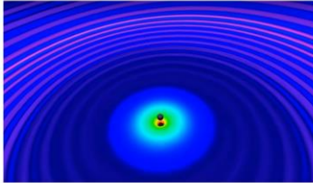
Source: Screenshot of the SXS (Simulating eXtreme Spacetimes) https://www.black-holes.org/ Computer Simulation "You fall into the GW150914 black hole - black hole merger" https://www.youtube.com/watch?v=dyP35HJRHk8&list=PQ9taJkE
