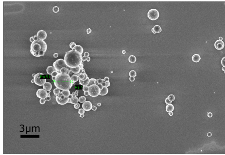
Figure 5.2: Scanning electron microscopy image of iron micro-spheres laying on a coverslip.
