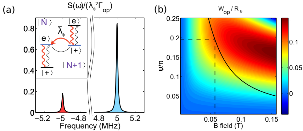
Figure 4.14: a) Spin excitation spectrum showing the emission ( \omega < 0 ) or absorption ( \omega > 0 ) of phonons under resonant conditions \omega_{e'} - \omega_{+} = \omega_{\phi} . The inset shows the cooling mechanism as a cascade between the dressed states from librational phonon numbers N + 1 to N . The parameters are: B = 2.6 mT, \Omega_R/(2\pi) = 0.5 MHz, \Delta/(2\pi) = 3 MHz and \Gamma_{\text{op}} = 10 kHz. b) Normalized cooling rate as a function of the B -field and \Psi/\pi for \Gamma_{\text{op}} = 100 kHz and \omega_{\phi}/(2\pi) = 5 MHz. The black line is the \psi parameter under the resonance condition as a function of the B -field for \Omega_R/(2\pi) = 1 GHz.
