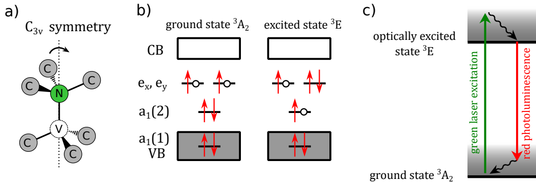
Figure 3.1: a) NV center embedded in a diamond crystal, with a C_{3v} symmetry around the NV axis. N: nitrogen, C: carbon, V: vacancy. b) Detailed electronic structure of the NV^- center, the molecular orbitals are named after their symmetry. VB: Valance Band, CB: Conduction Band. c) Orbital ground and excited states of the NV^- center. Excitation is typically done at 532 nm in the phonon band (grey gradient) while the photoluminescence spectrum is mostly in the red, following phonon emission (wavy arrow).
