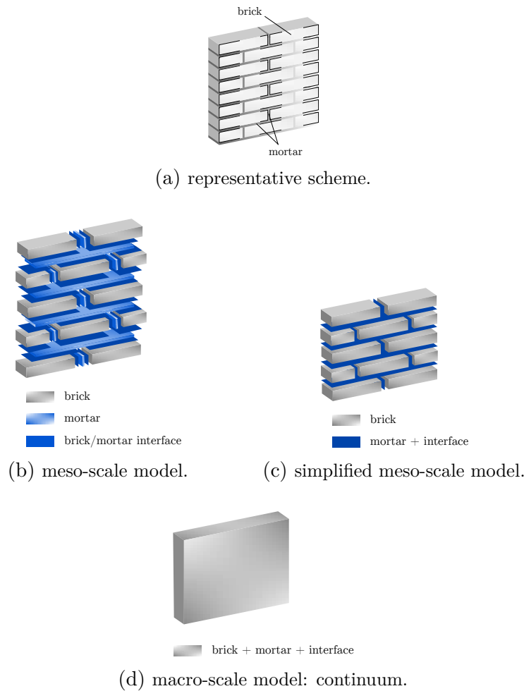
Figure 2.26 – Modeling approaches for masonry according to a meso-scale description, (b) and (c), and a macro-scale one (d).
