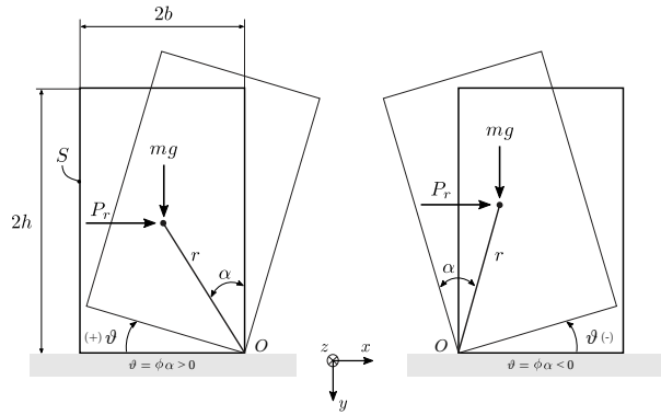
Figure 3.1 – Configuration considered for the rocking problem: a rectangular slender, rigid block resting on a horizontal plane with uniformly distributed mass, subjected to uniform pressure load due to an explosion.
