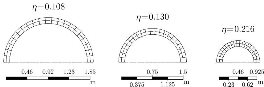
Figure 4.9 – Configurations for different slenderness ratios, \eta .
