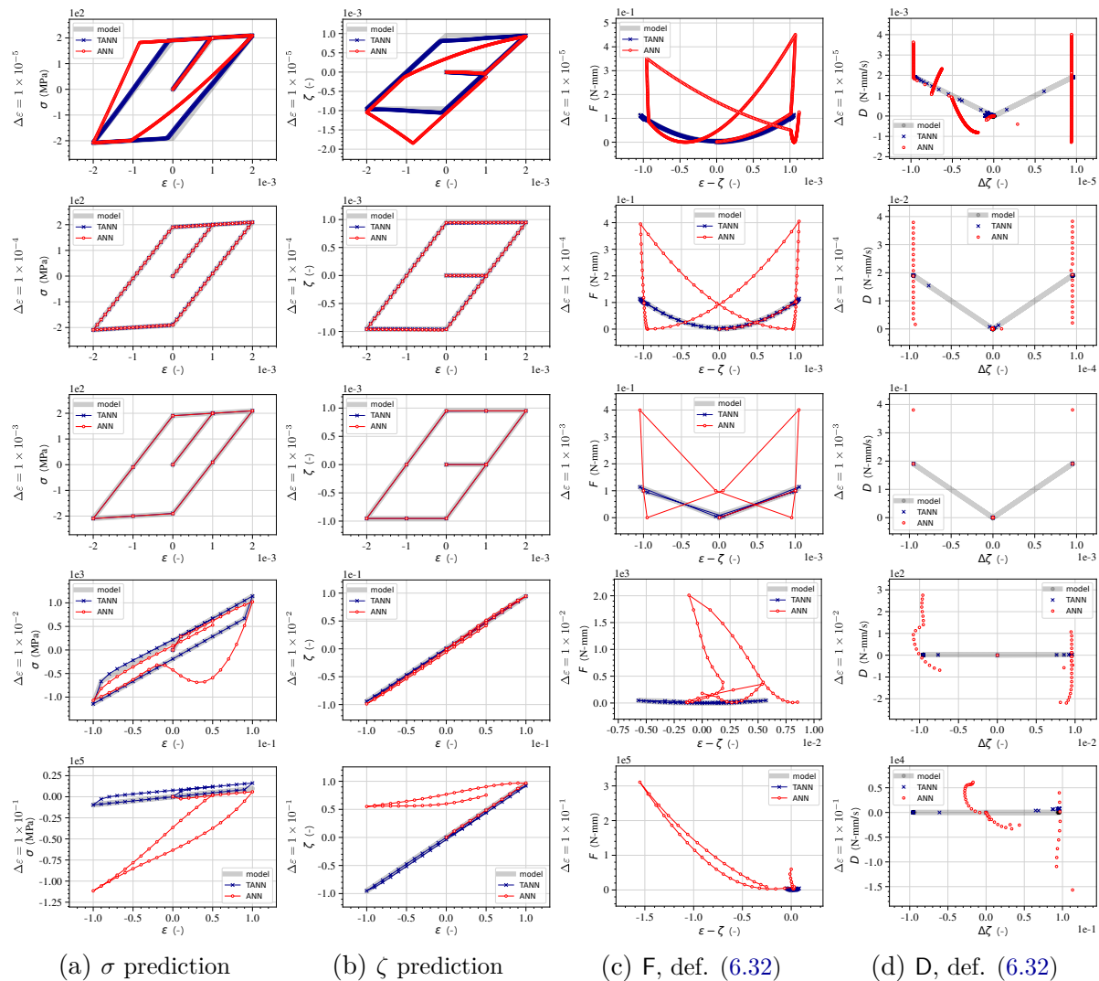
Figure 6.17 – Comparison of the predictions of TANN and those of standard ANN, for material case 1D-B (hardening). Each row represents the prediction at different \Delta\varepsilon .
