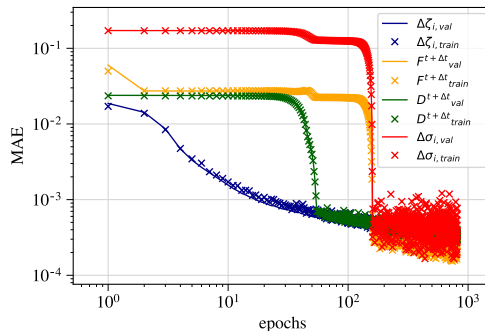
Figure 6.20 – Errors of the predictions of TANN (loss functions), as the training is being performed, evaluated with respect to the training (train) and validation (val) sets. Weights and biases update is computed only on the training set.
