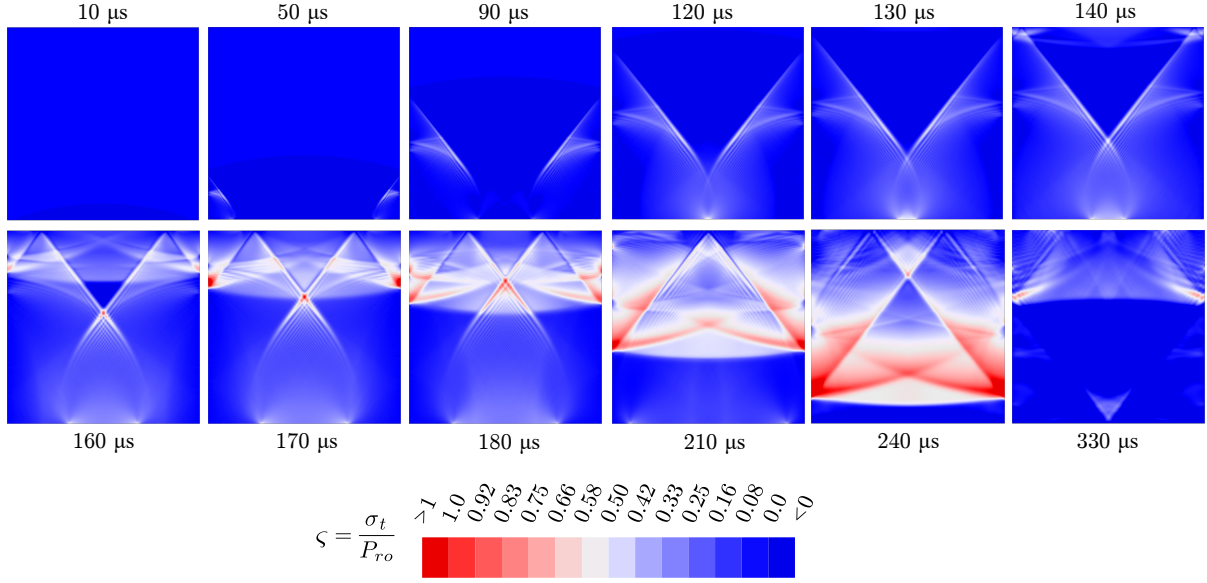
Figure 3.15 – Time evolution of the dimensionless stress \zeta = \sigma_t/P_{ro} through the cross-section A = 0.5 \times 0.5 \text{ m}^2 of a target due to an explosion ( R = 1 \text{ m} , W = 20 \text{ kg} ). The time origin is at the shock wave arrival on the free bottom boundary. The initial longitudinal wave is refracted at the free boundaries. The released waves interact continuously and cause stress concentrations. The material is assumed to be linear elastic.
