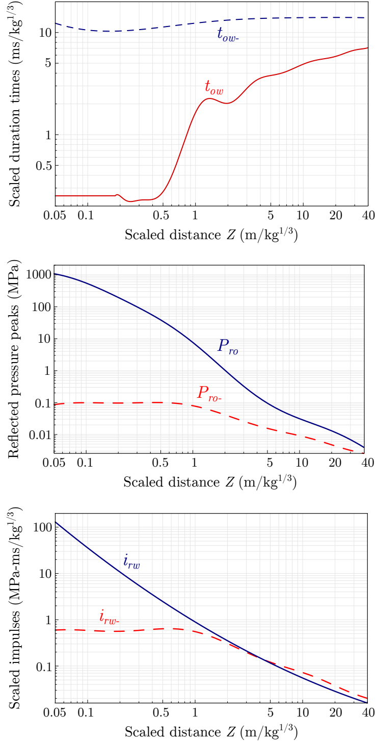
Figure A.1 – Analytical interpolations for blast loading: scaled duration times (top), reflected pressure (center) and impulses (bottom) as functions of the scaled distance, Z .
