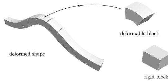
Figure C.2 – Out-of-plane deformation mode of blocky structure, modeled with deformable blocks (left). Block bending modes (right) with deformable (top) and rigid (bottom) blocks.
