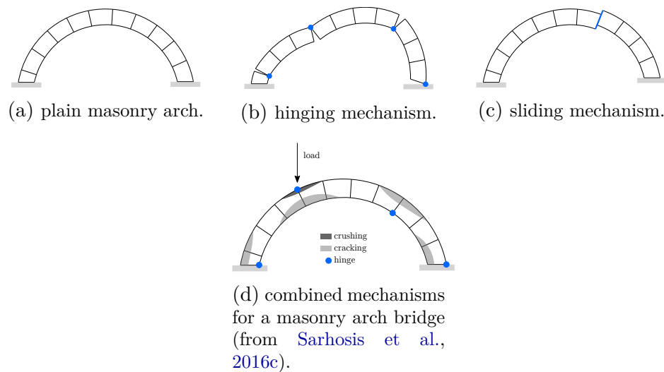
Figure 2.12 – Some typical structural failure mechanisms in plain arches under vertical loading and self-weight.
