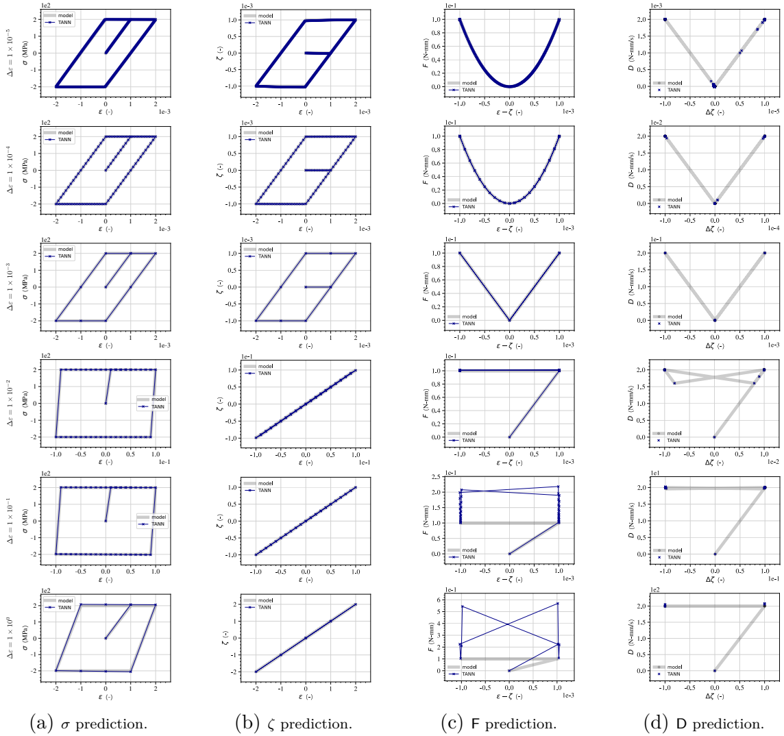
Figure 6.11 – Sensitivity on the inputs for material case 1D-A, with strain increments \Delta\varepsilon = \Delta\varepsilon \operatorname{sgn}\left(\cos\frac{n\pi}{2N}\right) –with N = \varepsilon_{\max}/\Delta\varepsilon , \varepsilon_{\max} = 2 \times 10^{-3} \div 2 , and \Delta\varepsilon varying from \times 10^{-5} (top) to 1 (bottom). Each column displays the response (from left to right) in term of \Delta\sigma (a), \Delta\zeta (b), F^{t+\Delta t} (c), and D^{t+\Delta t} (d). Each row represents the prediction at different \Delta\varepsilon .
