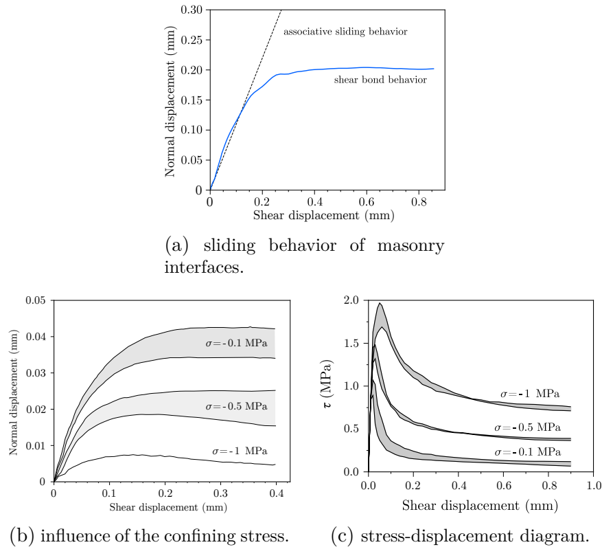
Figure 2.4 – Associative sliding behavior versus typical shear bond behavior of the joints (a) (Van der Pluijm, 1999), inelastic displacement normal to the joint upon inelastic shear of masonry (b) (Van der Pluijm, 1992), and stress-displacement diagram (c) for different normal stress levels (shaded areas indicate the envelope of multiple tests) (Van der Pluijm, 1999). Negative stress represents compression.
