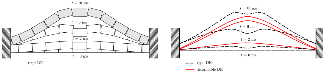
Figure C.4 – Representative scheme of the rotational locking displayed by infinitely rigid blocks (left) and comparison of the resulting deformed shaped with a deformable blocks model (right), for the non-associative case.
