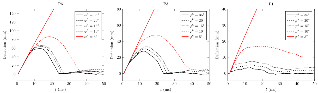
Figure 4.24 – Influence of the head joints angle of friction, \varphi^h , on the dynamic response of a barrel vault subjected to 10 kg of TNT in terms of the deflection of different points (P6, P3, and P1 cf. Fig. 4.18). The results refer to \varphi^b = 35^\circ , \psi^b = \psi^h = 0^\circ , and f_t = c = 0 MPa.
