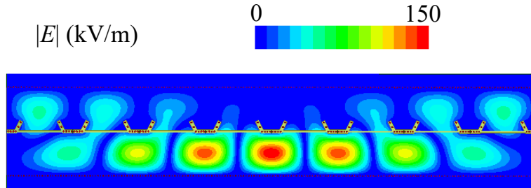
Fig. 3.28 The E -field distribution of 8-cell truncated SIWs of “air-filled cell 1”.
