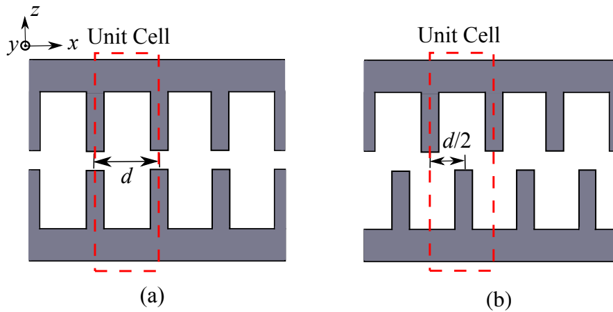
Fig. 4.2 Geometry comparison between normal periodic structures and glide-symmetric periodic structures [16], where d is the period length. (a) Normal periodic structures. (b) Glide-symmetric periodic structures.
