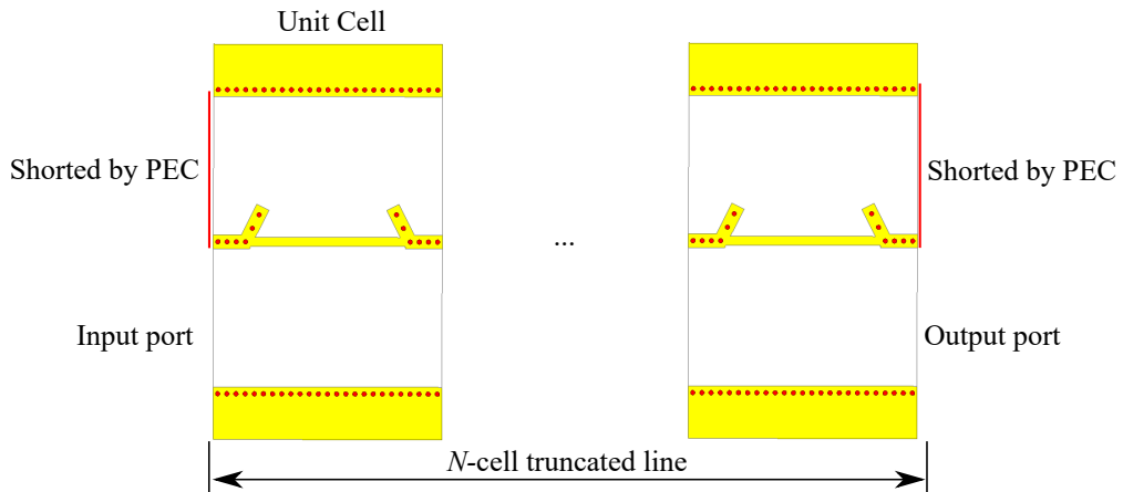
Fig. 3.25 The N -cell truncated simulation model of “air-filled cell 1”.
