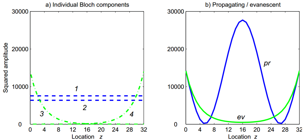
Fig. 1.7 Bloch components of DBE resonances [2]. The evanescent modes are essential for the enhancement of field amplitudes. (a) Four individual Bloch modes: forward and backward propagating modes, forward and backward evanescent modes. (b) Overall propagating and evanescent modes.
