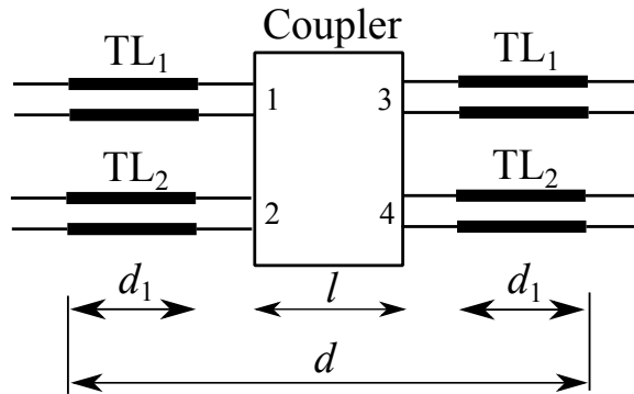
Fig. 2.3 Schematic of unit cell with one coupler.
