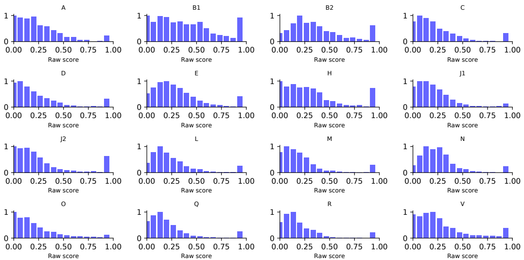
(b) Raw score distribution obtained with classifier-EXT .
